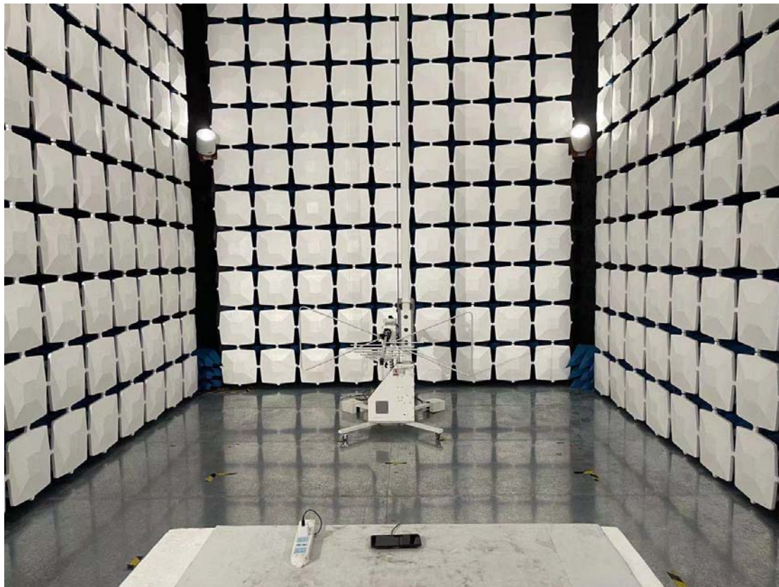
30MHZ-1GHz for radiated emission test setup
