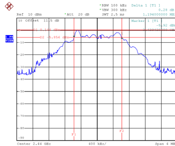
CH38 6 dB Bandwidth
