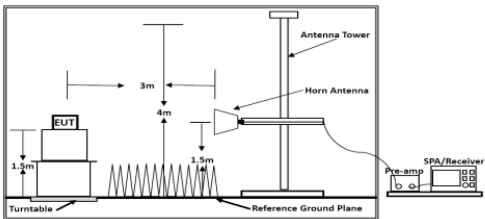
Above 1GHz
