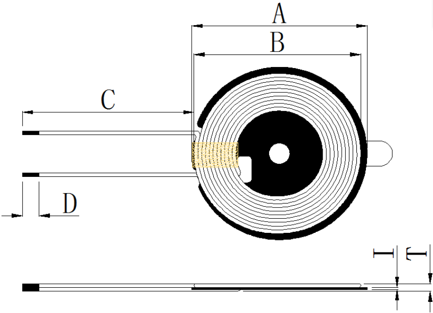
一、Outline dimensional drawing:(mm)
