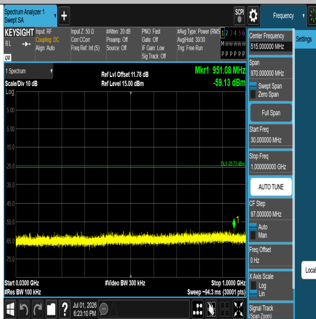
11B-Ant1-2462-30~1000-PASS
