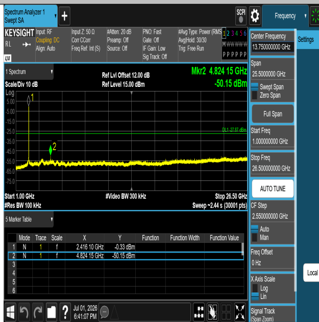
11G-Ant1-2412-1000~26500-PASS
