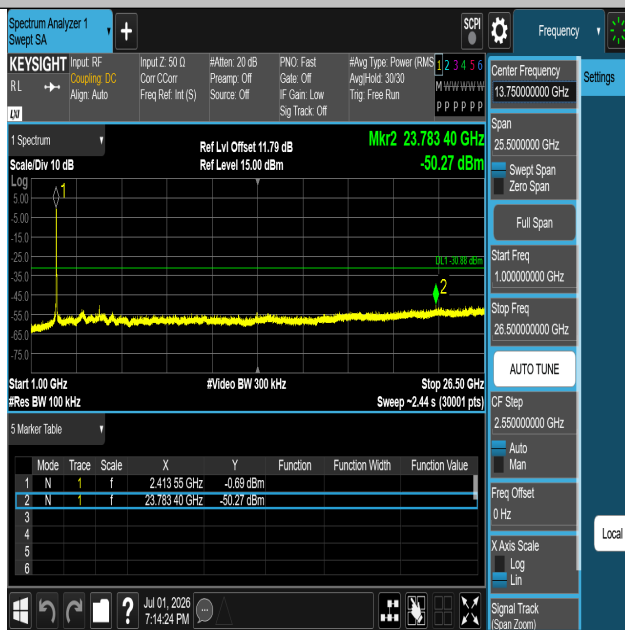
11N40SISO-Ant1-2422-1000~26500-PASS
