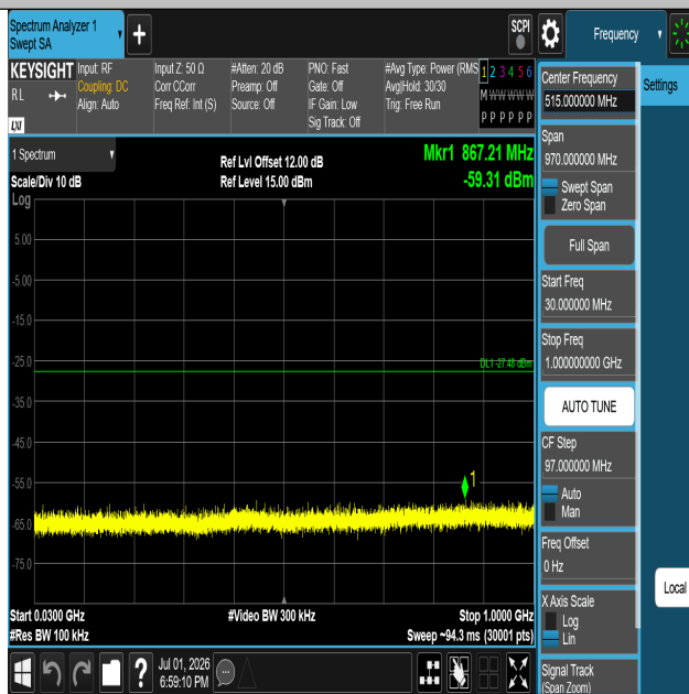
11N20SISO-Ant1-2412-30~1000-PASS
