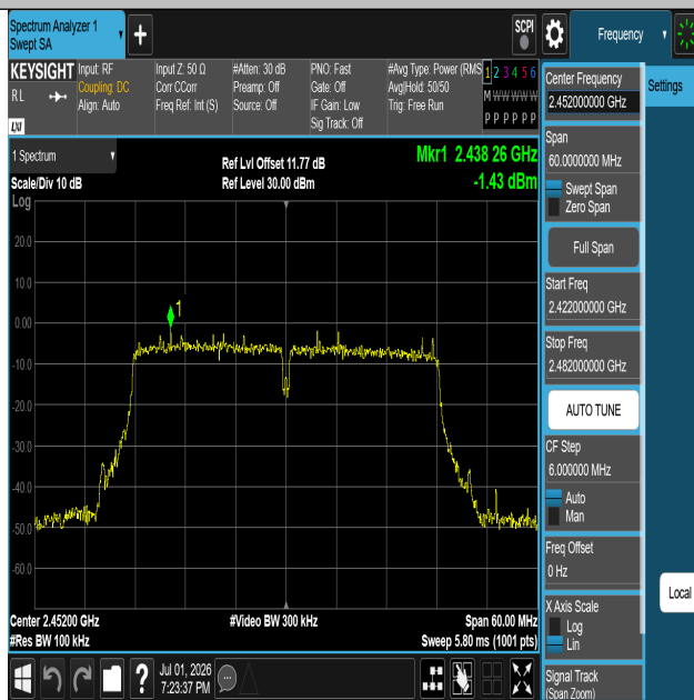
11N40SISO-Ant1-2452-0~Reference-PASS
