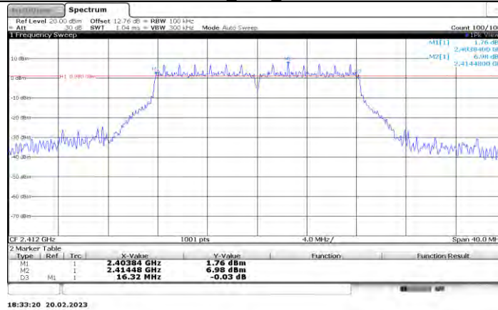
11G_Ant6_2412
