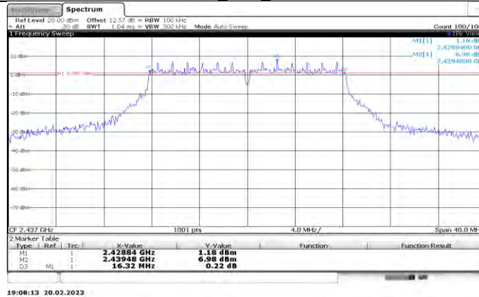
11G_Ant5_2437
