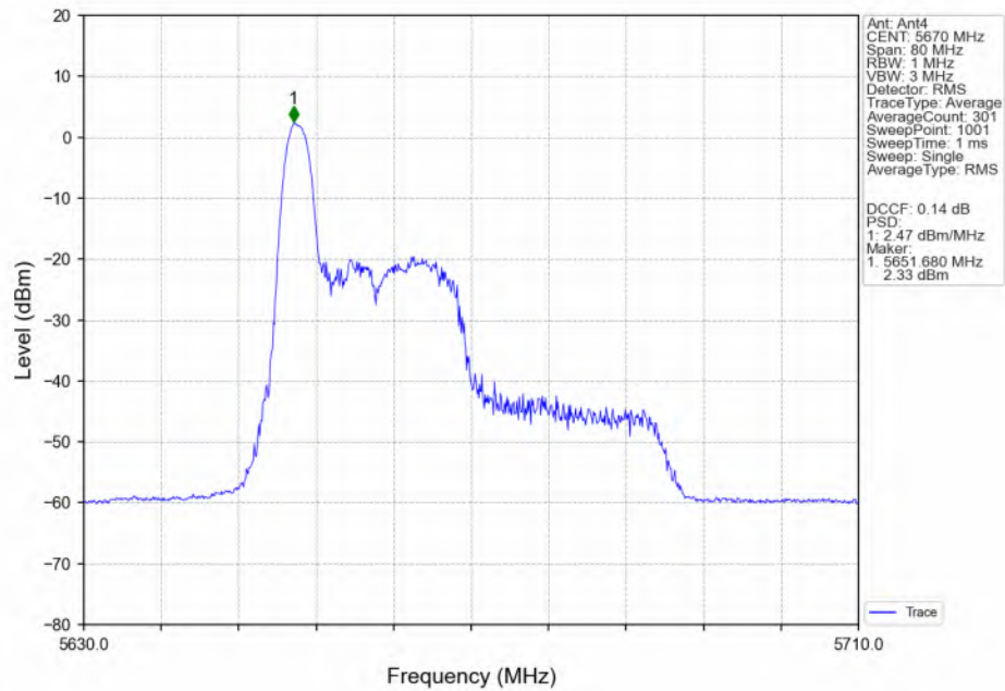
802.11ax(HEW40) HCH_5670MHz_RU26_Left(0)_MIMO_NTNV
