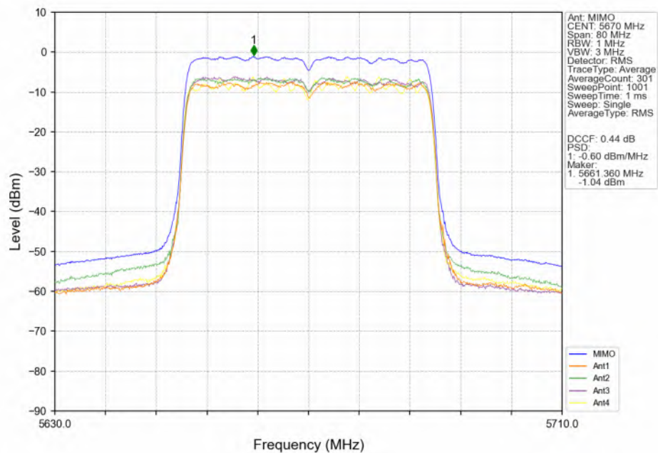
802.11ax(HEW40)_HCH_5670MHz_RU484_Left(65)_MIMO_NTNV
