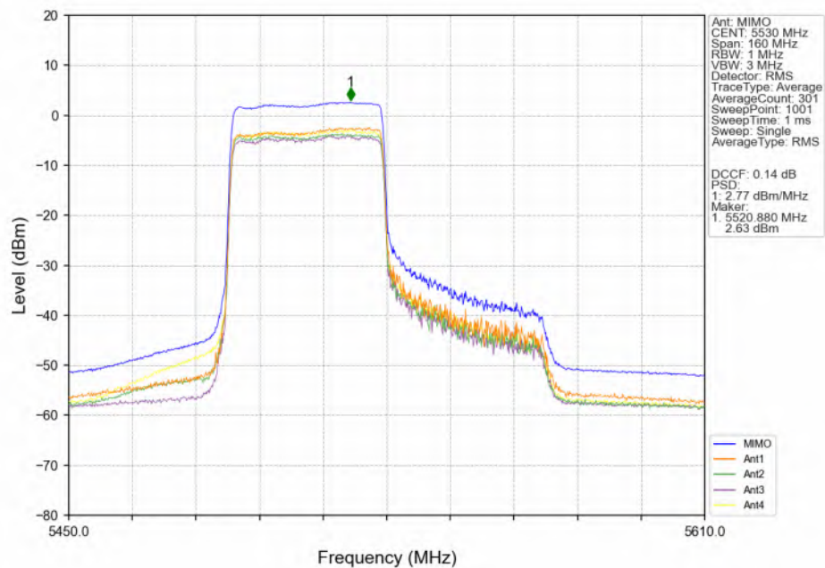
802.11ax(HEW80)_LCH_5530MHz_RU484_Left(65)_MIMO_NTNV
