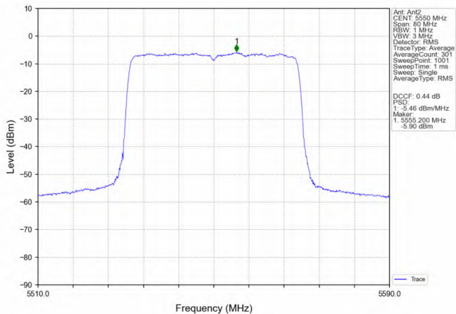
802.11ax(HEW40) MCH_5550MHz RU484 Left(65) Ant2 NTN
