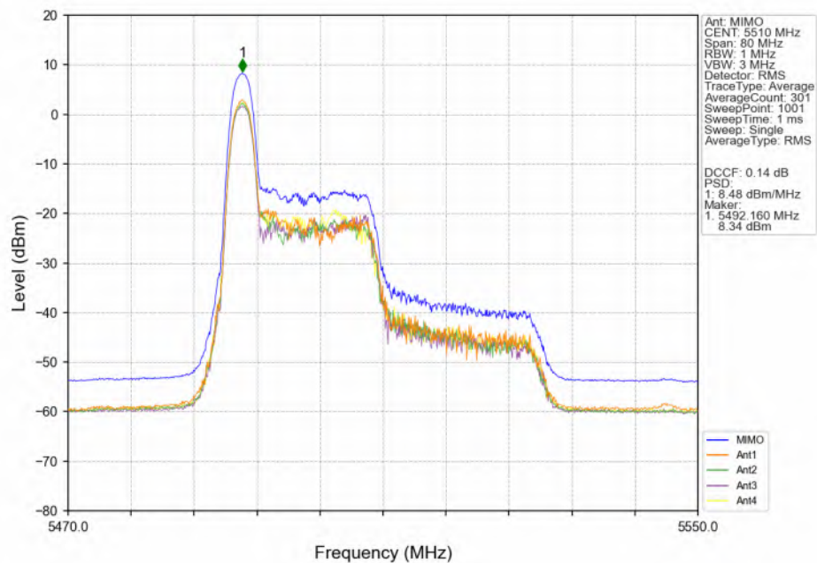
802.11ax(HEW40)_LCH_5510MHz_RU26_Left(0)_MIMO_NTNV
