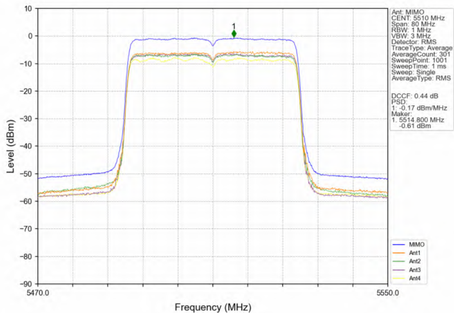
802.11ax(HEW40)_LCH_5510MHz_RU484_Left(65)_MIMO_NTNV
