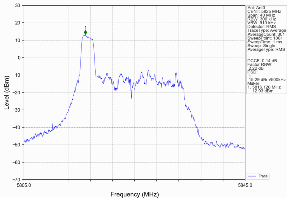
802.11ax(HEW20) HCH_5825MHz_RU26 Left(0)_Ant3_NTNV
