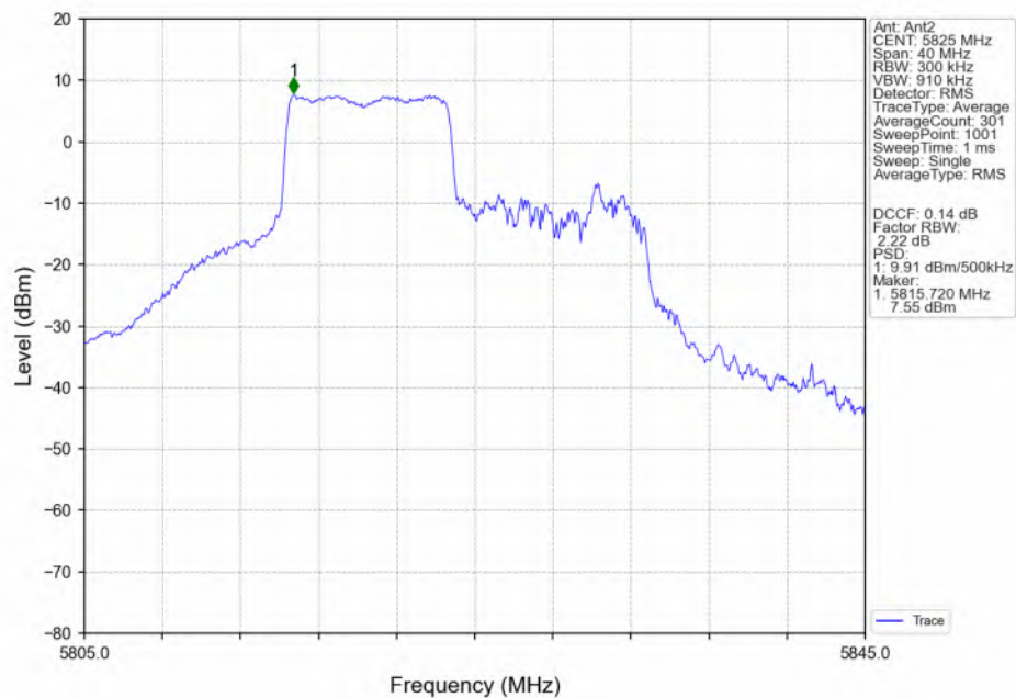
802.11ax(HEW20)_HCH_5825MHz_RU106_Left(53)_Ant2_NTNV
