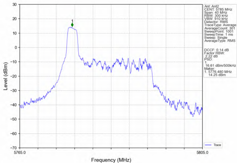
802.11ax(HEW20)_MCH_5785MHz_RU26_Left(0)_Ant2_NTNV
