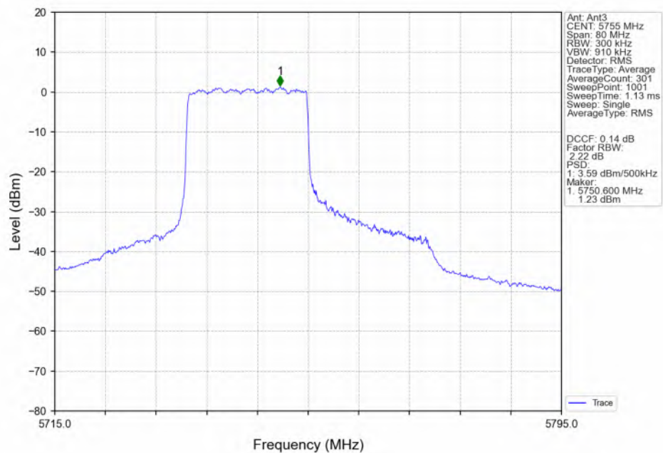
802.11ax(HEW40)_LCH_5755MHz_RU242_Left(61)_Ant3_NTNV
