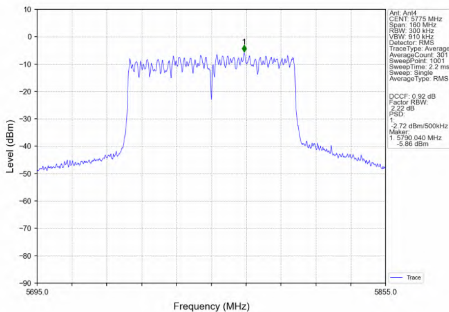
802.11ac(VHT80)_MCH_5775MHz_Ant4_NTNV
