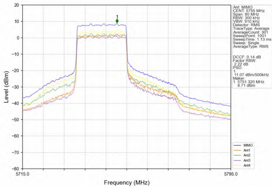
802.11ax(HEW40)_LCH_5755MHz_RU242_Left(61)_MIMO_NTNV
