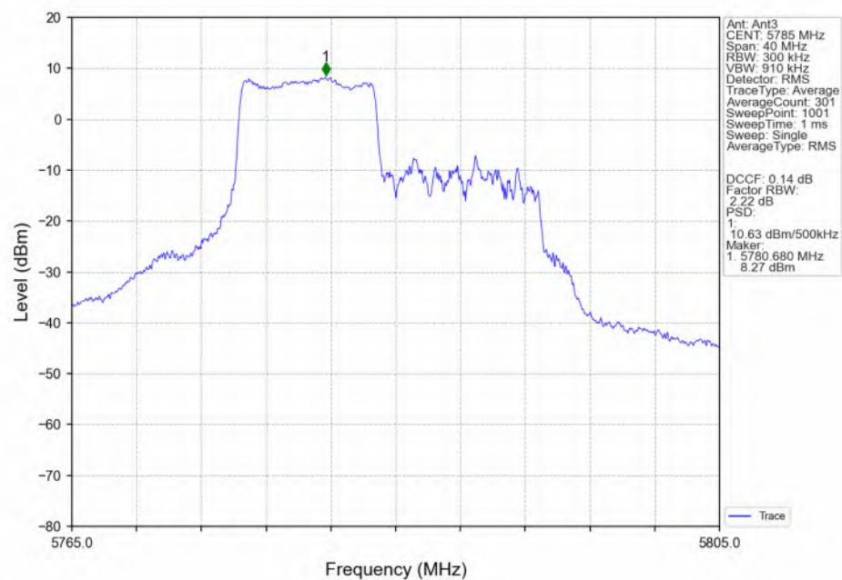
802.11ax(HEW20) MCH_5785MHz_RU106_Left(53)_Ant3_NTNV
