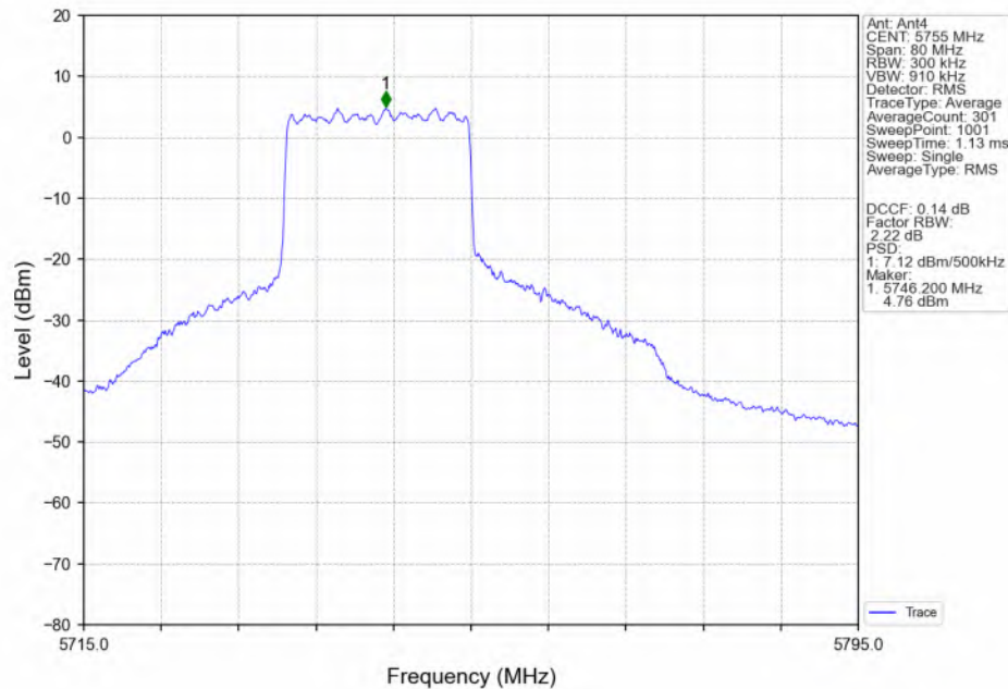
802.11ax(HEW40)_LCH_5755MHz_RU242_Left(61)_MIMO_NTNV
