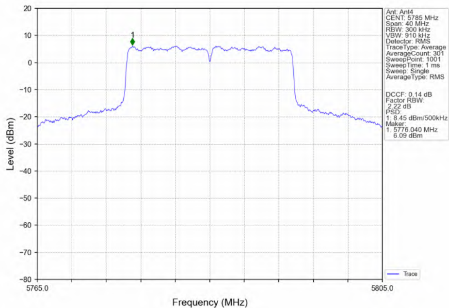
802.11ax(HEW20) MCH_5785MHz_RU242_Left(61)_Ant4_NTNV
