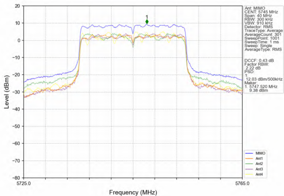
802.11ax(HEW20)_LCH_5745MHz_RU242_Left(61)_MIMO_NTNV
