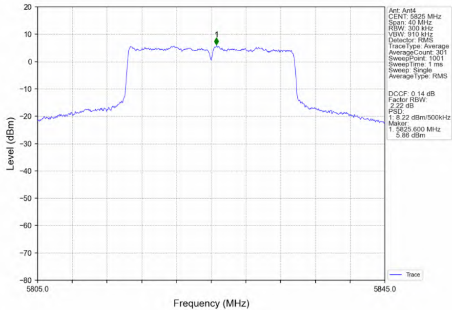
802.11ax(HEW20) HCH_5825MHz_RU242_Left(61)_MIMO_NTNV
