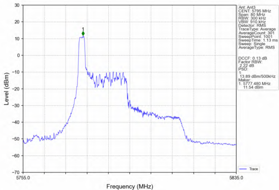
802.11ax(HEW40) HCH_5795MHz_RU26_Left(0)_Ant3_NTNV
