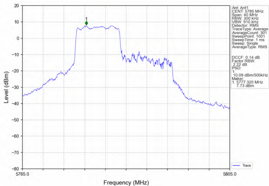
802.11ax(HEW20)_MCH_5785MHz_RU106_Left(53)_Ant1_NTNV
