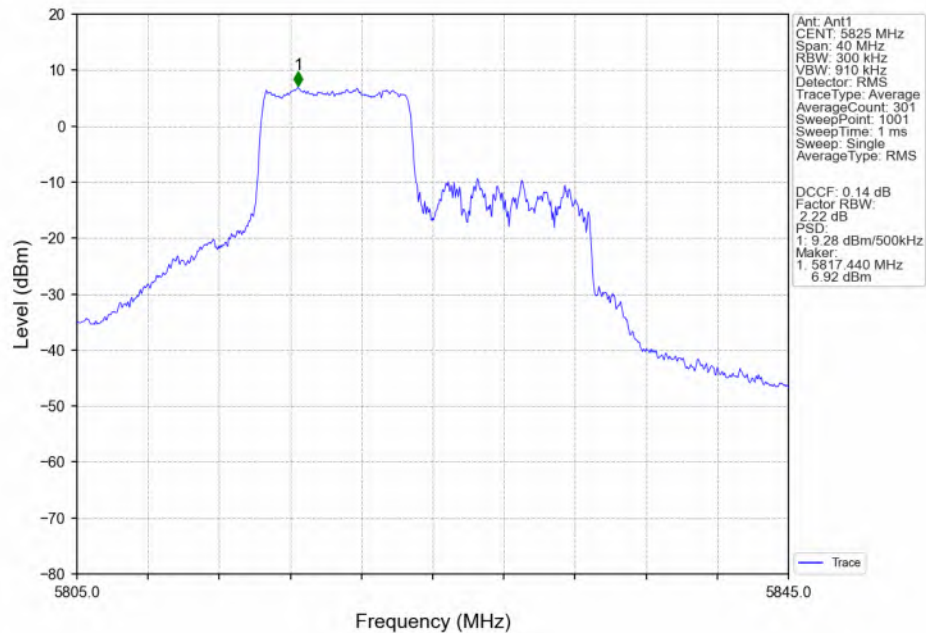
802.11ax(HEW20)_HCH_5825MHz_RU106_Left(53)_Ant2_NTNV
