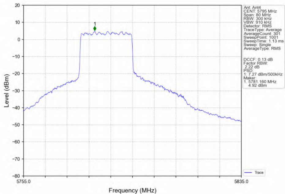
802.11ax(HEW40)_HCH_5795MHz_RU242_Left(61)_Ant4_NTNV
