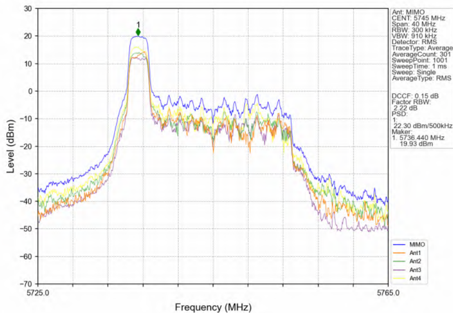
802.11ax(HEW20)_LCH_5745MHz_RU26_Left(0)_MIMO_NTNV
