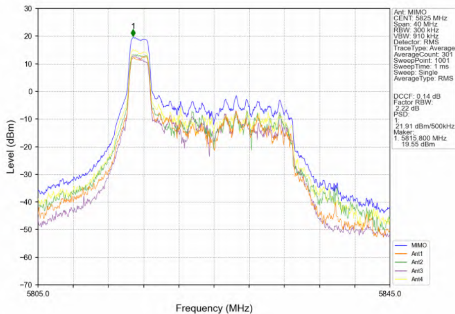
802.11ax(HEW20) HCH_5825MHz_RU26_Left(0)_MIMO_NTNV
