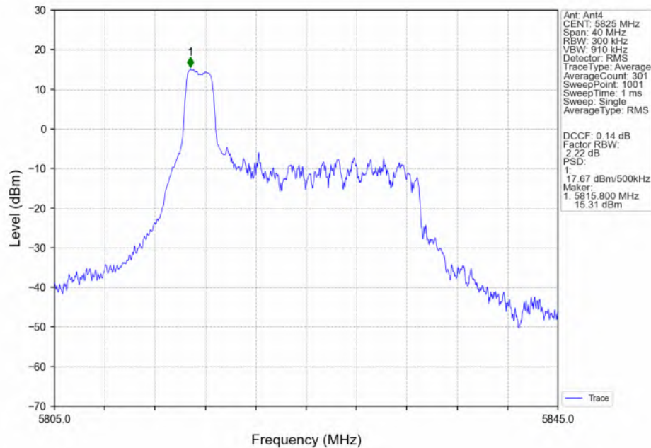
802.11ax(HEW20) HCH_5825MHz_RU26_Left(0)_MIMO_NTNV
