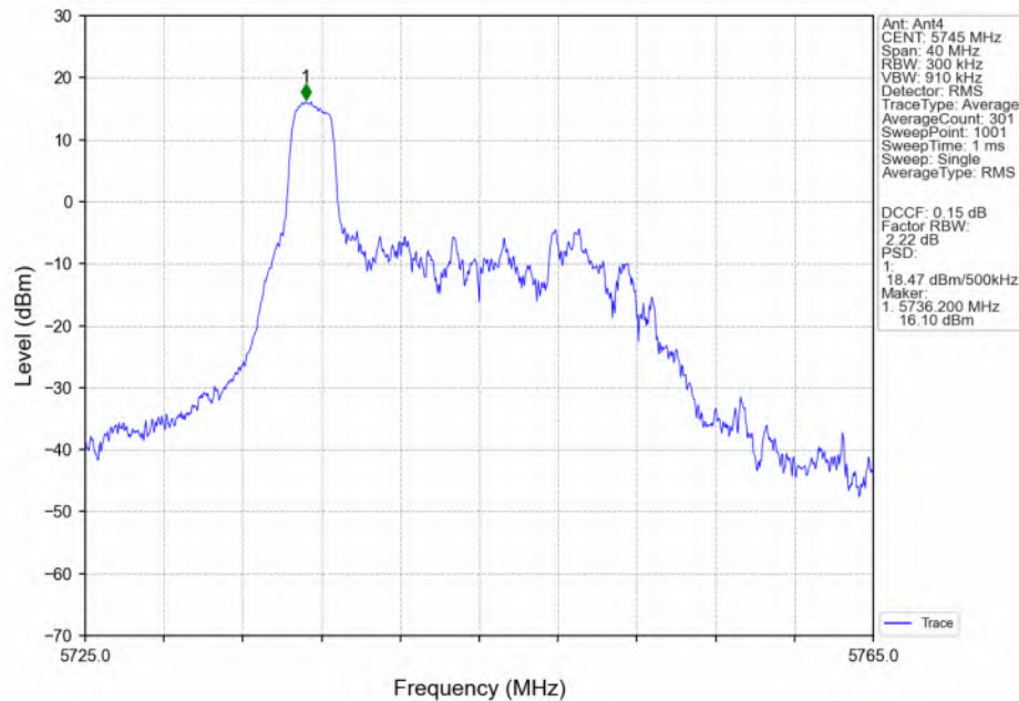
802.11ax(HEW20)_LCH_5745MHz_RU26_Left(0)_MIMO_NTNV
