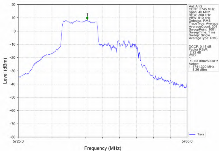
802.11ax(HEW20)_LCH_5745MHz_RU106_Left(53)_Ant2_NTNV
