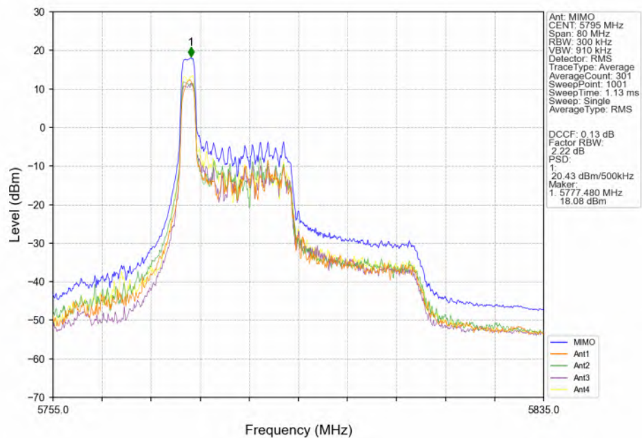
802.11ax(HEW40) HCH_5795MHz_RU26_Left(0)_MIMO_NTNV
