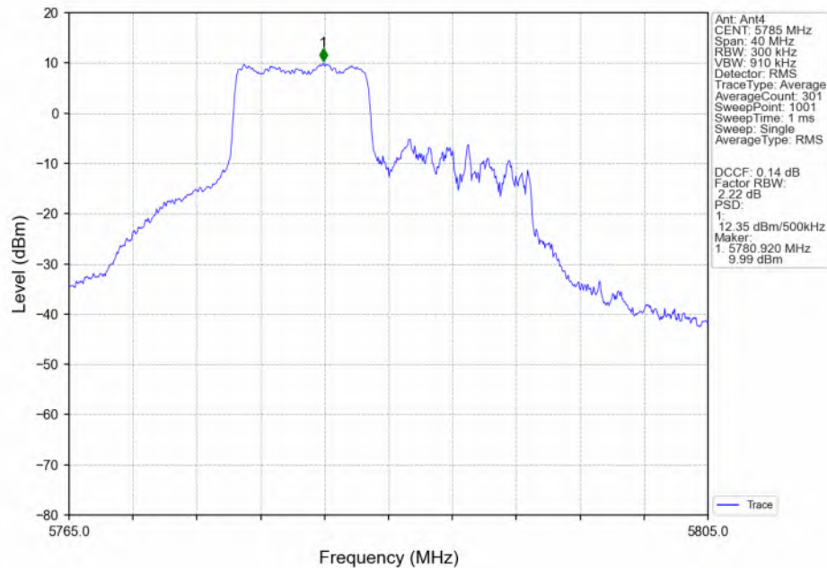
802.11ax(HEW20) MCH_5785MHz_RU106_Left(53)_MIMO_NTNV
