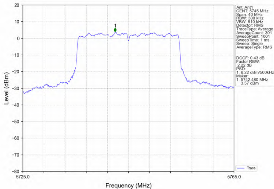
802.11ax(HEW20)_LCH_5745MHz_RU242_Left(61)_Ant1_NTNV
