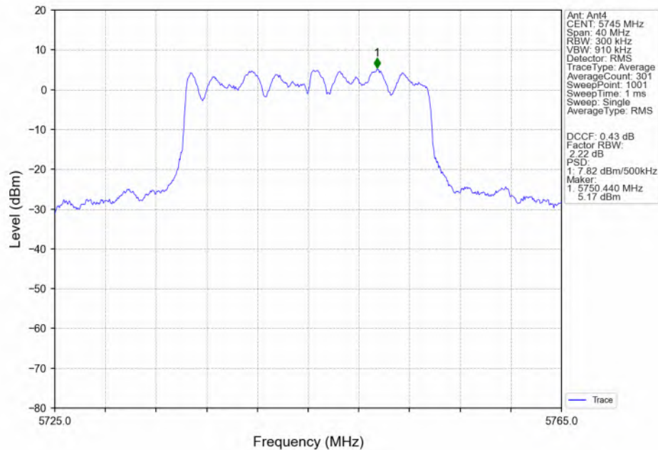
802.11ax(HEW20)_LCH_5745MHz_RU242_Left(61)_MIMO_NTNV
