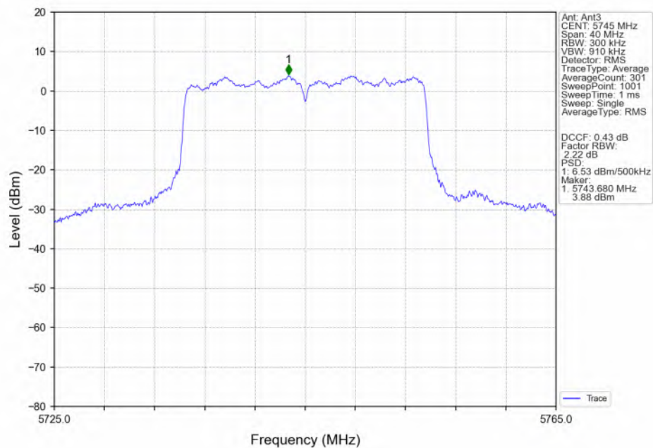
802.11ax(HEW20)_LCH_5745MHz_RU242_Left(61)_Ant3_NTNV
