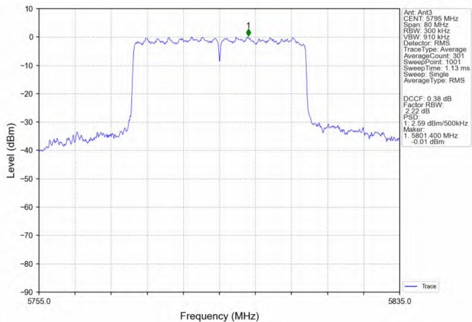
802.11ax(HEW40) HCH_5795MHz_RU484_Left(65)_Ant3_NTNV
