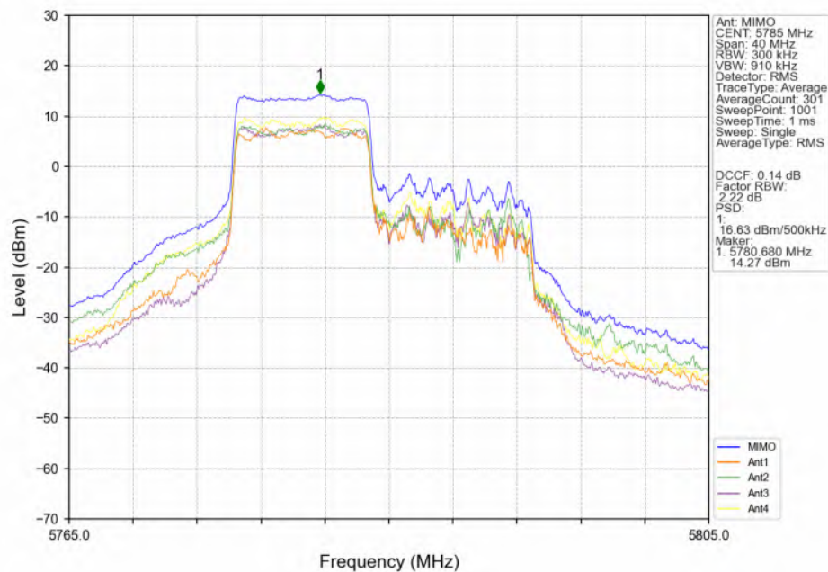
802.11ax(HEW20) MCH_5785MHz_RU106_Left(53)_MIMO_NTNV
