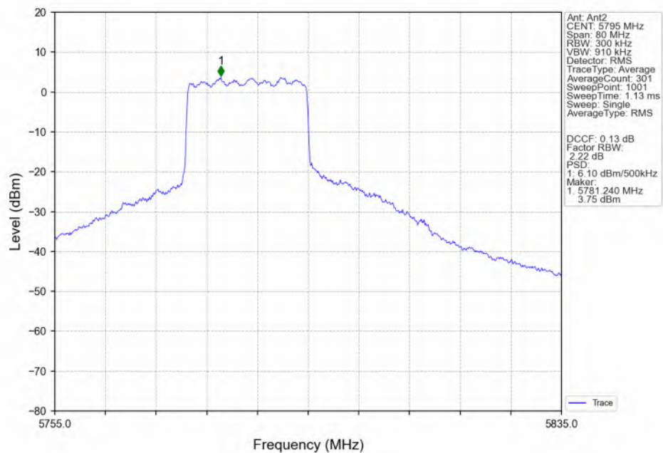
802.11ax(HEW40)_HCH_5795MHz_RU242_Left(61)_Ant2_NTNV
