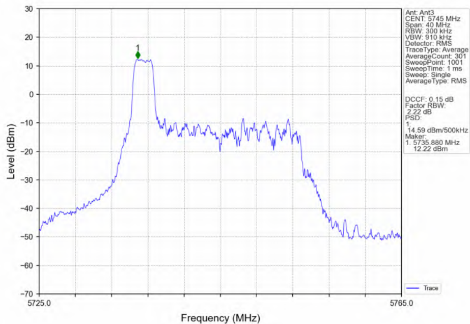
802.11ax(HEW20)_LCH_5745MHz_RU26_Left(0)_Ant3_NTNV
