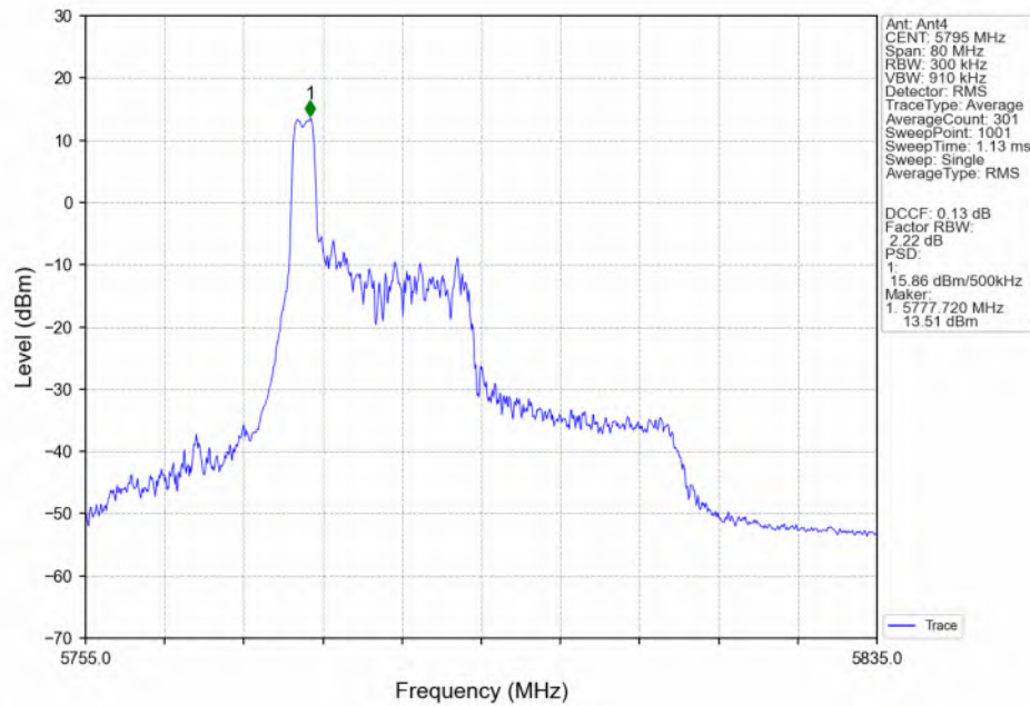
802.11ax(HEW40) HCH_5795MHz_RU26_Left(0)_MIMO_NTNV
