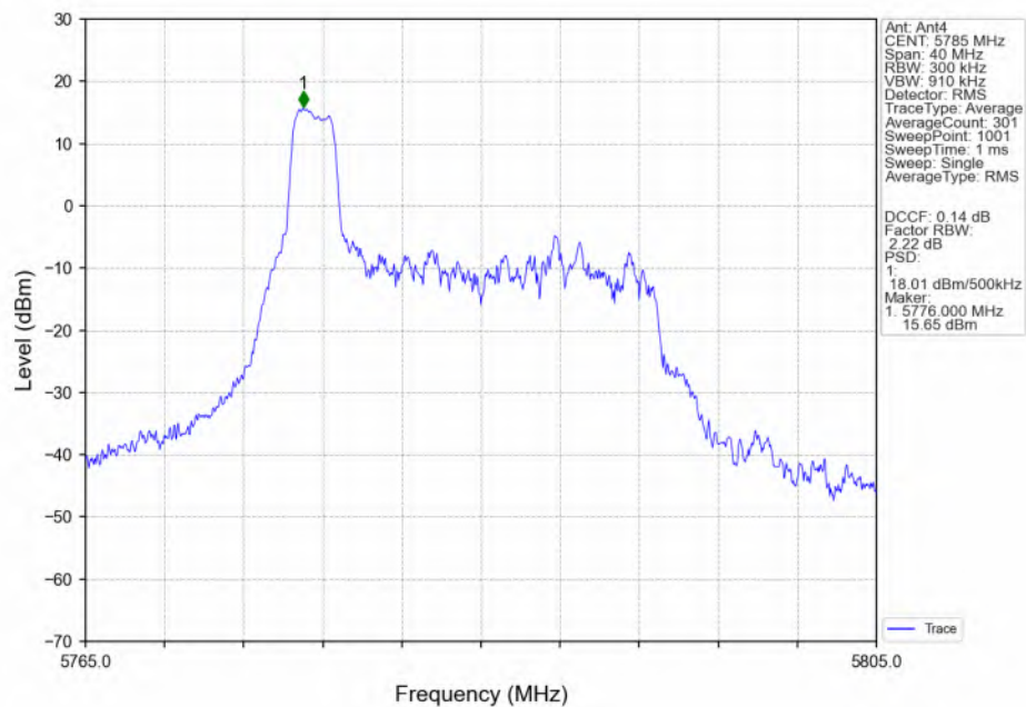
802.11ax(HEW20)_MCH_5785MHz_RU26_Left(0)_Ant4_NTNV
