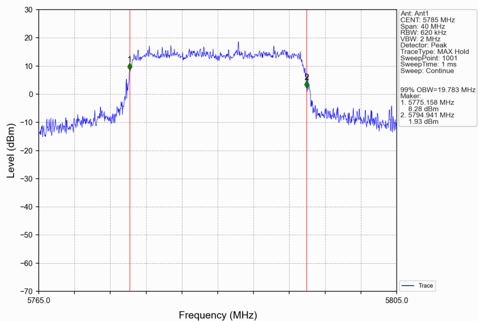
802.11ax(HEW20)_MCH_5785MHz_RU242_Left(61)_Ant1_NTNV
