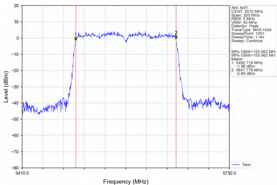
802.11ac(VHT160)_MCH_5570MHz_Ant1_NTNV
