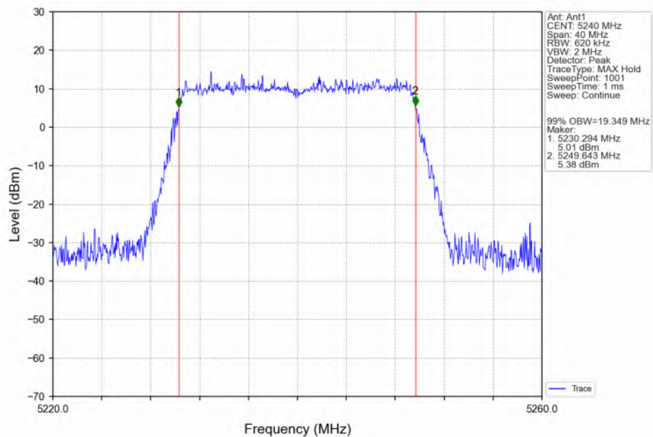
802.11ax(HEW20) HCH_5240MHz_RU242_Left(61)_Ant1_NTNV
