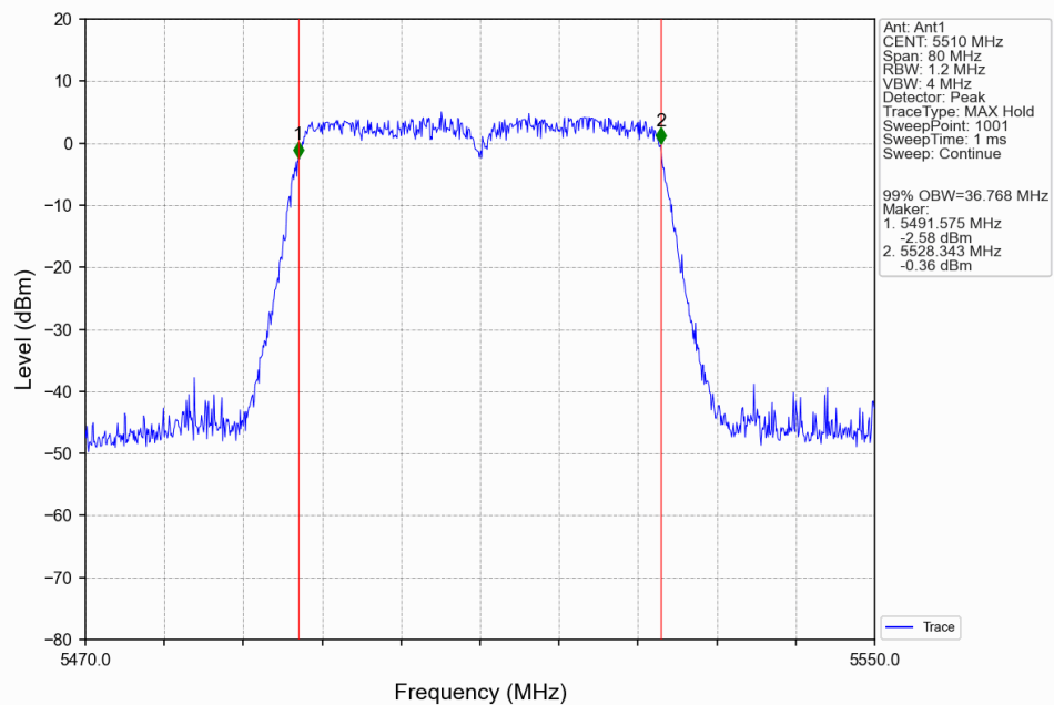
802.11ac(VHT40)_LCH_5510MHz_Ant1_NTNV
