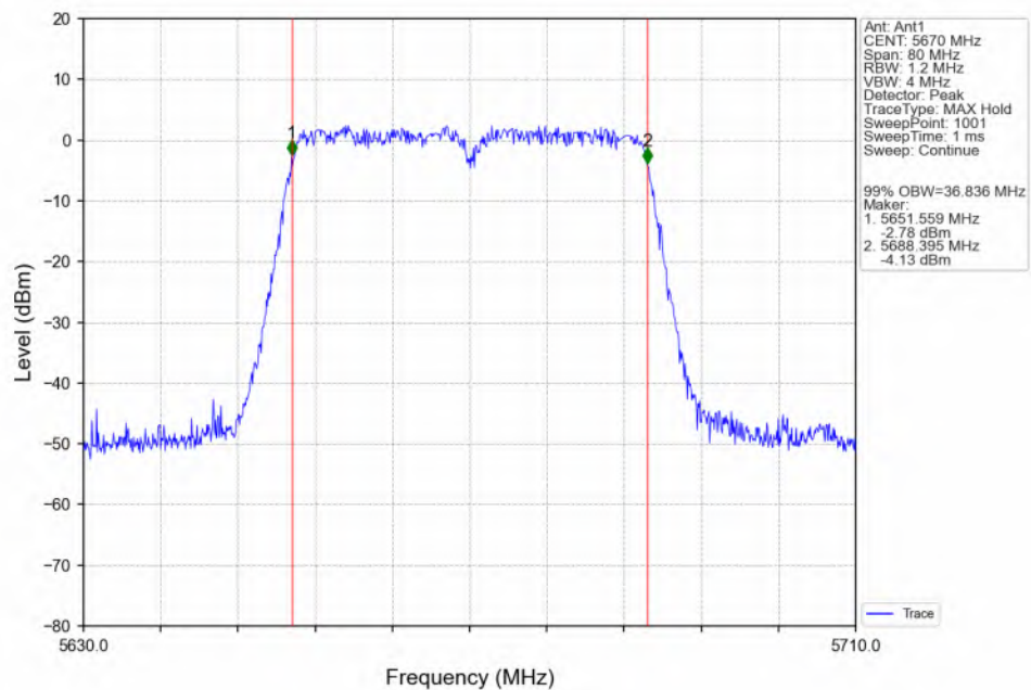
802.11ac(VHT40)_HCH_5670MHz_Ant1_NTNV
