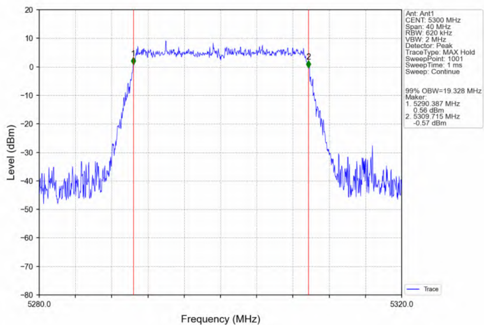
802.11ax(HEW20)_MCH_5300MHz_RU242_Left(61)_Ant1_NTNV
