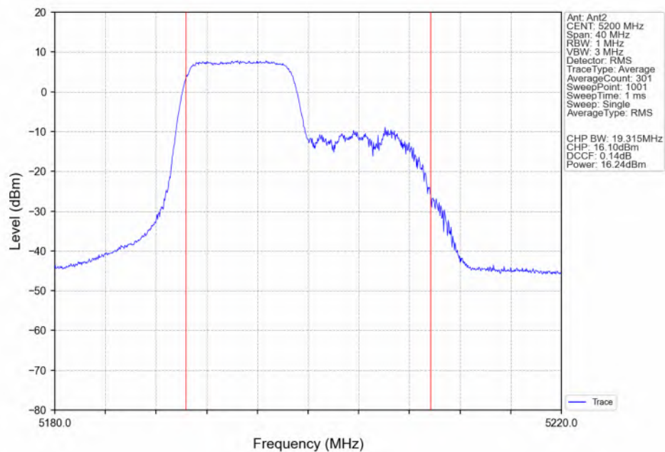
802.11ax(HEW20) MCH_5200MHz_RU106_Left(53)_Ant2_NTNV
