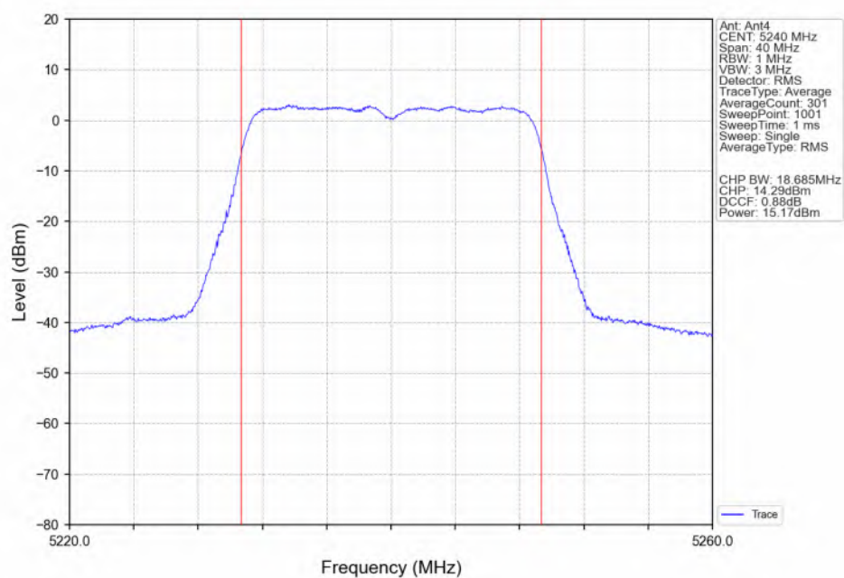
802.11ac(VHT20)_HCH_5240MHz_Ant4_NTNV
