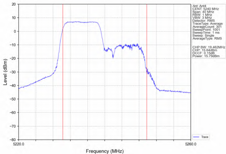
802.11ax(HEW20) HCH 5240MHz RU106 Left(53) Ant4 NTNv
