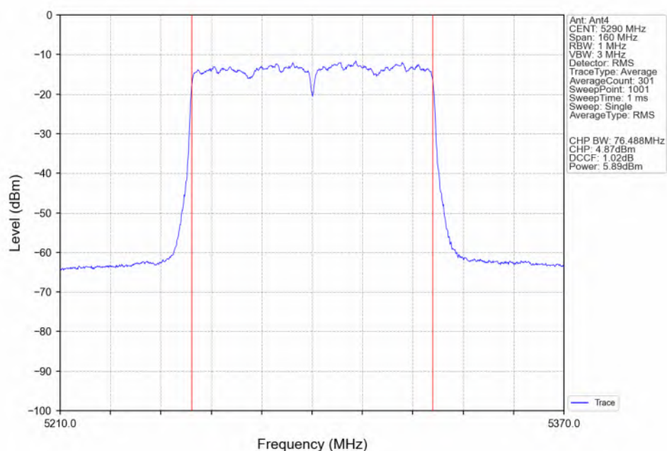
802.11ac(VHT80)_MCH_5290MHz_Ant4_NTNV
