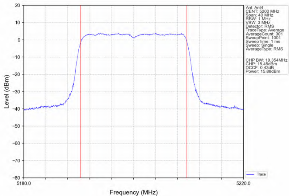
802.11ax(HEW20) MCH_5200MHz_RU242_Left(61)_Ant4_NTNV
