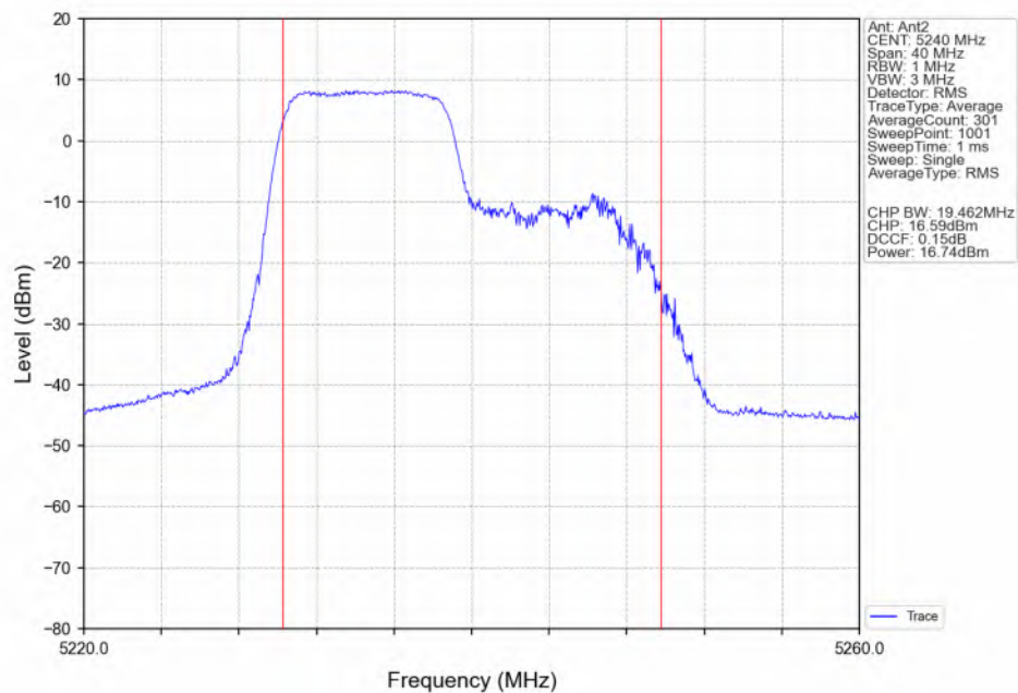
802.11ax(HEW20) HCH 5240MHz RU106 Left(53) Ant2 NTN
