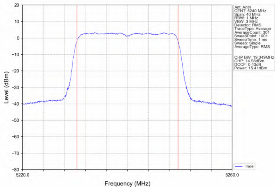
802.11ax(HEW20)_HCH_5240MHz_RU242_Left(61)_Ant4_NTNV
