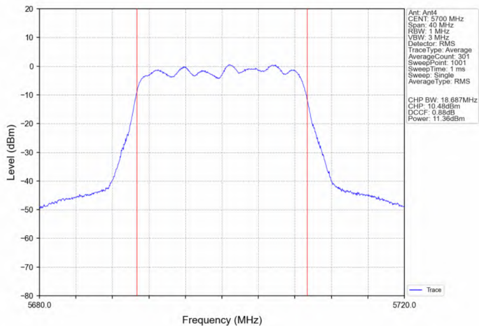
802.11ac(VHT20)_HCH_5700MHz_Ant4_NTNV
