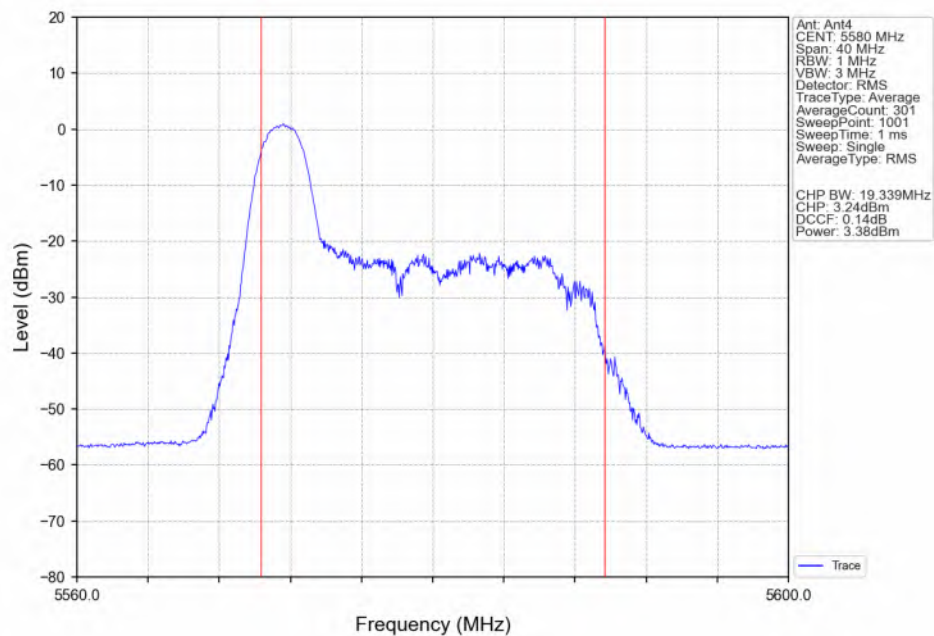
802.11ax(HEW20)_MCH_5580MHz_RU26_Left(0)_Ant4_NTNV
