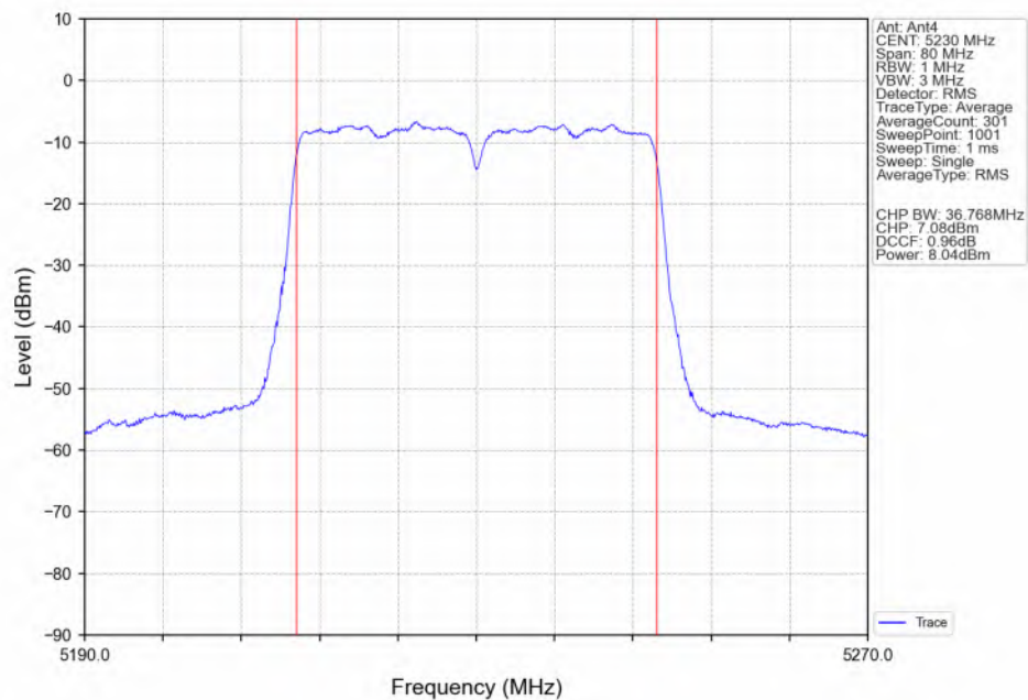
802.11ac(VHT40)_HCH_5230MHz_Ant4_NTNV
