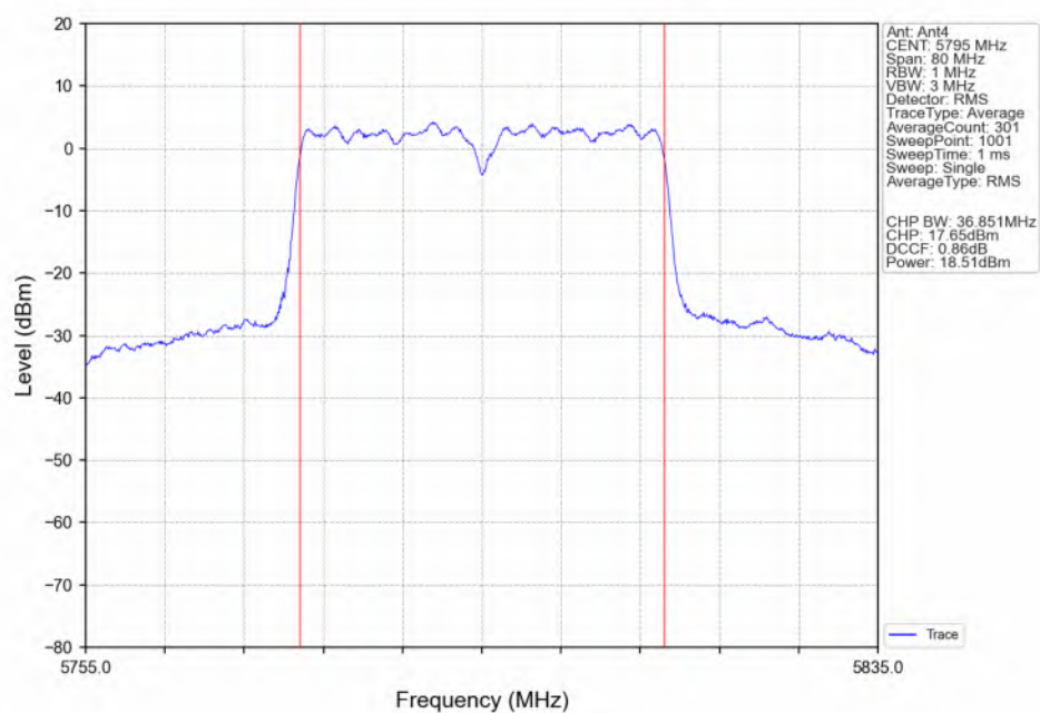
802.11ac(VHT40)_HCH_5795MHz_Ant4_NTNV
