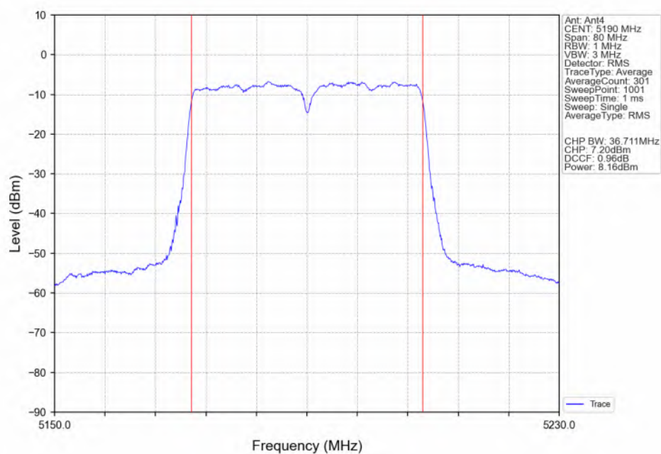
802.11ac(VHT40)_LCH_5190MHz_Ant4_NTNV
