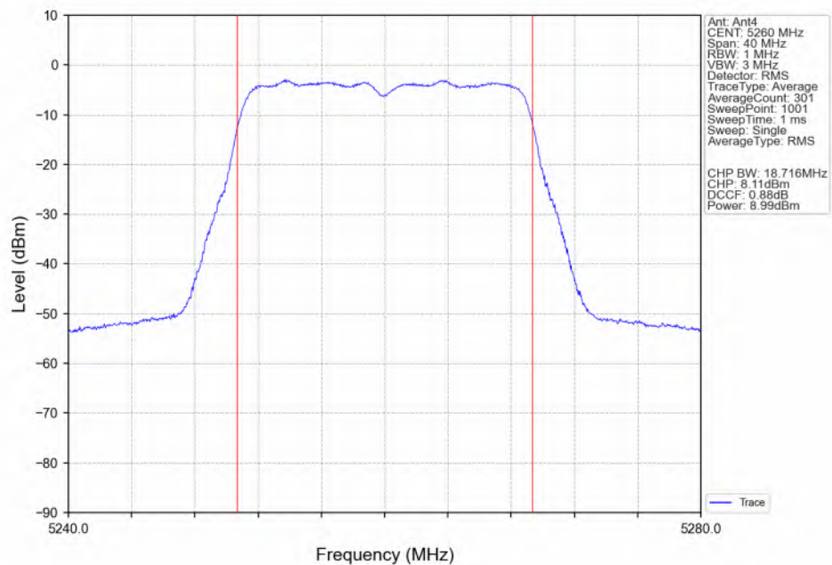
802.11ac(VHT20)_LCH_5260MHz_Ant4_NTNV
