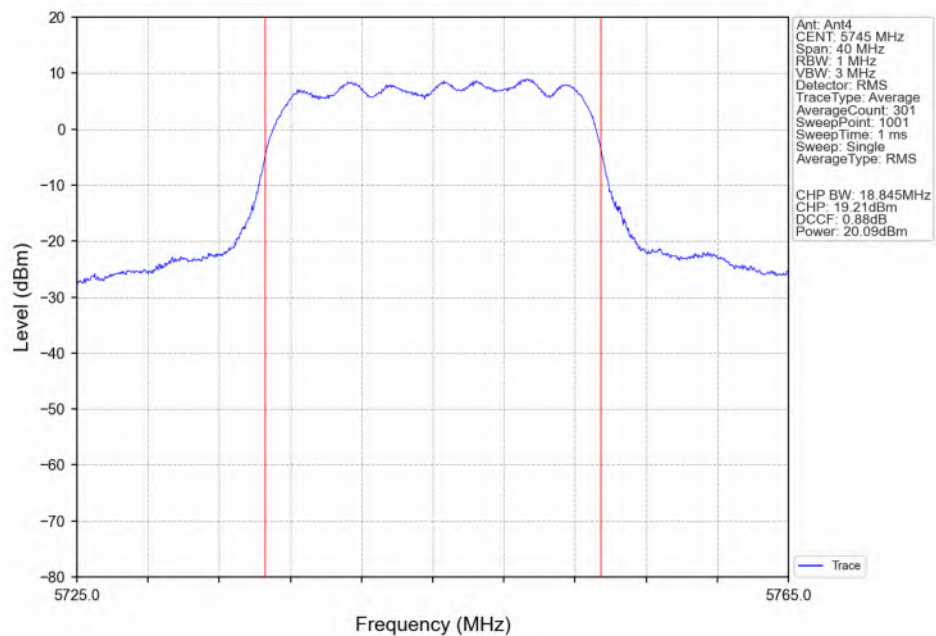
802.11ac(VHT20)_LCH_5745MHz_Ant4_NTNV
