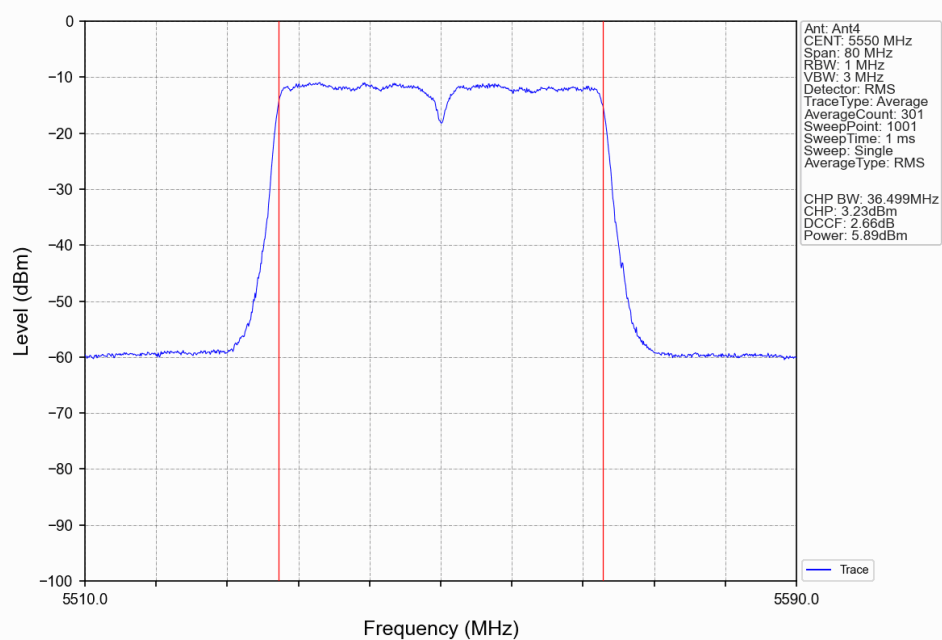
802.11n(HT40)_MCH_5550MHz_Ant4_NTNV
