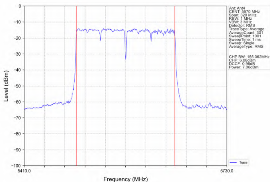
802.11ac(VHT160)_MCH_5570MHz_Ant4_NTNV
