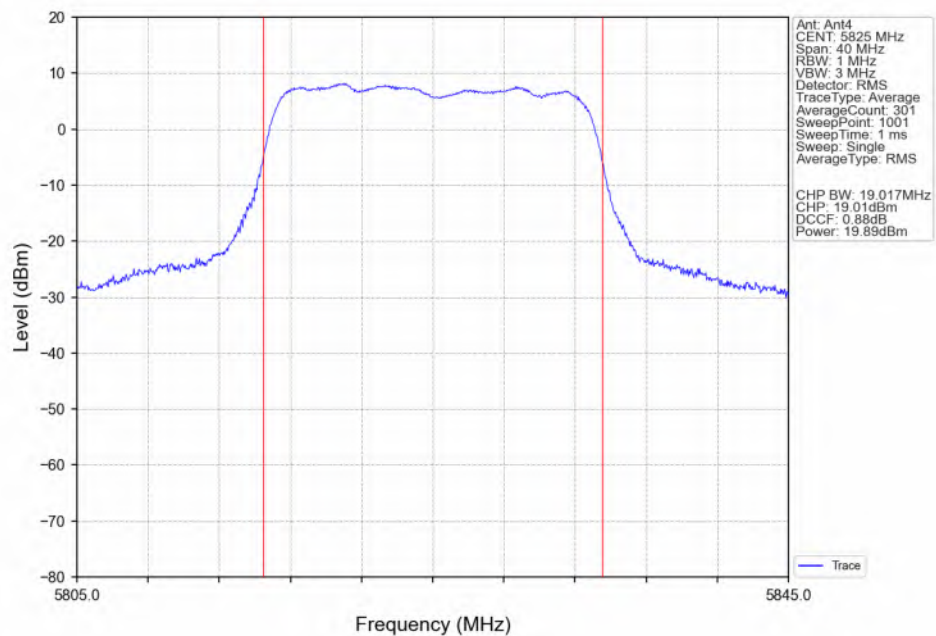
802.11ac(VHT20)_HCH_5825MHz_Ant4_NTNV
