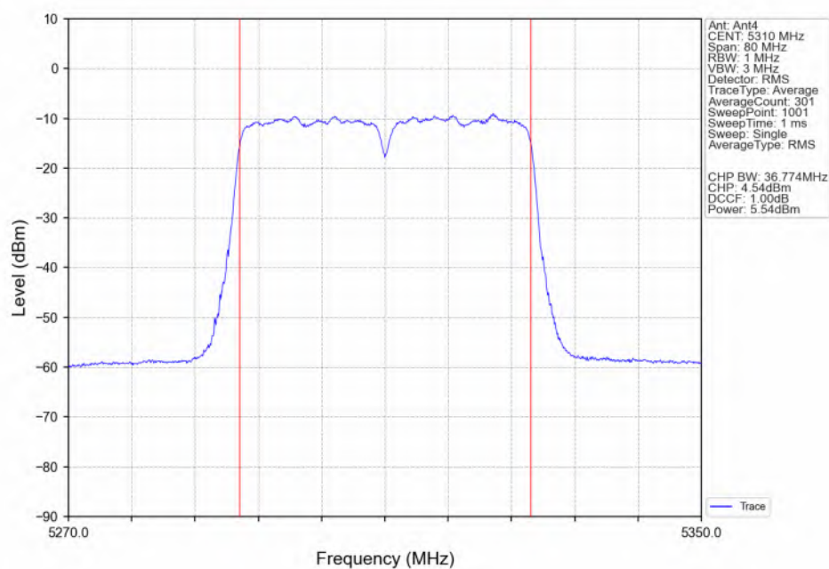
802.11ac(VHT40)_HCH_5310MHz_Ant4_NTNV
