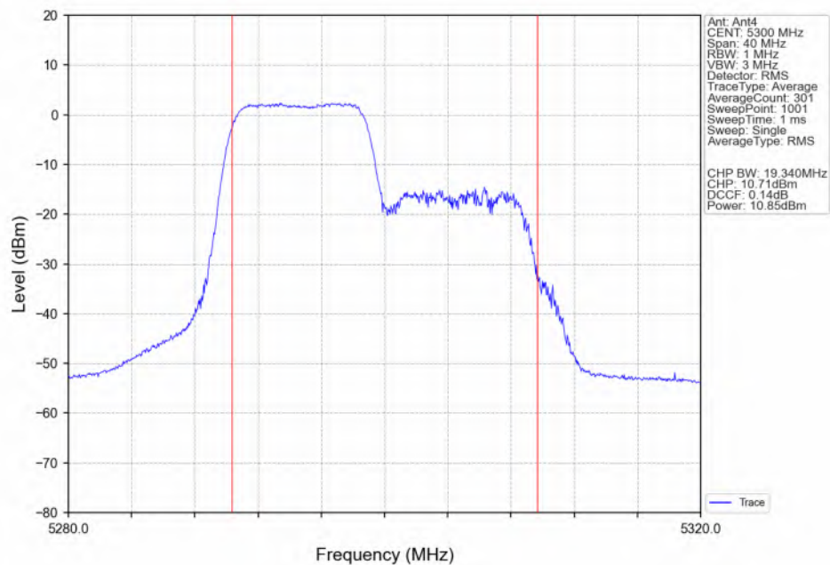
802.11ax(HEW20) MCH_5300MHz_RU106_Left(53)_Ant4_NTNV
