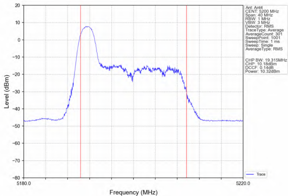
802.11ax(HEW20)_MCH_5200MHz_RU26_Left(0)_Ant4_NTNV
