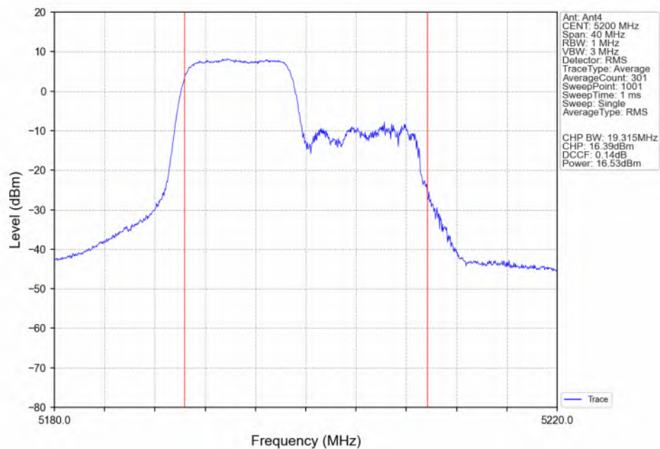
802.11ax(HEW20) MCH_5200MHz_RU106_Left(53)_Ant4_NTNV
