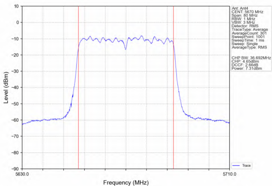
802.11n(HT40)_HCH_5670MHz_Ant4_NTNV
