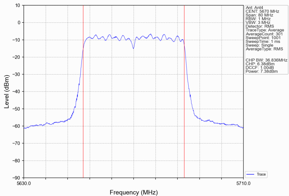
802.11ac(VHT40)_HCH_5670MHz_Ant4_NTNV
