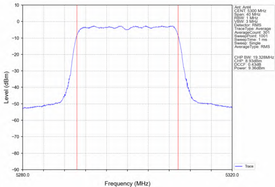
802.11ax(HEW20) MCH_5300MHz_RU242_Left(61)_Ant4_NTNV
