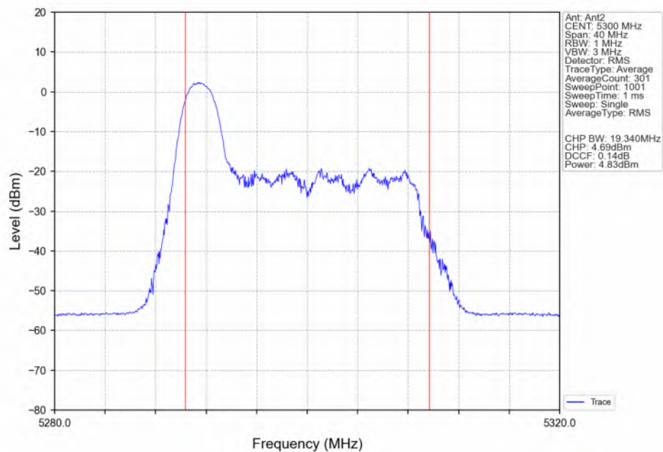
802.11ax(HEW20)_MCH_5300MHz_RU26_Left(0)_Ant2_NTNV
