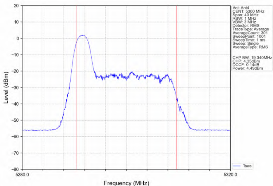
802.11ax(HEW20)_MCH_5300MHz_RU26_Left(0)_Ant4_NTNV
