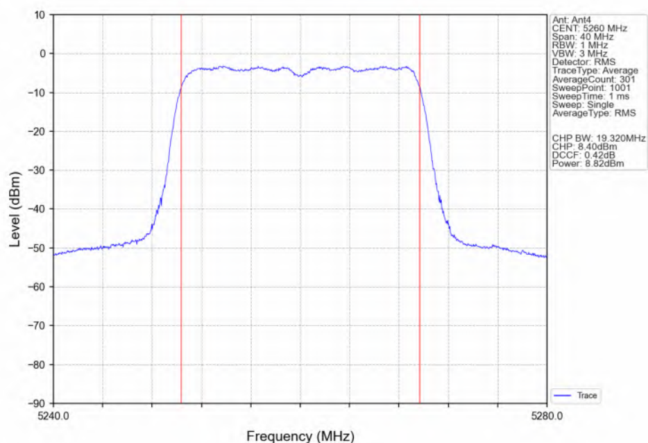
802.11ax(HEW20)_LCH_5260MHz_RU242_Left(61)_Ant4_NTNV
