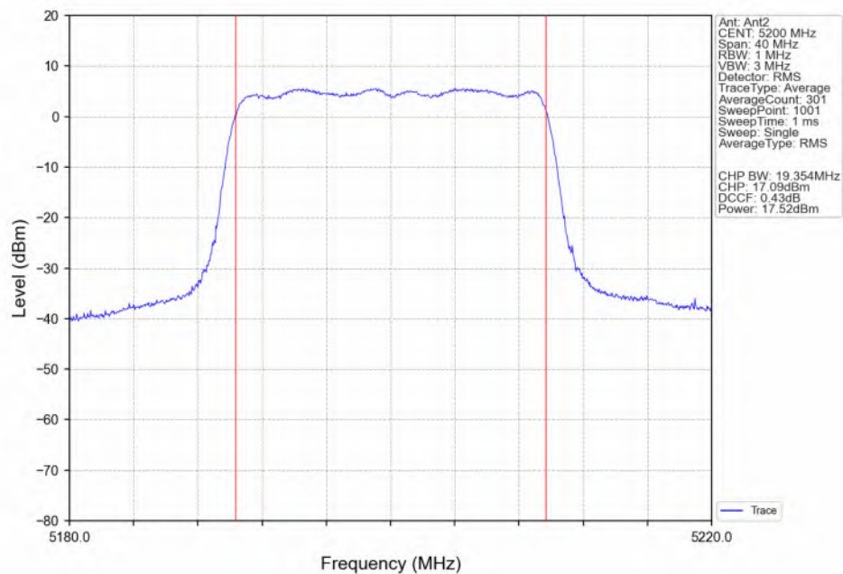
802.11ax(HEW20) MCH_5200MHz_RU242_Left(61)_Ant2_NTNV
