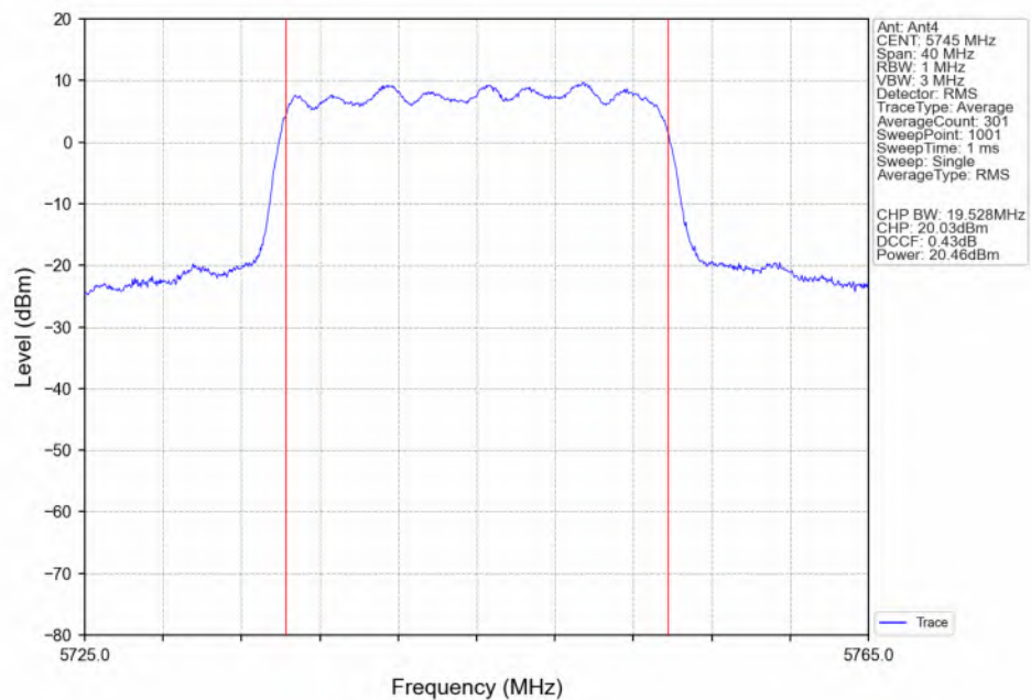
802.11ax(HEW20)_LCH_5745MHz_RU242_Left(61)_Ant4_NTNV
