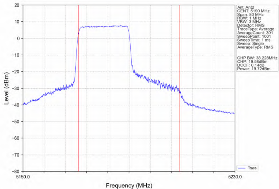
802.11ax(HEW40)_LCH_5190MHz_RU242_Left(61)_Ant2_NTNV
