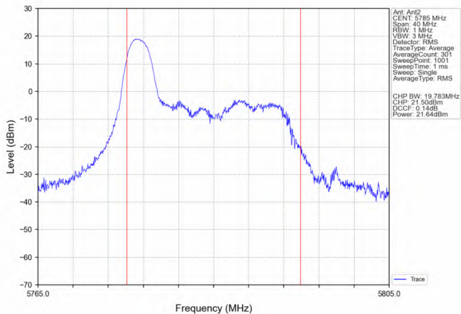
802.11ax(HEW20)_MCH_5785MHz_RU26_Left(0)_Ant2_NTNV
