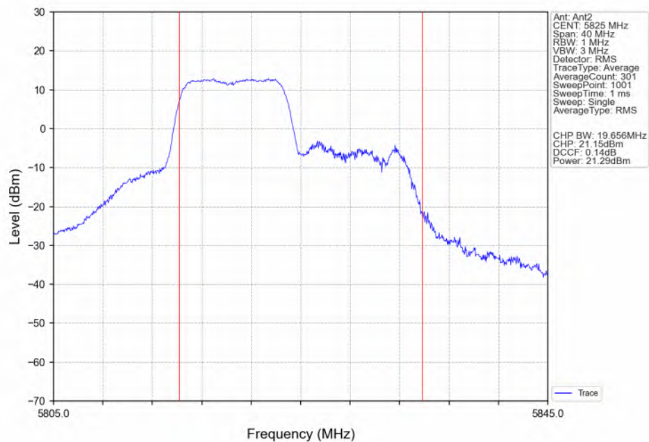
802.11ax(HEW20) HCH 5825MHz RU106 Left(53) Ant2 NTN
