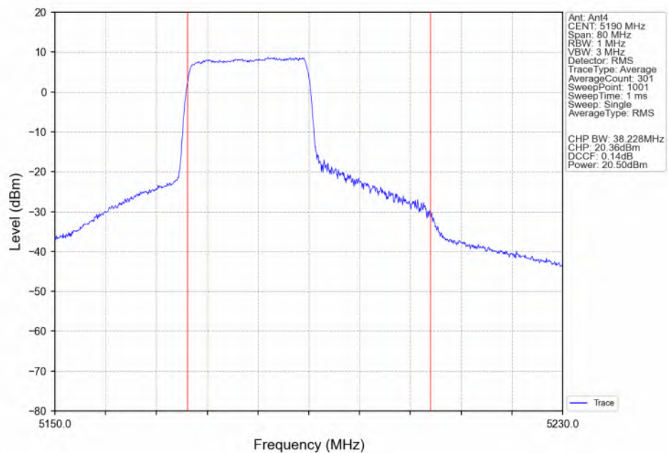
802.11ax(HEW40)_LCH_5190MHz_RU242_Left(61)_Ant4_NTNV
