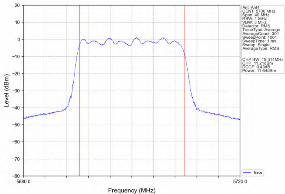
802.11ax(HEW20) HCH_5700MHz_RU242_Left(61)_Ant4_NTNV
