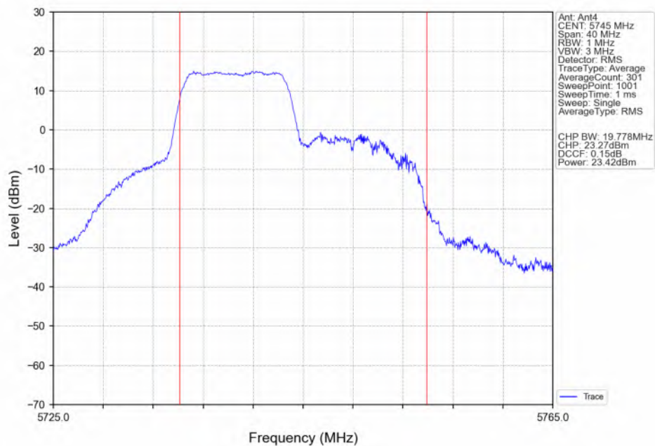
802.11ax(HEW20)_LCH_5745MHz_RU106_Left(53)_Ant4_NTNV
