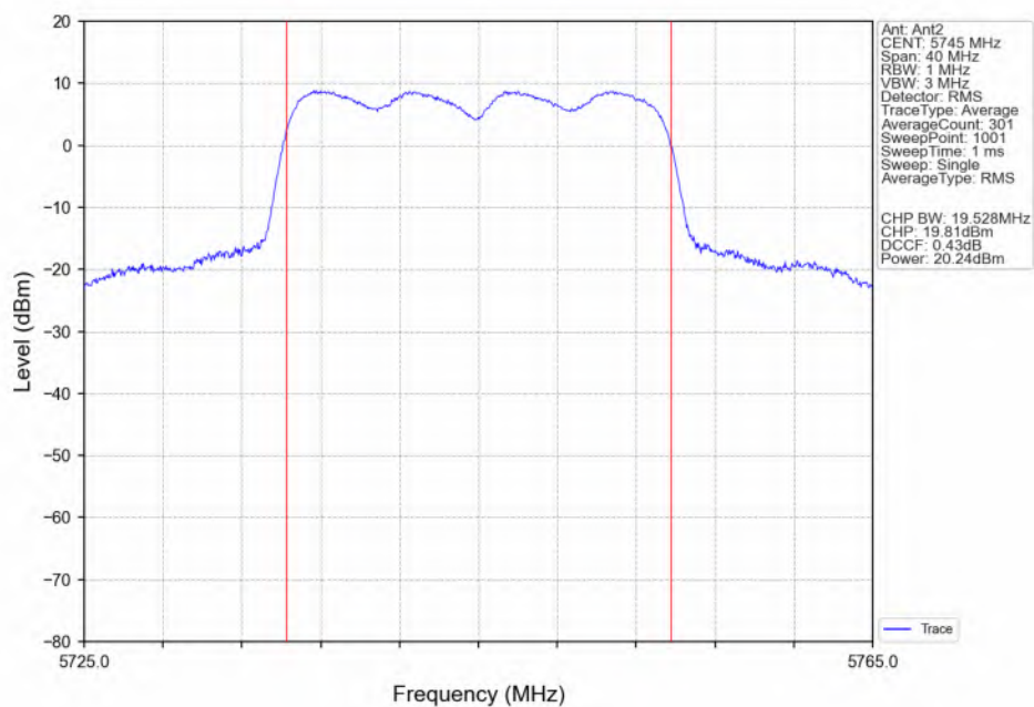
802.11ax(HEW20)_LCH_5745MHz_RU242_Left(61)_Ant2_NTNV
