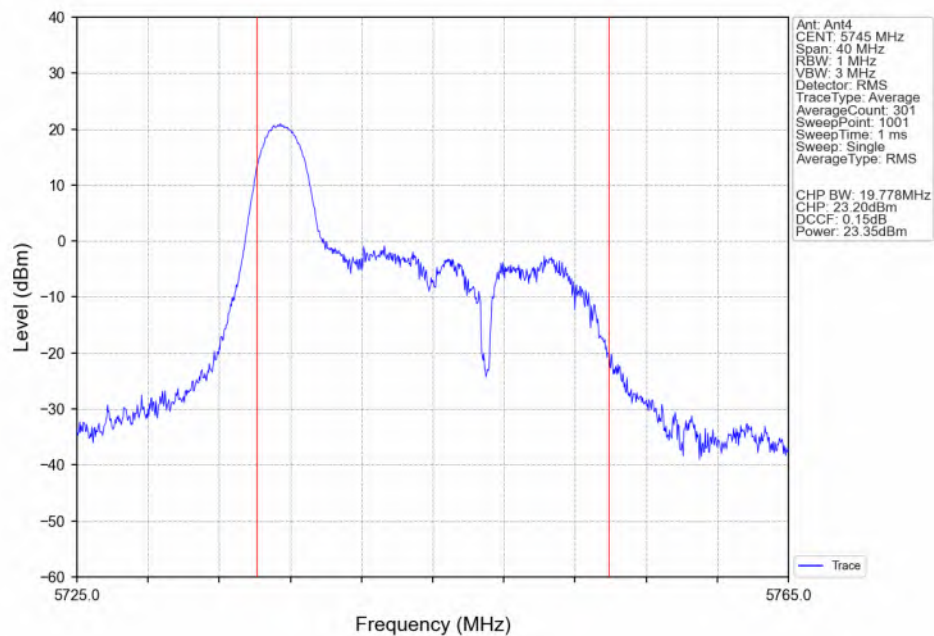
802.11ax(HEW20)_LCH_5745MHz_RU26_Left(0)_Ant4_NTNV
