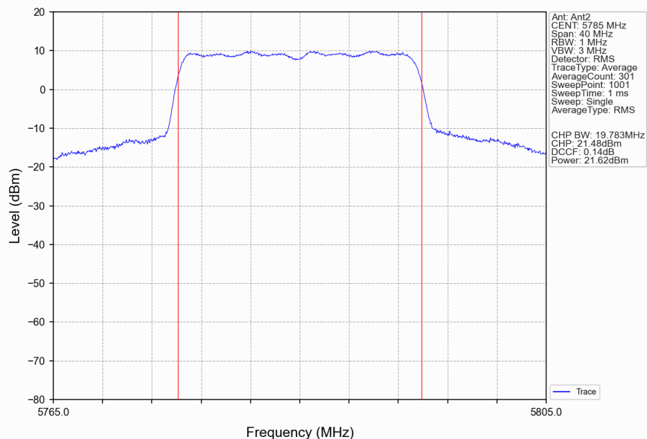
802.11ax(HEW20) MCH_5785MHz_RU242_Left(61)_Ant2_NTNV
