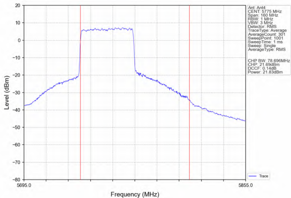
802.11ax(HEW80) MCH_5775MHz RU484 Left(65) Ant4 NTN
