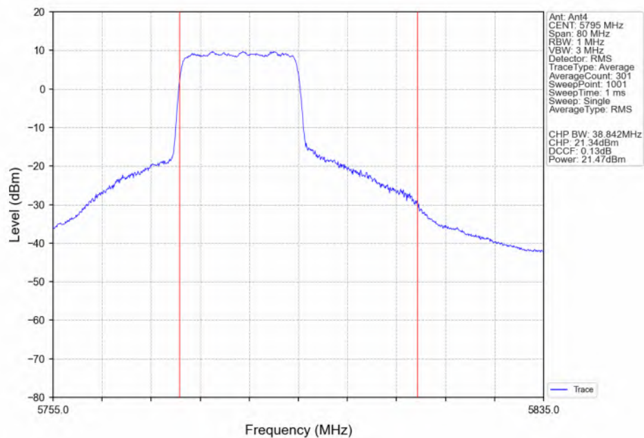
802.11ax(HEW40) HCH_5795MHz_RU242_Left(61)_Ant4_NTNV
