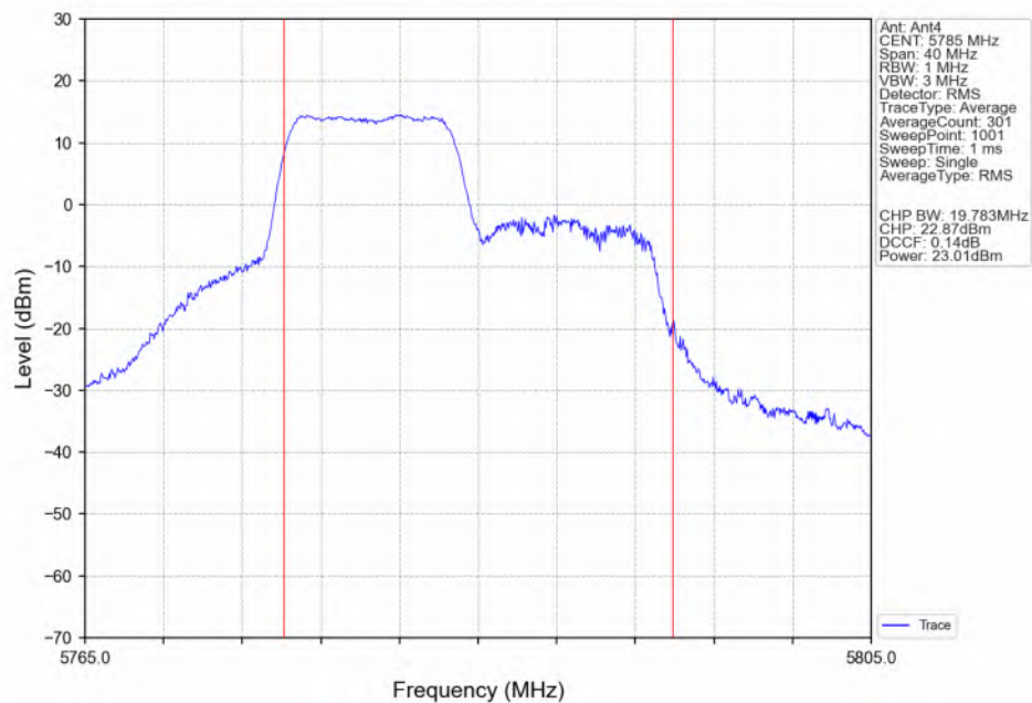
802.11ax(HEW20) MCH_5785MHz_RU106_Left(53)_Ant4_NTNV
