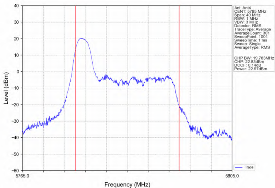
802.11ax(HEW20)_MCH_5785MHz_RU26_Left(0)_Ant4_NTNV
