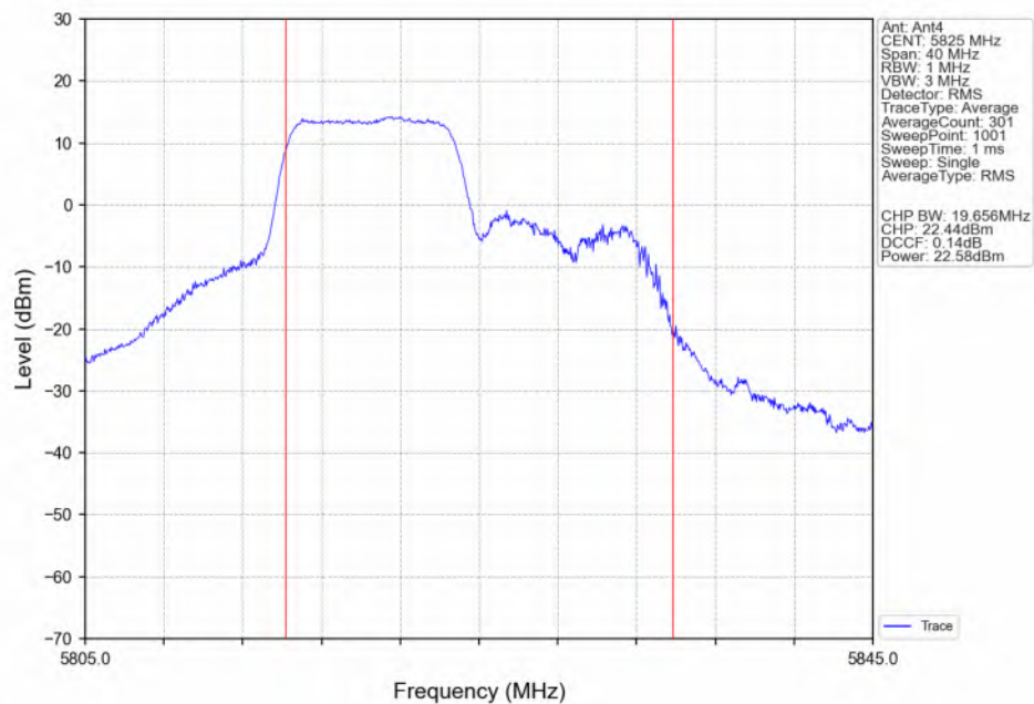
802.11ax(HEW20) HCH 5825MHz RU106 Left(53) Ant4 NTN
