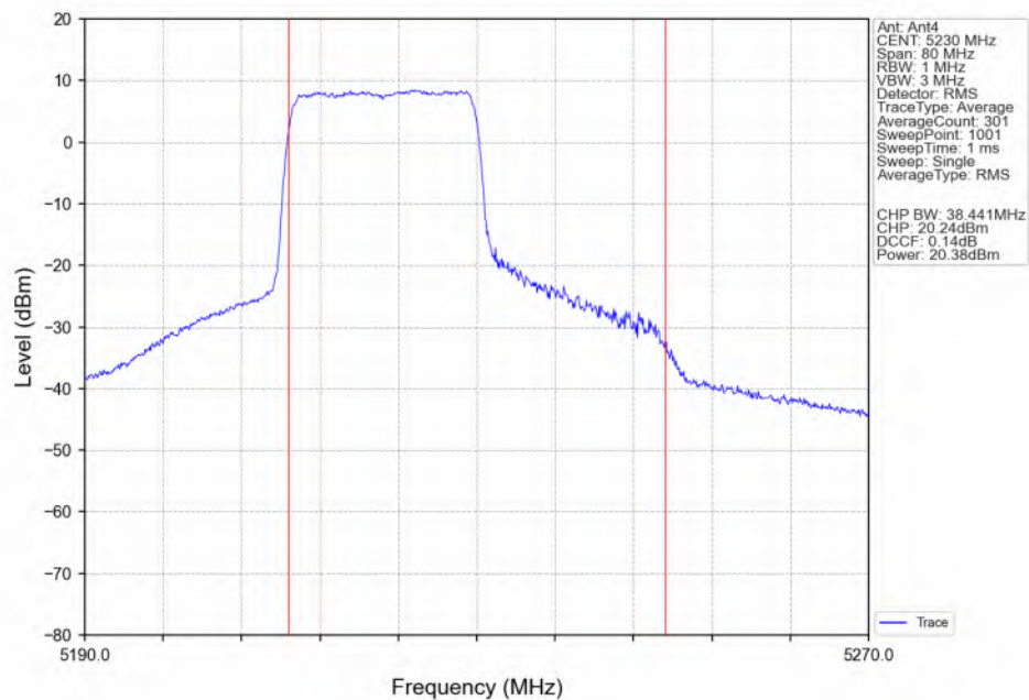
802.11ax(HEW40) HCH 5230MHz RU242 Left(61) Ant4 NTN
