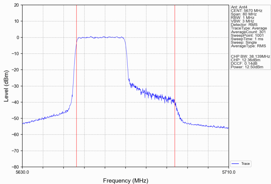
802.11ax(HEW40)_HCH_5670MHz_RU242_Left(61)_Ant4_NTNV
