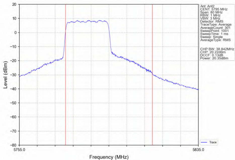
802.11ax(HEW40) HCH_5795MHz_RU242_Left(61)_Ant2_NTNV
