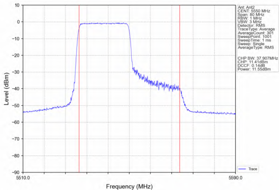
802.11ax(HEW40) MCH_5550MHz_RU242_Left(61)_Ant2_NTNV
