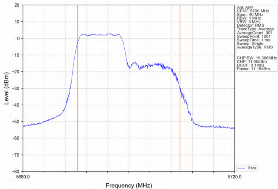
802.11ax(HEW20)_HCH_5700MHz_RU106_Left(53)_Ant4_NTNV
