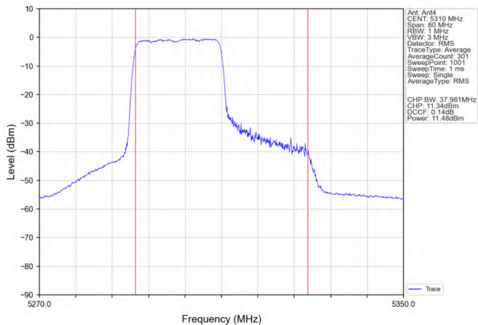
802.11ax(HEW40) HCH_5310MHz_RU242_Left(61)_Ant4_NTNV
