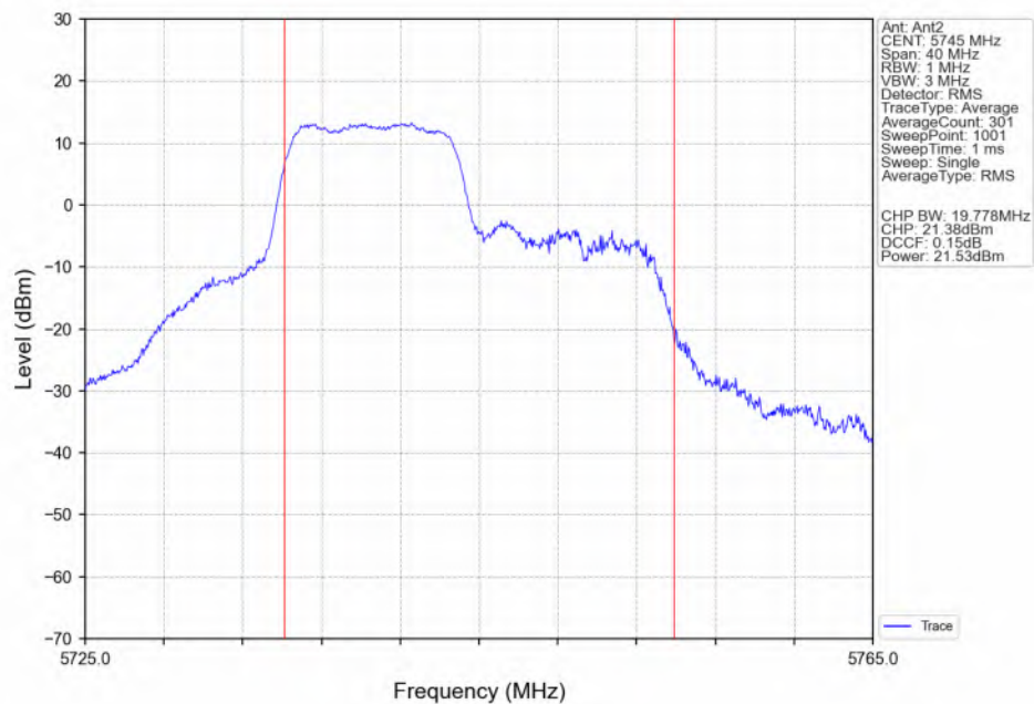
802.11ax(HEW20)_LCH_5745MHz_RU106_Left(53)_Ant2_NTNV
