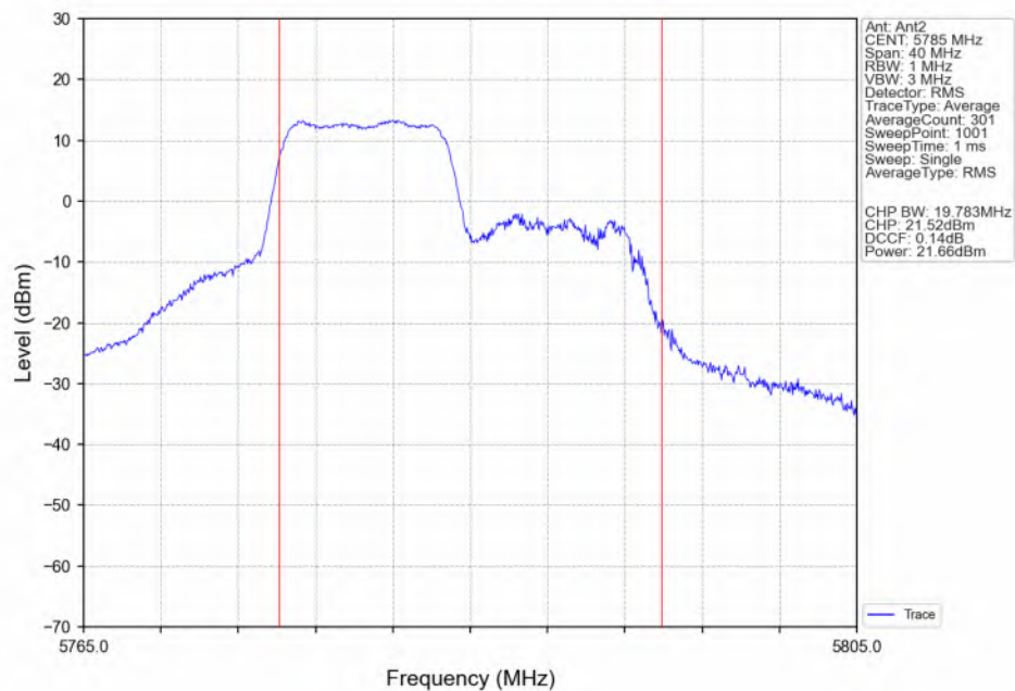
802.11ax(HEW20) MCH_5785MHz_RU106_Left(53)_Ant2_NTNV
