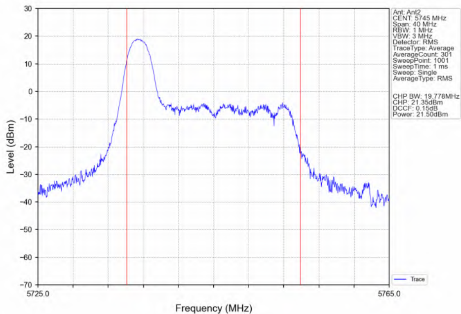
802.11ax(HEW20)_LCH_5745MHz_RU26_Left(0)_Ant2_NTNV
