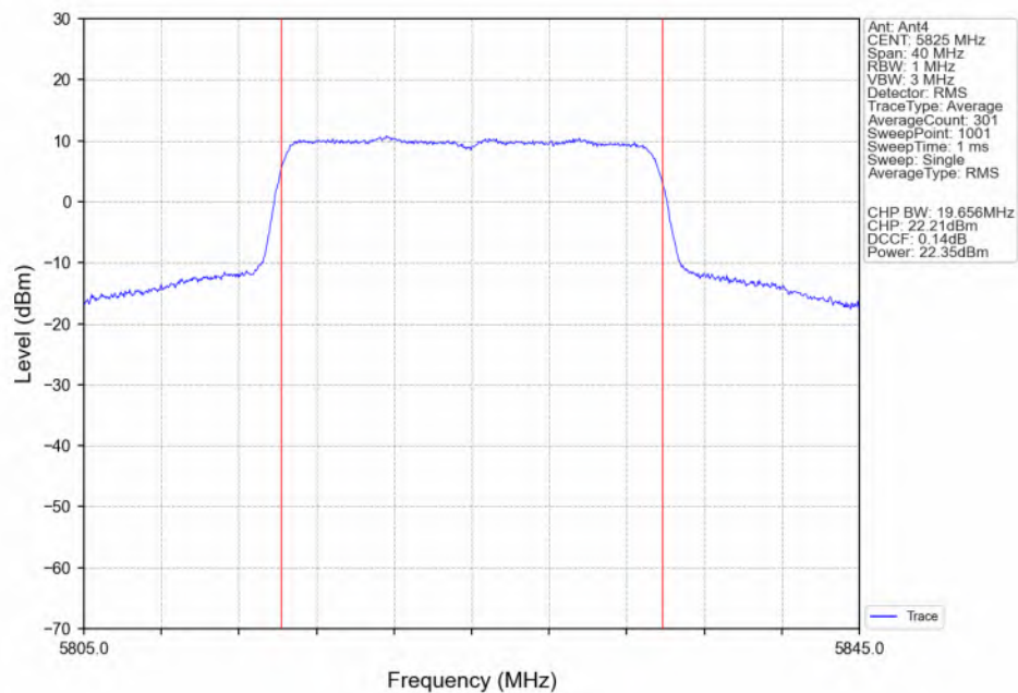
802.11ax(HEW20)_HCH_5825MHz_RU242_Left(61)_Ant4_NTNV
