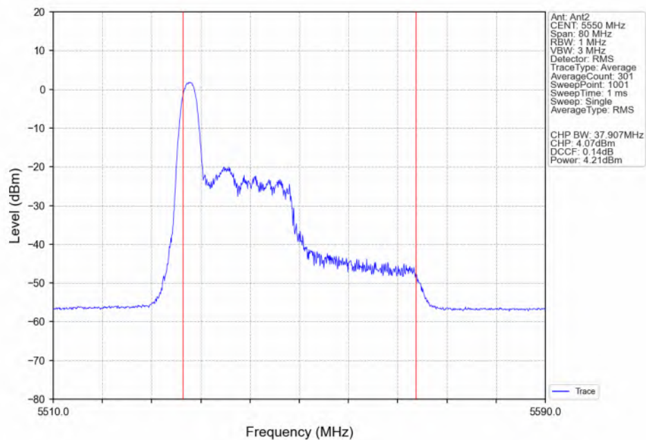
802.11ax(HEW40)_MCH_5550MHz_RU26_Left(0)_Ant2_NTNV
