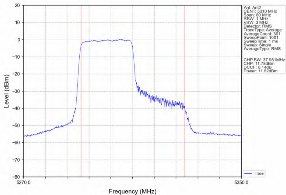
802.11ax(HEW40)_HCH_5310MHz_RU242_Left(61)_Ant2_NTNV
