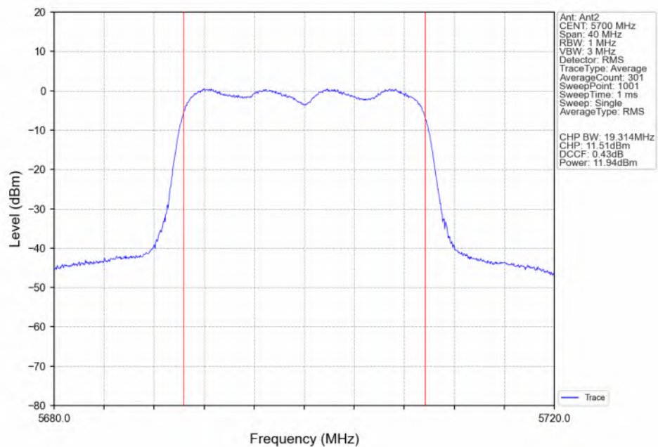
802.11ax(HEW20) HCH_5700MHz_RU242_Left(61)_Ant2_NTNV
