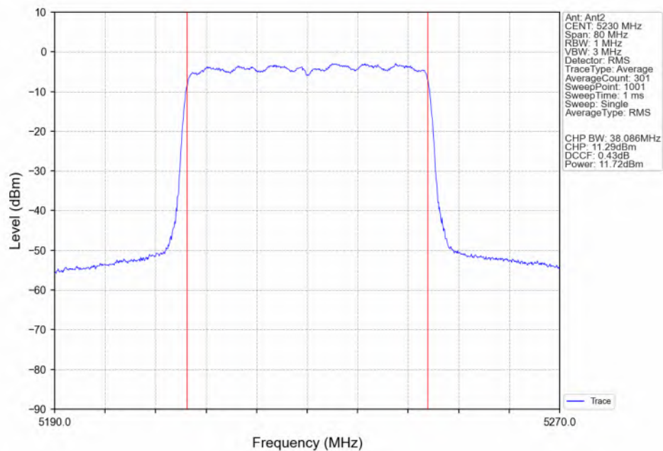
802.11ax(HEW40) HCH 5230MHz RU484 Left(65) Ant2 NTN
