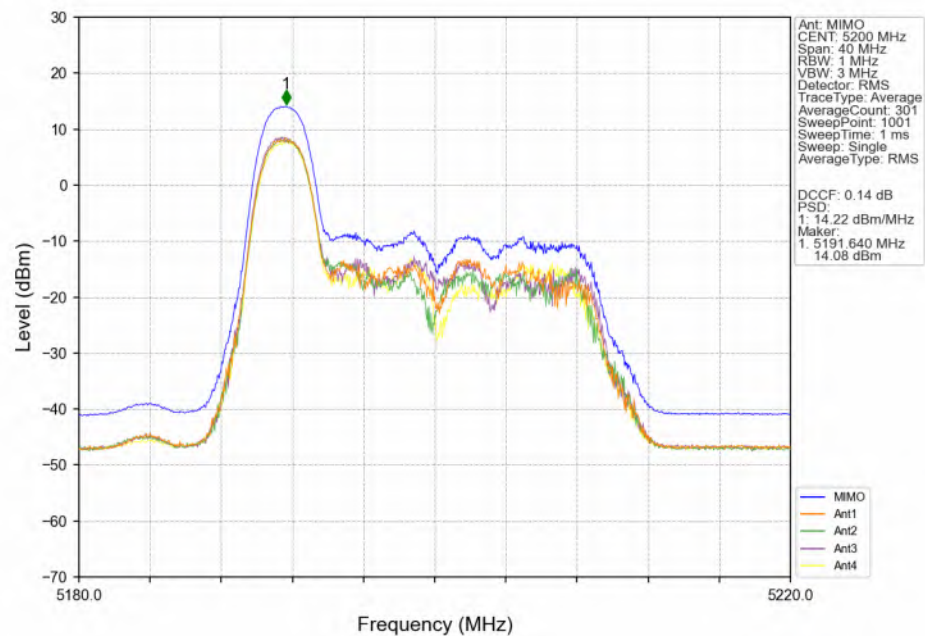
802.11ax(HEW20)_MCH_5200MHz_RU26_Left(0)_MIMO_NTNV
