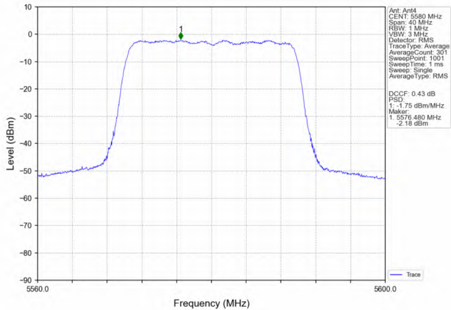
802.11ax(HEW20) MCH_5580MHz_RU242_Left(61)_MIMO_NTNV
