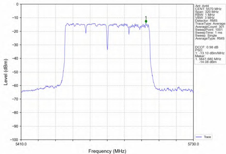
802.11ac(VHT160)_MCH_5570MHz_Ant4_NTNV
