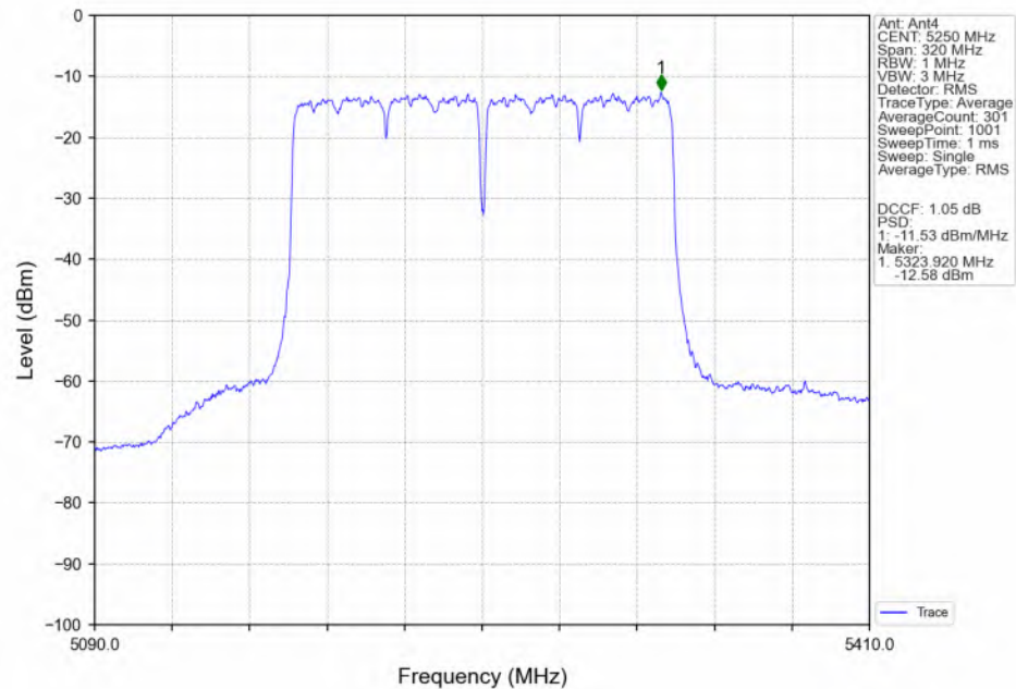
802.11ac(VHT160)_MCH_5250MHz_MIMO_NTNV
