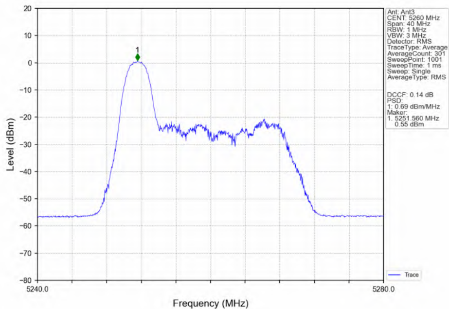
802.11ax(HEW20)_LCH_5260MHz_RU26_Left(0)_Ant3_NTNV
