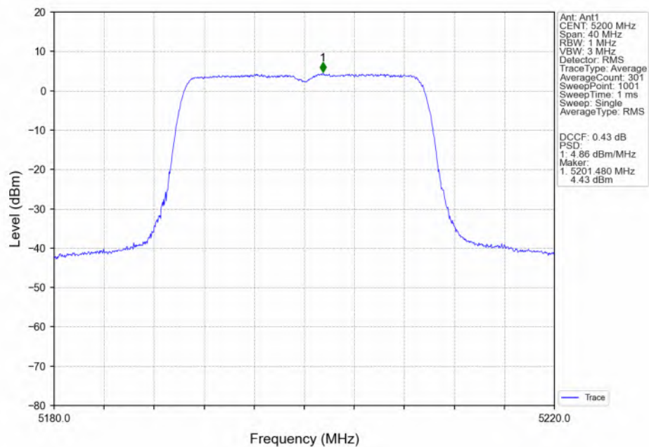
802.11ax(HEW20)_MCH_5200MHz_RU242_Left(61)_Ant1_NTNV
