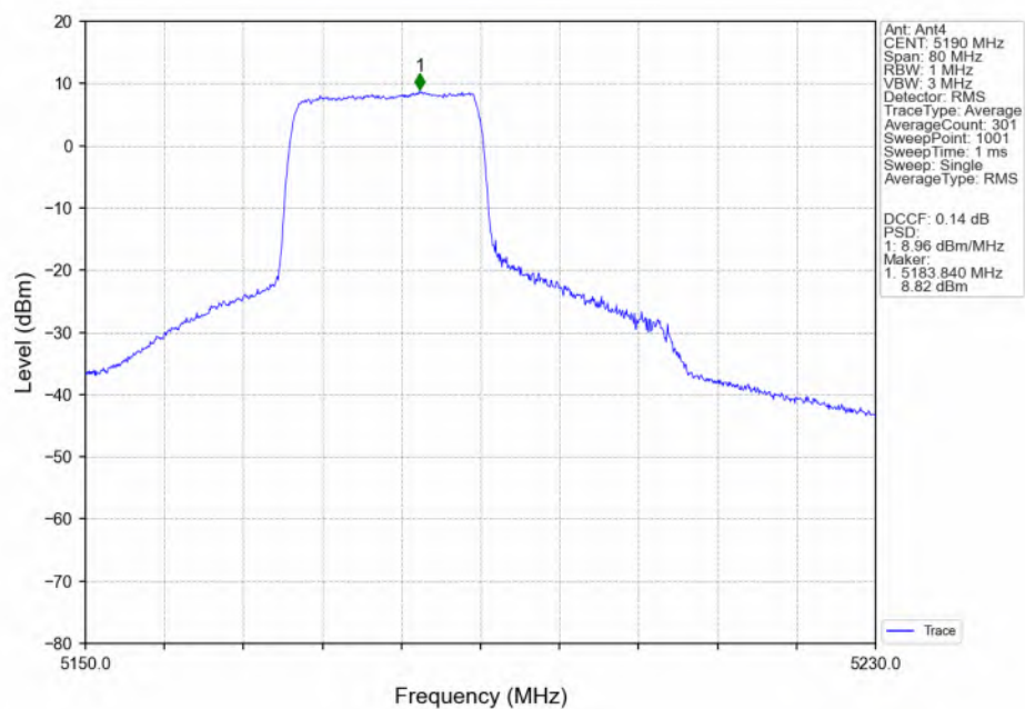
802.11ax(HEW40)_LCH_5190MHz_RU242_Left(61)_Ant4_NTNV
