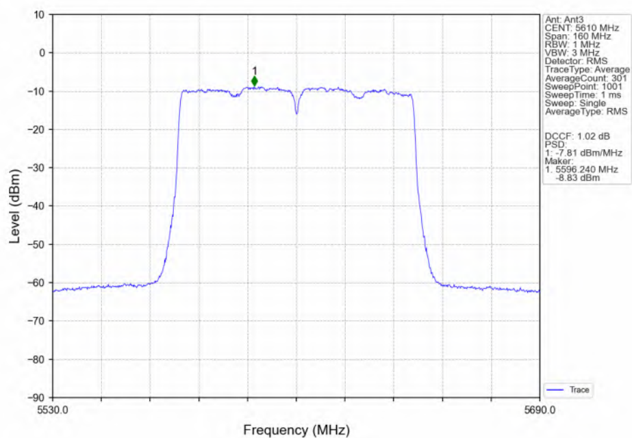
802.11ac(VHT80)_HCH_5610MHz_Ant3_NTNV
