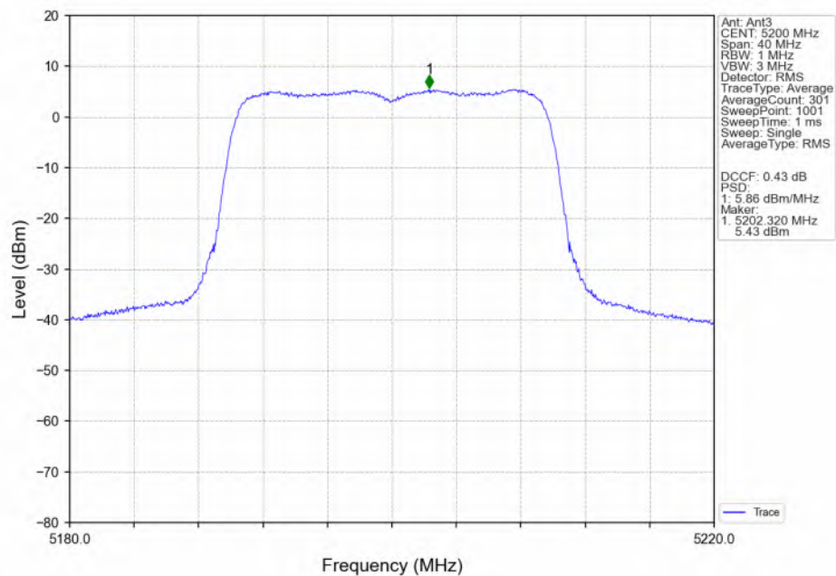
802.11ax(HEW20) MCH_5200MHz_RU242_Left(61)_Ant3_NTNV
