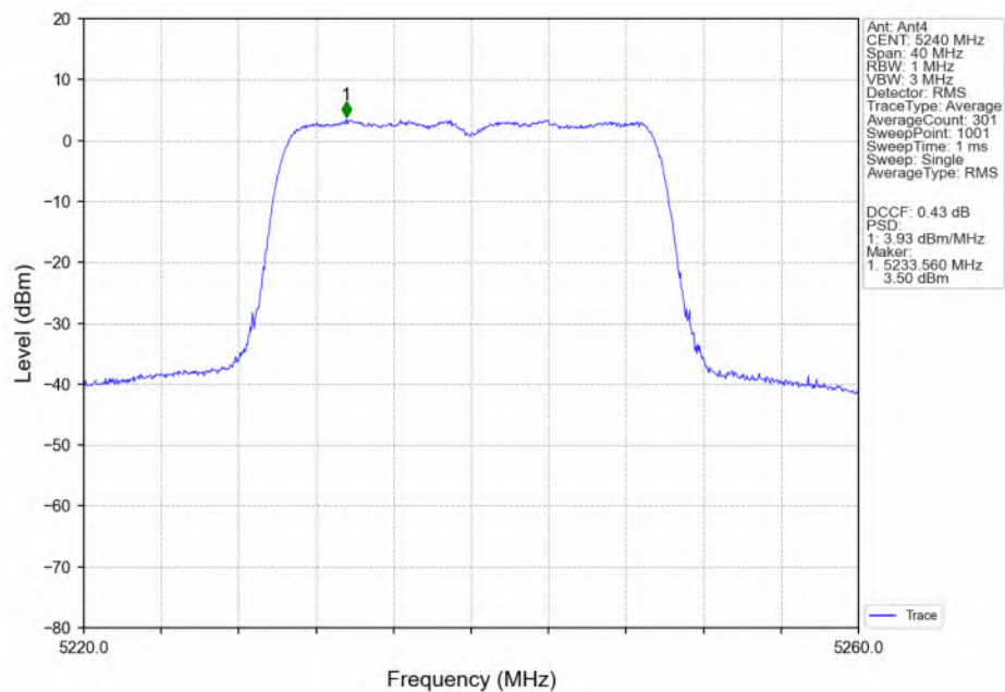
802.11ax(HEW20)_HCH_5240MHz_RU242_Left(61)_Ant4_NTNV
