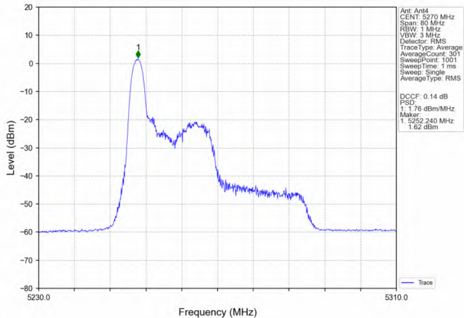
802.11ax(HEW40)_LCH_5270MHz_RU26_Left(0)_MIMO_NTNV
