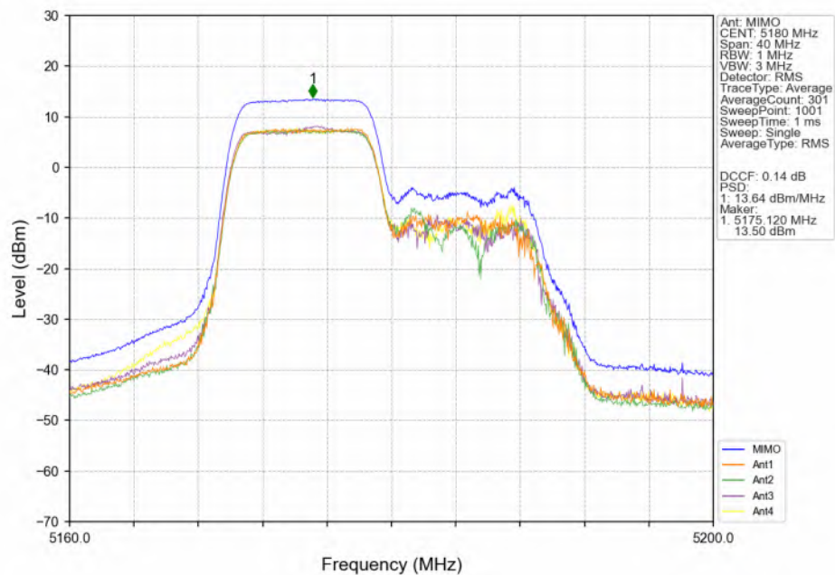
802.11ax(HEW20)_LCH_5180MHz_RU106_Left(53)_MIMO_NTNV
