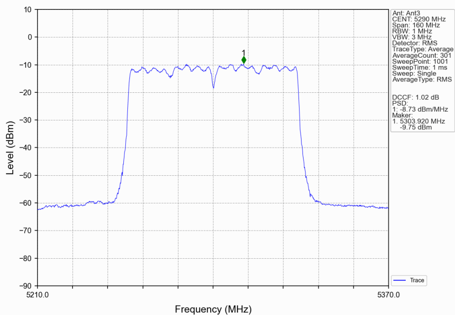
802.11ac(VHT80)_MCH_5290MHz_Ant3_NTNV
