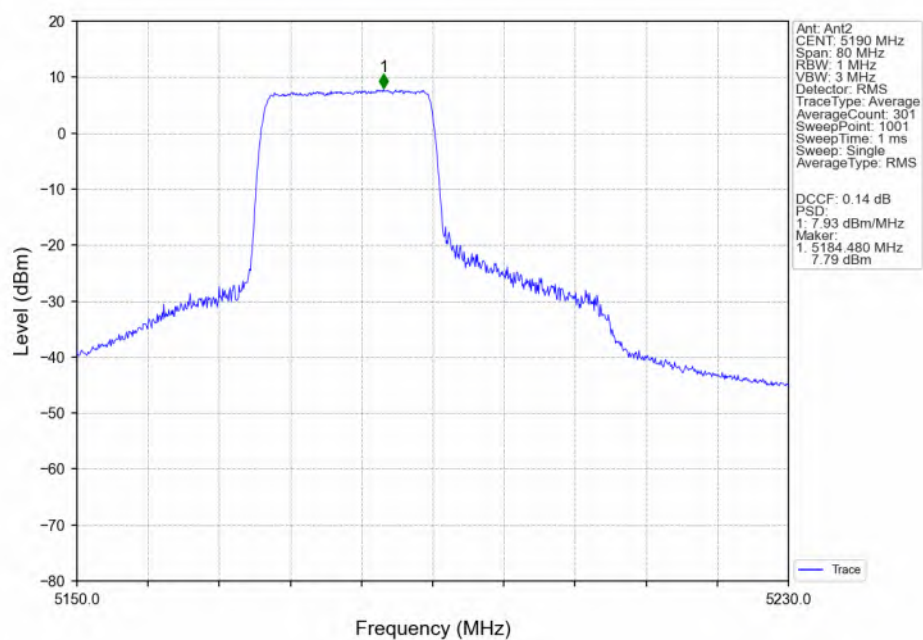
802.11ax(HEW40)_LCH_5190MHz_RU242_Left(61)_Ant2_NTNV
