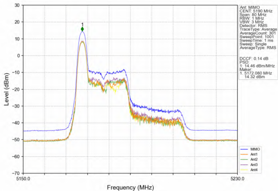
802.11ax(HEW40)_LCH_5190MHz_RU26_Left(0)_MIMO_NTNV
