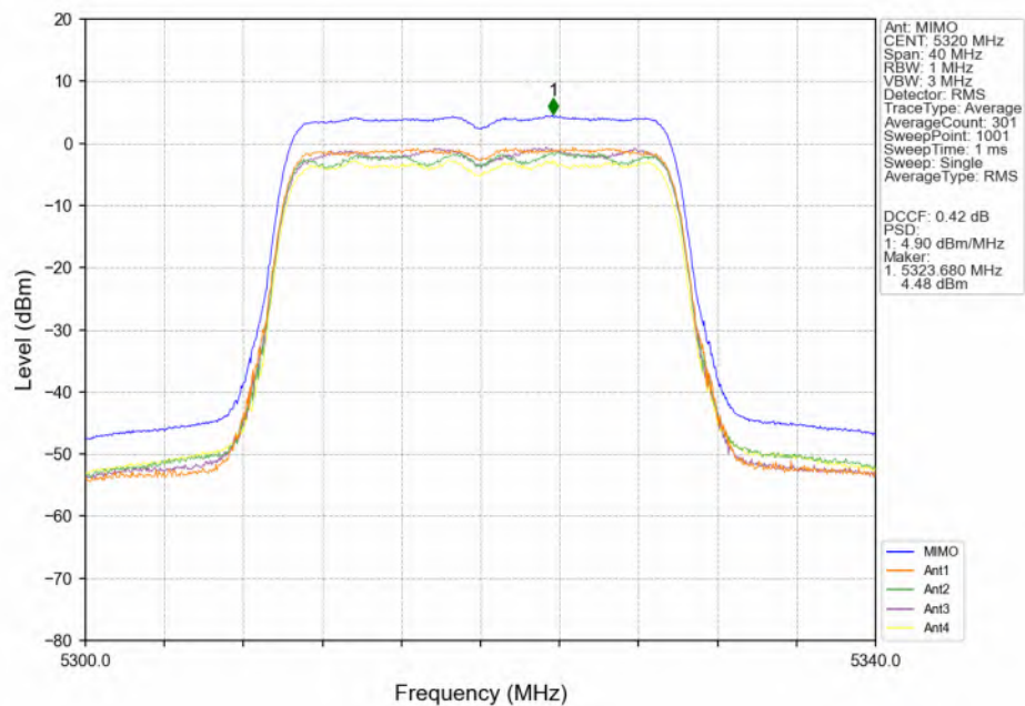
802.11ax(HEW20)_HCH_5320MHz_RU242_Left(61)_MIMO_NTNV
