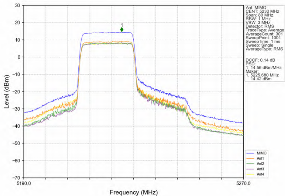
802.11ax(HEW40) HCH_5230MHz_RU242_Left(61)_MIMO_NTNV
