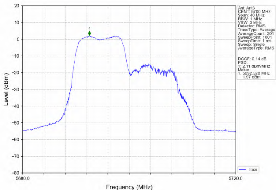
802.11ax(HEW20)_HCH_5700MHz_RU106_Left(53)_Ant3_NTNV
