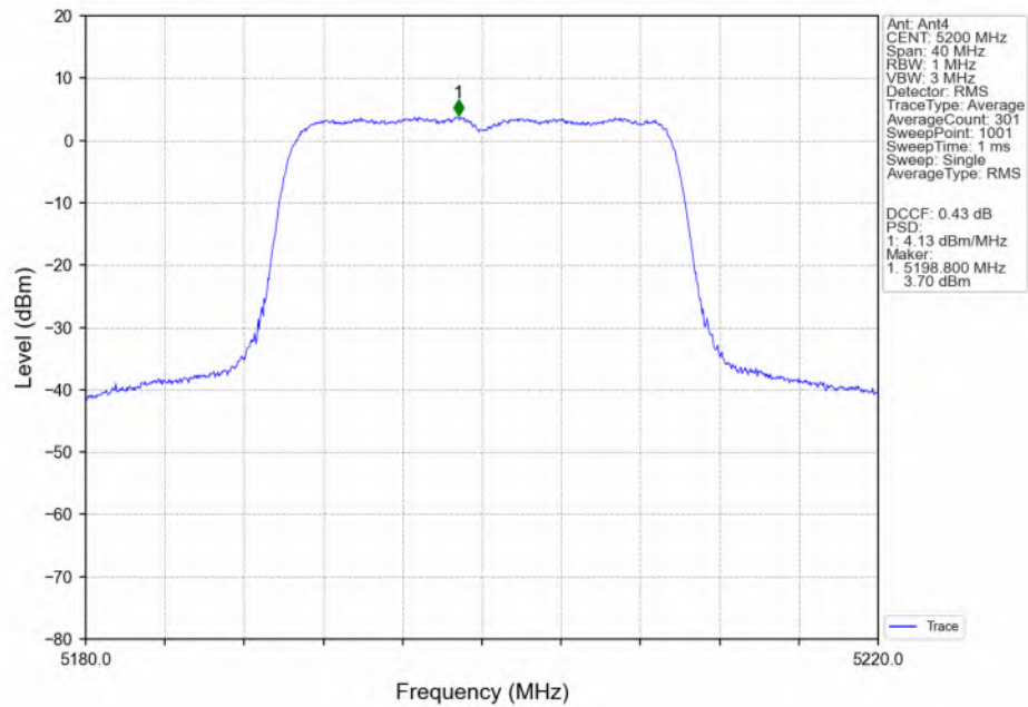
802.11ax(HEW20) MCH_5200MHz_RU242_Left(61)_MIMO_NTNV
