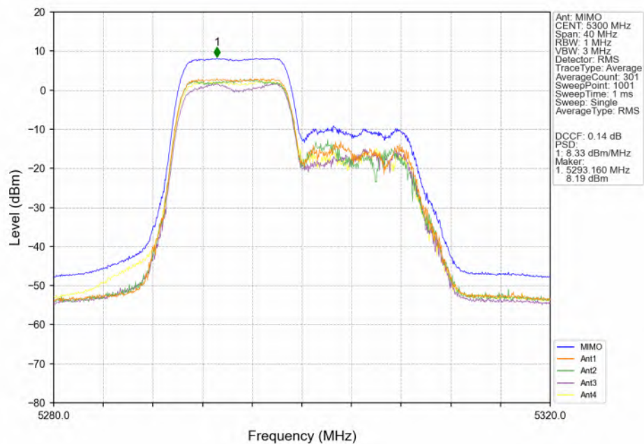
802.11ax(HEW20) MCH_5300MHz_RU106_Left(53)_MIMO_NTNV
