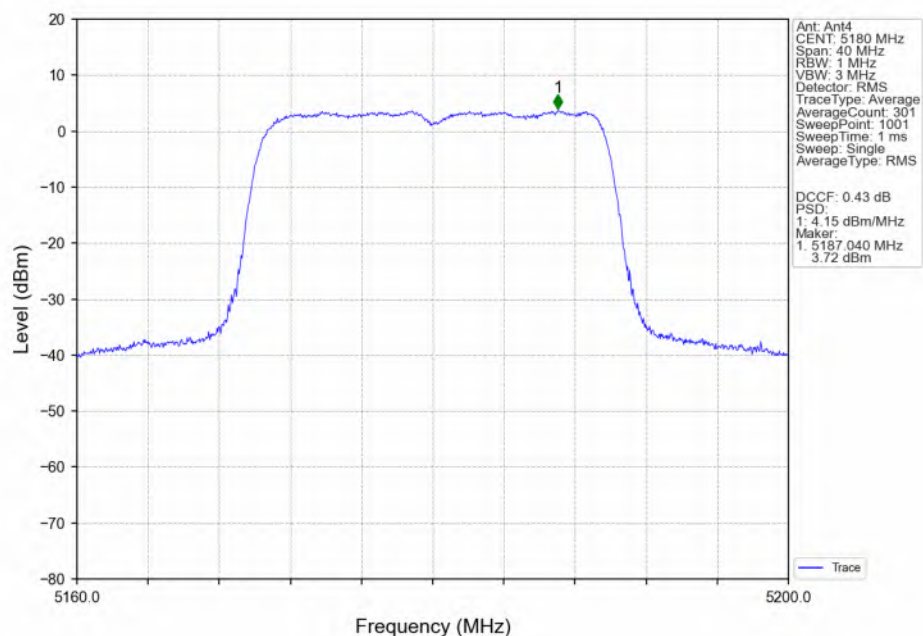
802.11ax(HEW20)_LCH_5180MHz_RU242_Left(61)_Ant4_NTNV
