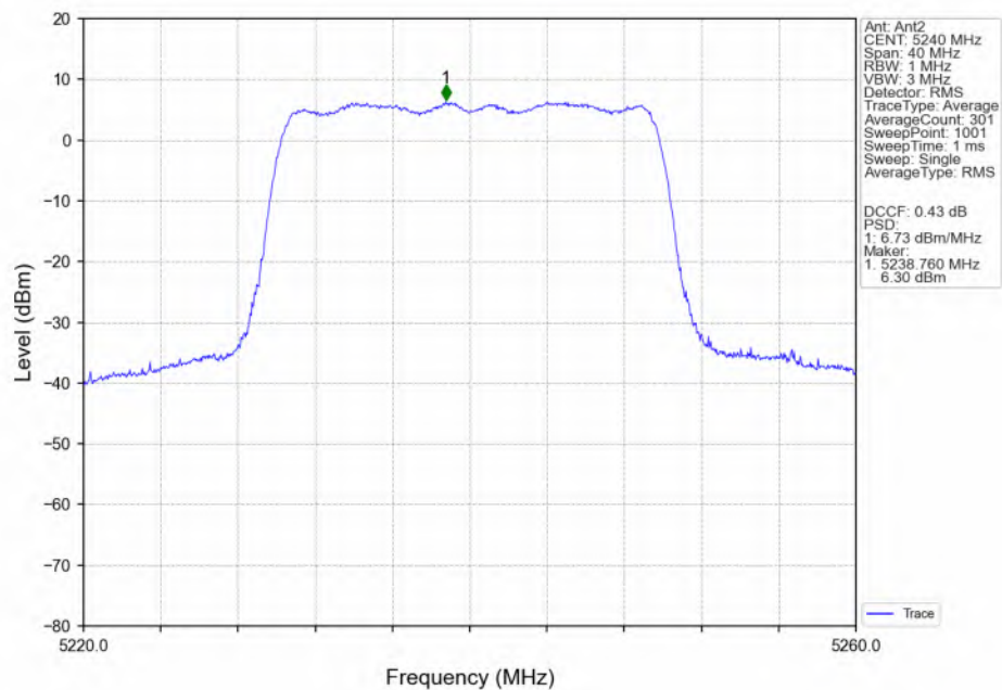
802.11ax(HEW20)_HCH_5240MHz_RU242_Left(61)_Ant2_NTNV
