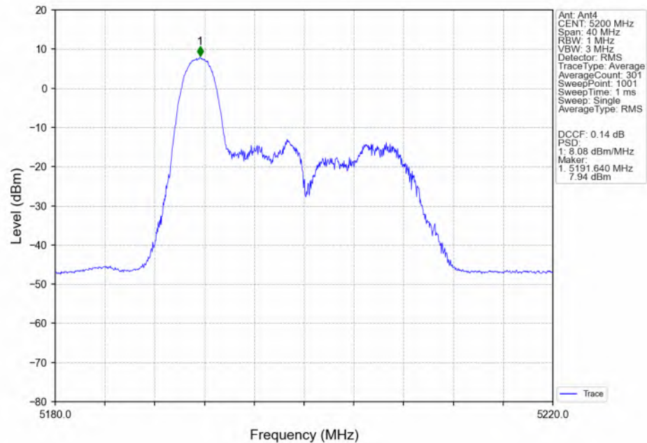
802.11ax(HEW20)_MCH_5200MHz_RU26_Left(0)_MIMO_NTNV
