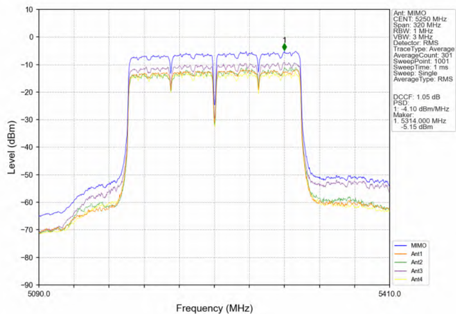
802.11ac(VHT160)_MCH_5250MHz_MIMO_NTNV
