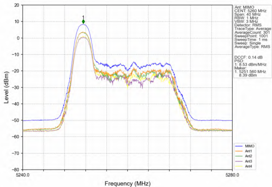
802.11ax(HEW20)_LCH_5260MHz_RU26_Left(0)_MIMO_NTNV
