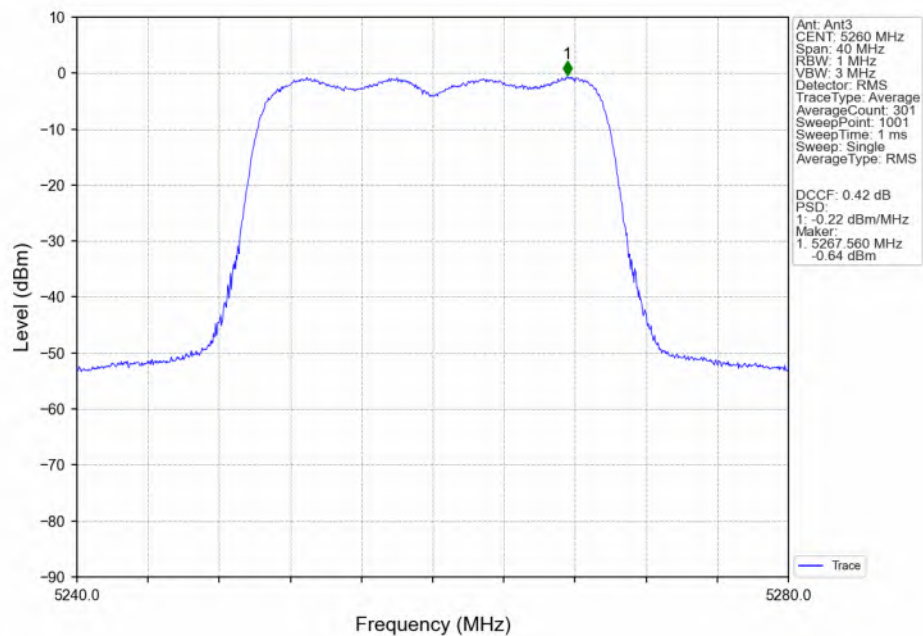
802.11ax(HEW20)_LCH_5260MHz_RU242_Left(61)_Ant3_NTNV
