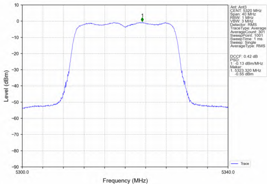
802.11ax(HEW20)_HCH_5320MHz_RU242_Left(61)_Ant3_NTNV
