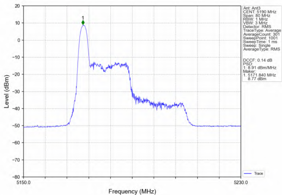
802.11ax(HEW40)_LCH_5190MHz_RU26_Left(0)_Ant3_NTNV
