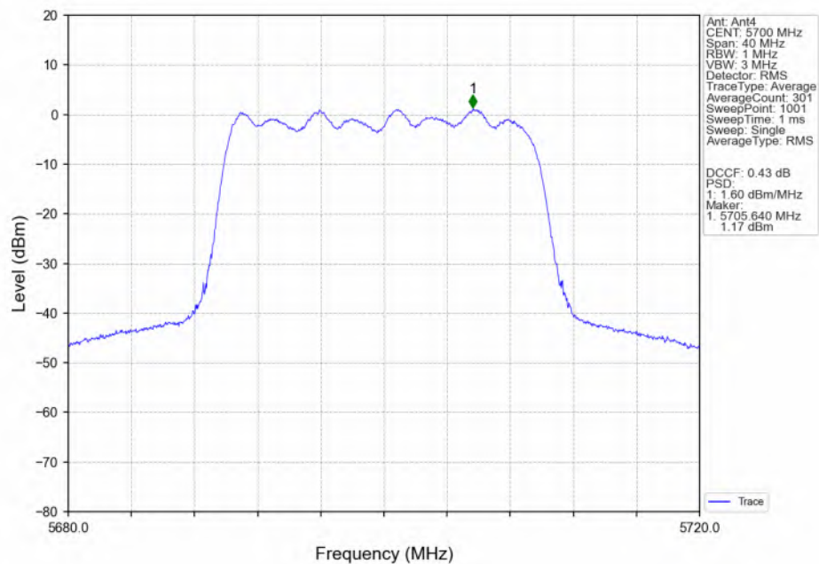
802.11ax(HEW20)_HCH_5700MHz_RU242_Left(61)_Ant4_NTNV
