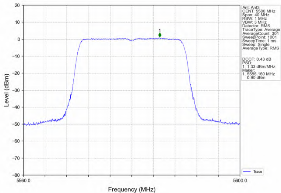
802.11ax(HEW20) MCH_5580MHz_RU242_Left(61)_Ant3_NTNV
