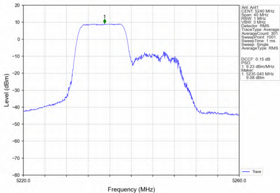
802.11ax(HEW20)_HCH_5240MHz_RU106_Left(53)_Ant1_NTNV
