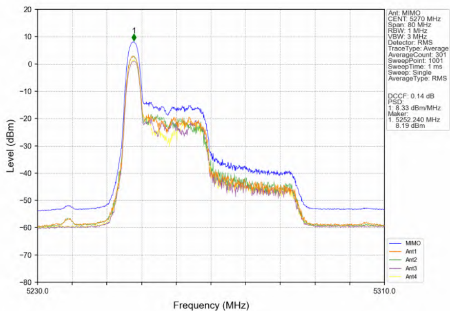
802.11ax(HEW40)_LCH_5270MHz_RU26_Left(0)_MIMO_NTNV
