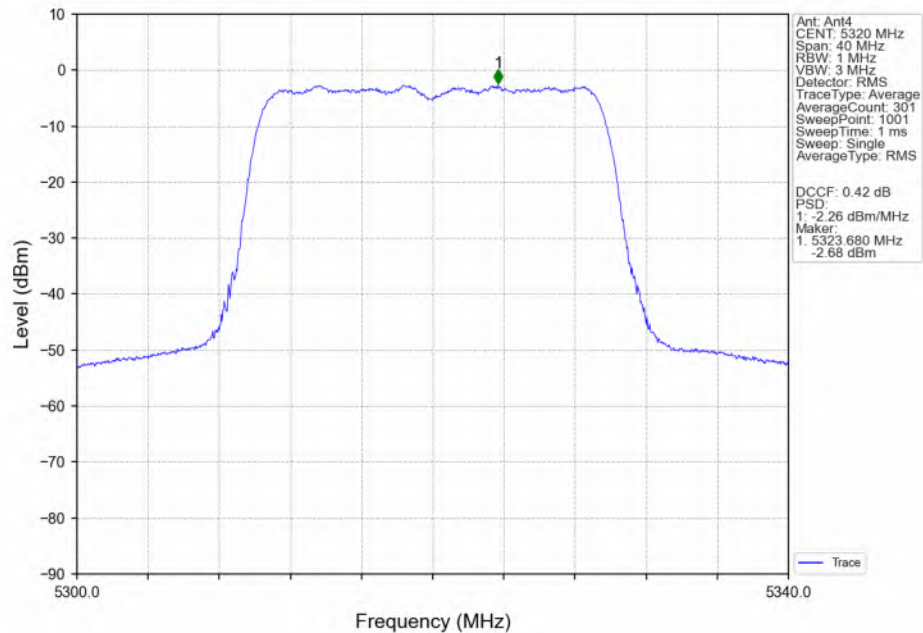
802.11ax(HEW20)_HCH_5320MHz_RU242_Left(61)_MIMO_NTNV
