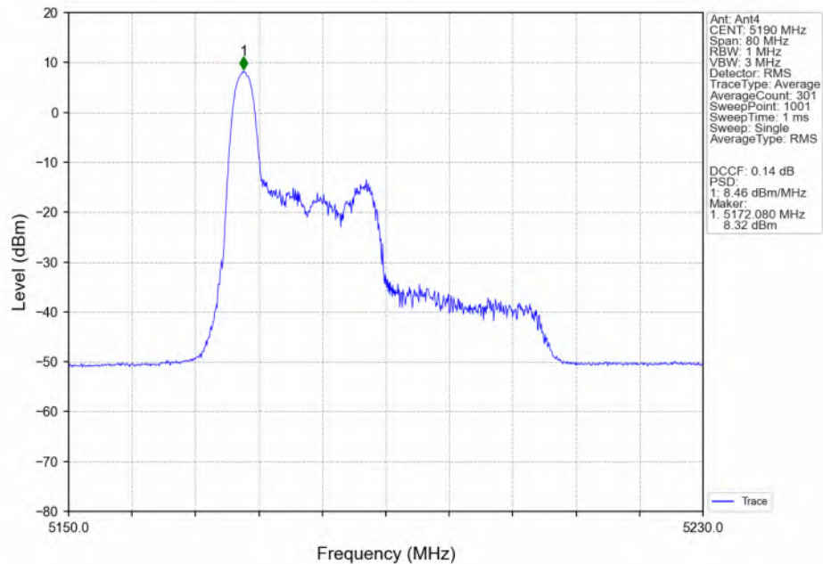
802.11ax(HEW40)_LCH_5190MHz_RU26_Left(0)_MIMO_NTNV
