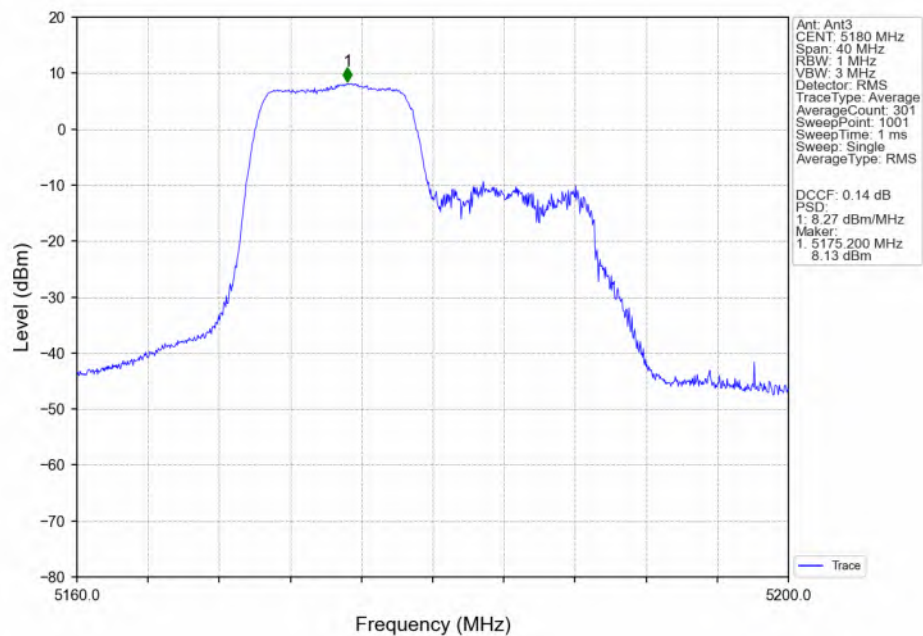
802.11ax(HEW20)_LCH_5180MHz_RU106_Left(53)_Ant3_NTNV
