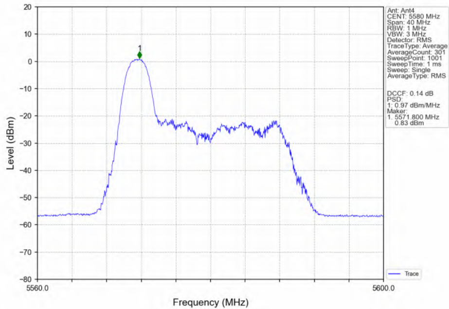
802.11ax(HEW20)_MCH_5580MHz_RU26_Left(0)_MIMO_NTNV
