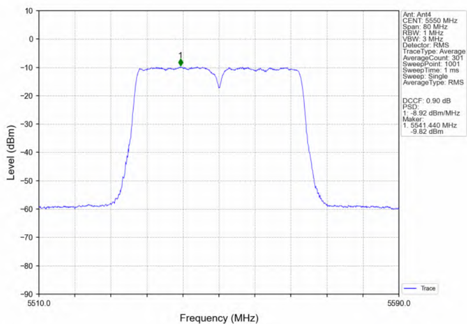
802.11ac(VHT40)_MCH_5550MHz_Ant4_NTNV
