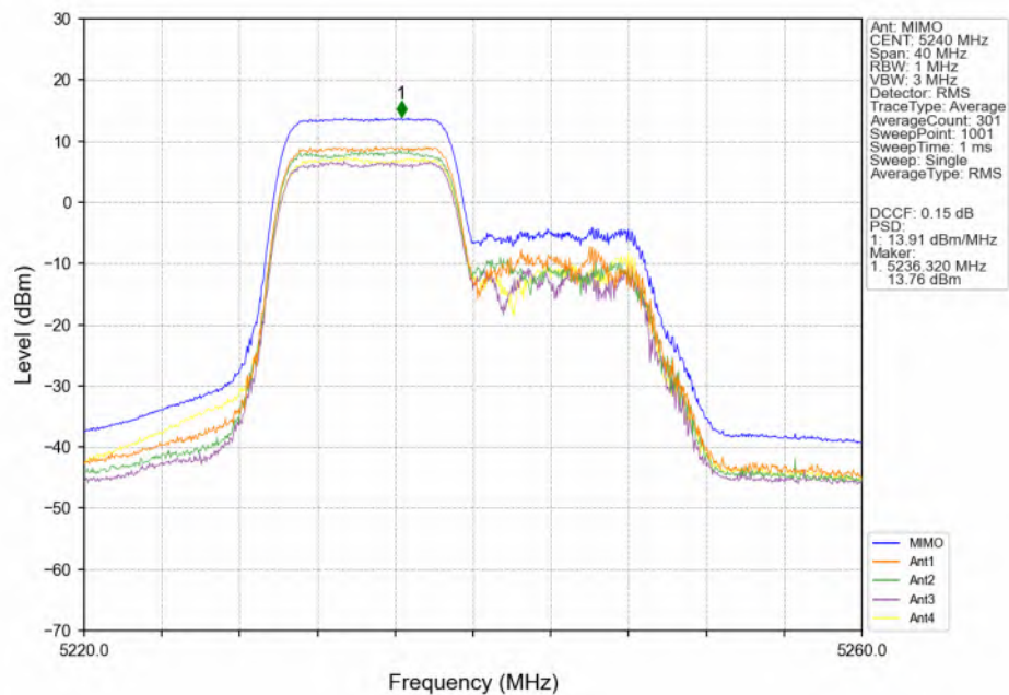
802.11ax(HEW20) HCH_5240MHz_RU106_Left(53)_MIMO_NTNV
