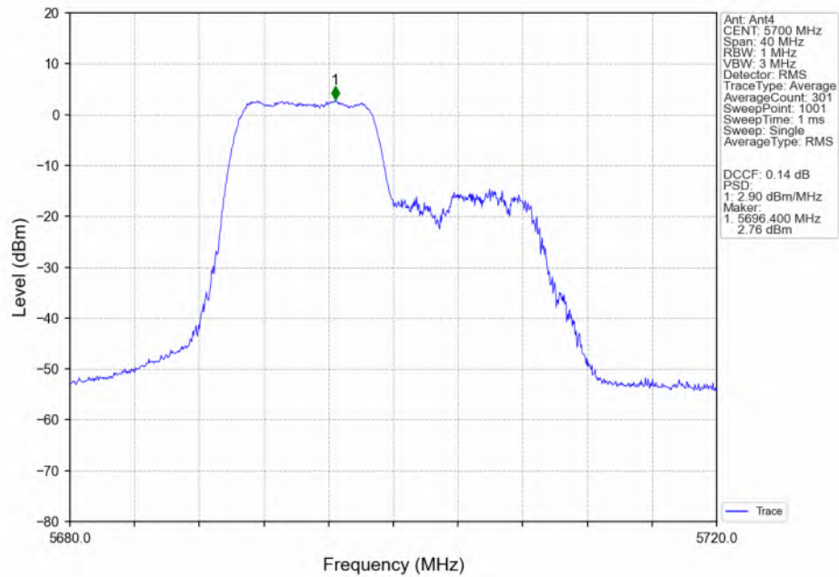
802.11ax(HEW20)_HCH_5700MHz_RU106_Left(53)_MIMO_NTNV
