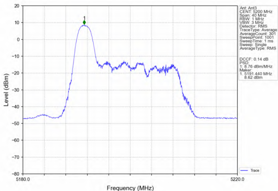
802.11ax(HEW20) MCH_5200MHz_RU26_Left(0)_Ant3_NTNV
