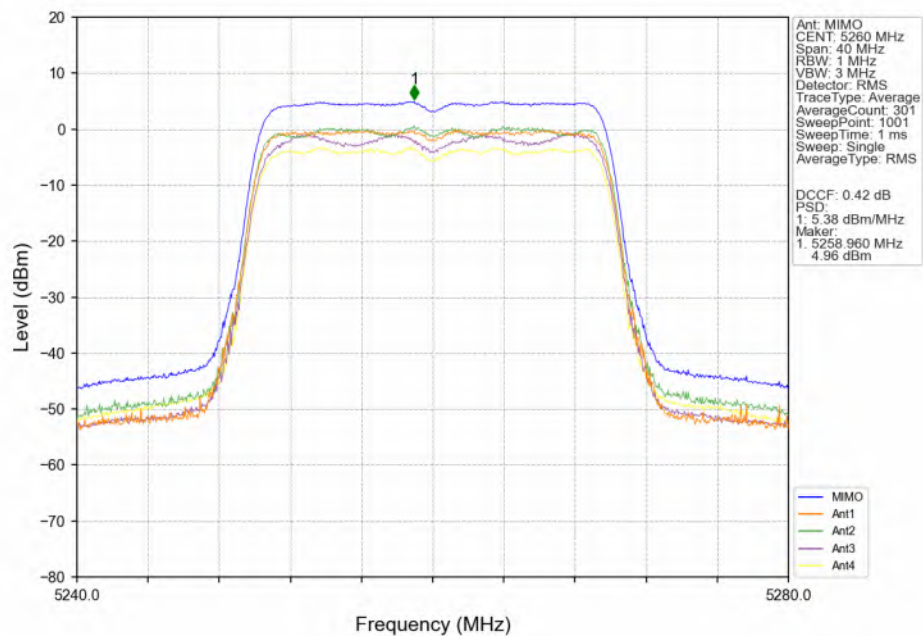
802.11ax(HEW20)_LCH_5260MHz_RU242_Left(61)_MIMO_NTNV
