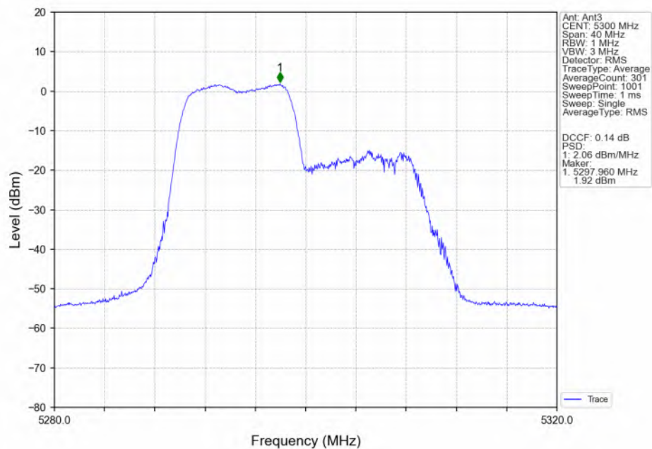
802.11ax(HEW20) MCH_5300MHz_RU106_Left(53)_Ant3_NTNV
