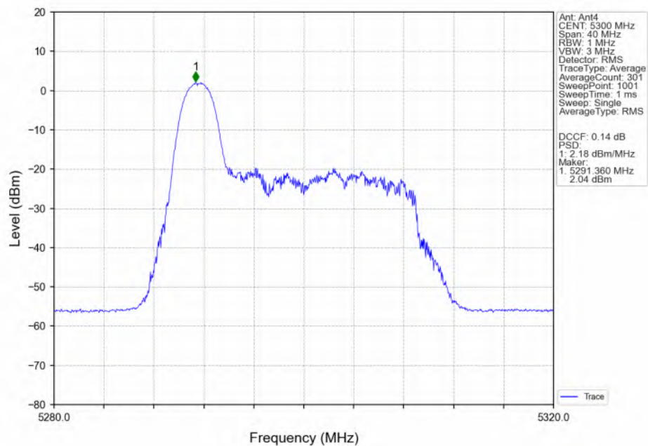
802.11ax(HEW20)_MCH_5300MHz_RU26_Left(0)_Ant4_NTNV
