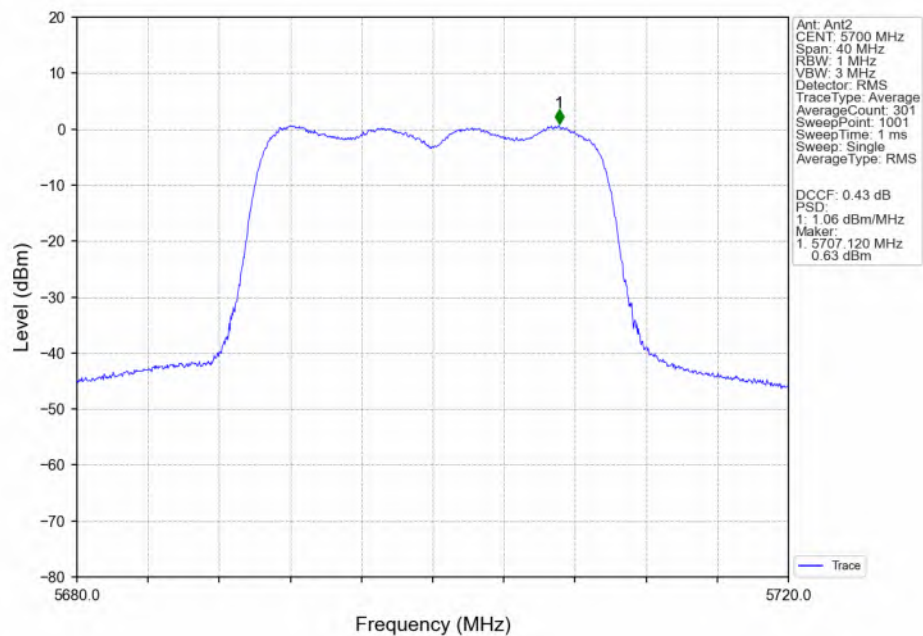
802.11ax(HEW20)_HCH_5700MHz_RU242_Left(61)_Ant2_NTNV
