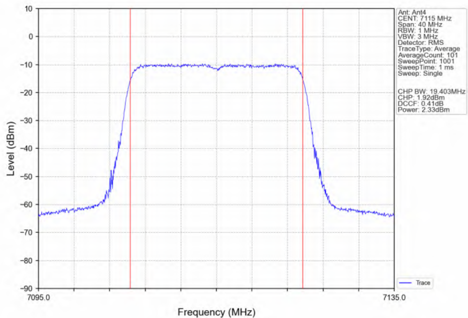
802.11ax(HEW20)_HCH_7115MHz_SU_ / Ant4_NTNV
