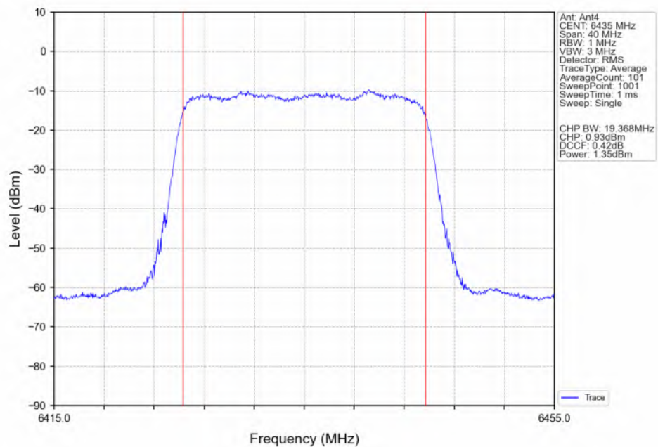
802.11ax(HEW20)_LCH_6435MHz_SU_ / Ant4_NTNV
