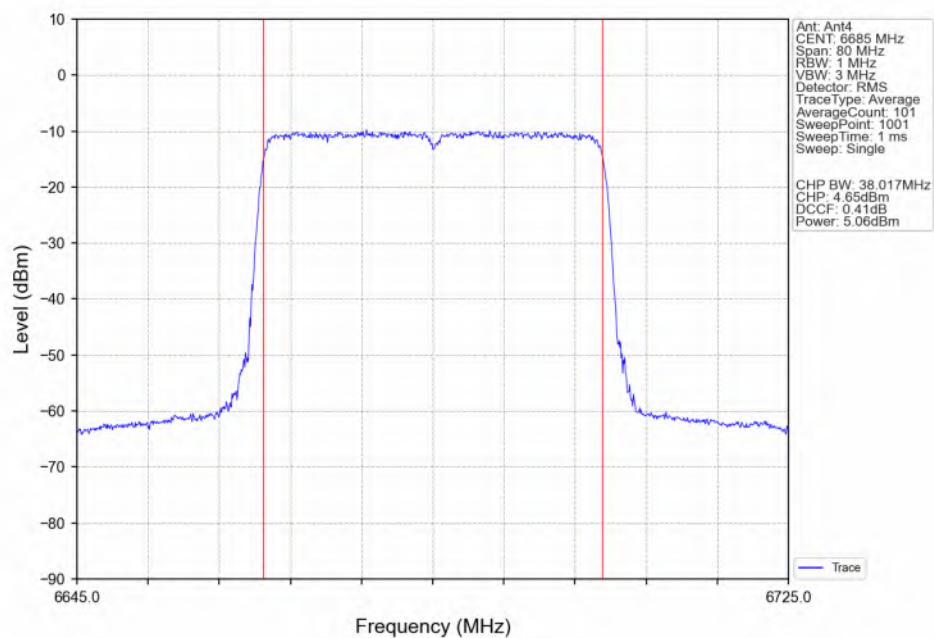
802.11ax(HEW40)_MCH_6685MHz_SU_ / Ant4_NTNV
