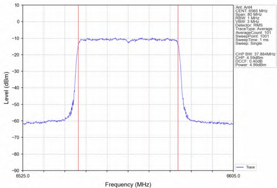
802.11ax(HEW40)_LCH_6565MHz_SU_ / Ant4_NTNV
