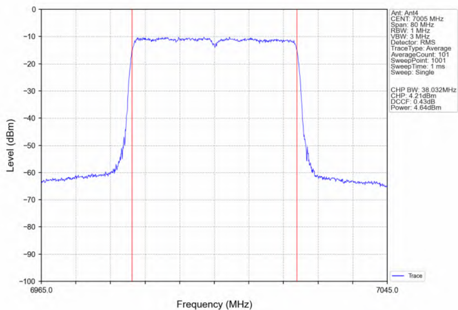
802.11ax(HEW40)_MCH_7005MHz_SU_ / Ant4_NTNV
