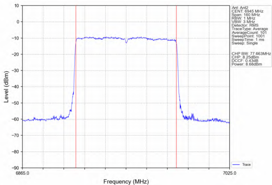
802.11ax(HEW80)_LCH_6945MHz_SU_ / Ant2_NTNV
