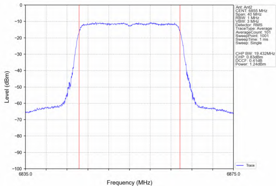
802.11ax(HEW20)_HCH_6855MHz_SU_ / Ant2_NTNV
