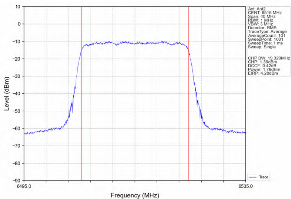
802.11ax(HEW20)_HCH_6515MHz_SU_ / Ant2_NTNV
