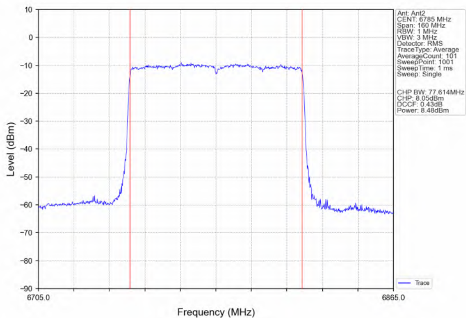
802.11ax(HEW80)_HCH_6785MHz_SU_ / Ant2_NTNV
