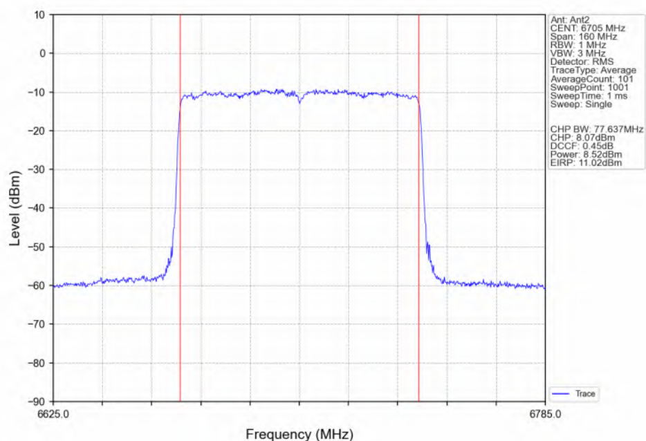
802.11ax(HEW80)_MCH_6705MHz_SU_ / Ant2_NTNV
