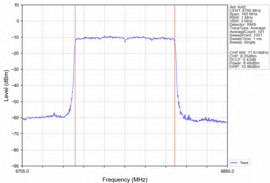
802.11ax(HEW80)_HCH_6785MHz_SU_ / Ant2_NTNV
