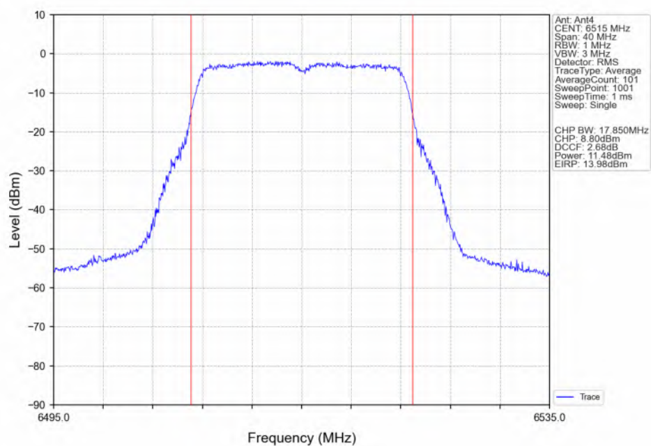
802.11a_HCH_6515MHz_Ant4_NTNV
