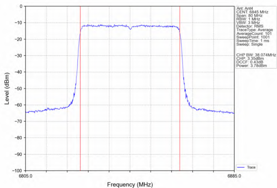
802.11ax(HEW40)_HCH_6845MHz_SU_ / Ant4_NTNV
