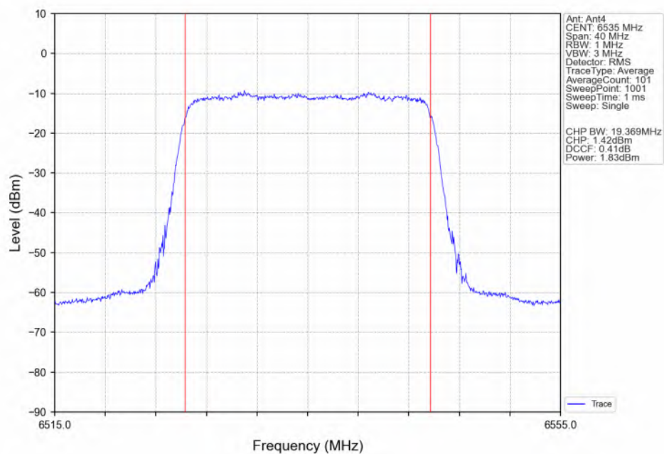
802.11ax(HEW20)_LCH_6535MHz_SU_ / Ant4_NTNV
