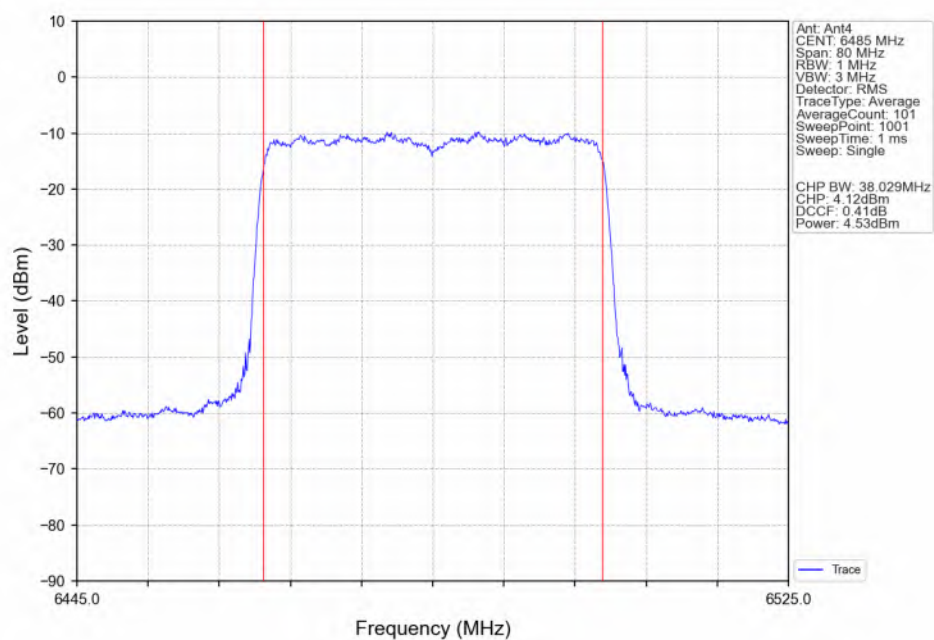
802.11ax(HEW40)_MCH_6485MHz_SU_ / Ant4_NTNV
