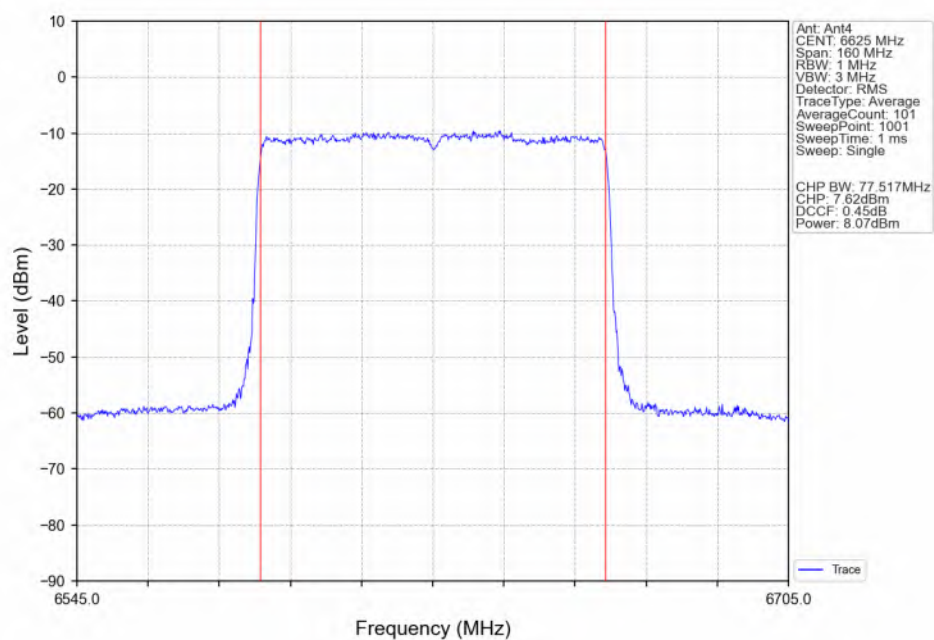
802.11ax(HEW80)_LCH_6625MHz_SU_ / Ant4_NTNV
