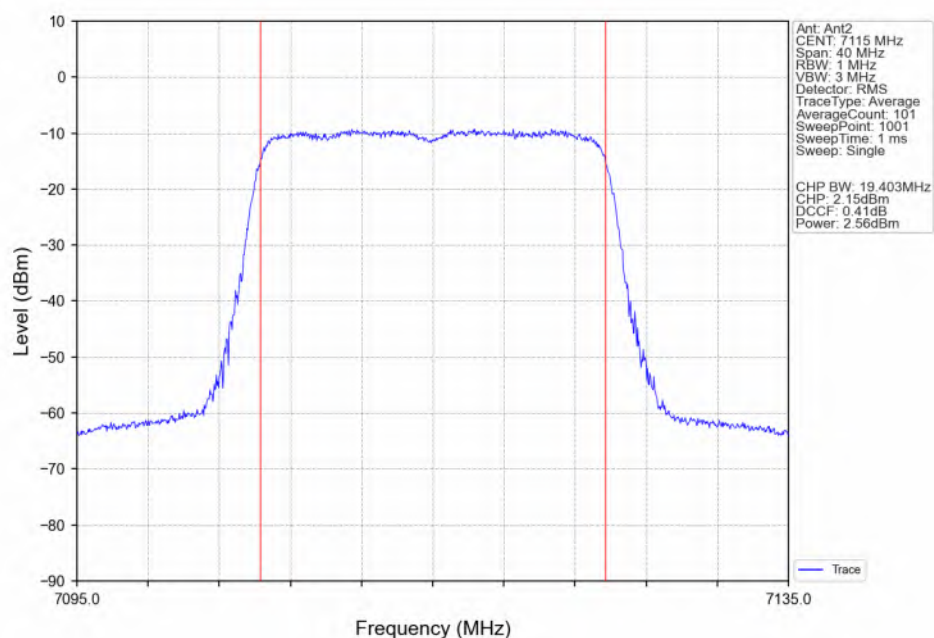
802.11ax(HEW20)_HCH_7115MHz_SU_ / Ant2_NTNV
