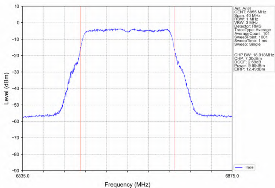
802.11a_HCH_6855MHz_Ant4_NTNV
