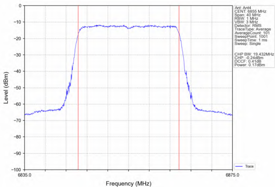
802.11ax(HEW20)_HCH_6855MHz_SU_ / Ant4_NTNV
