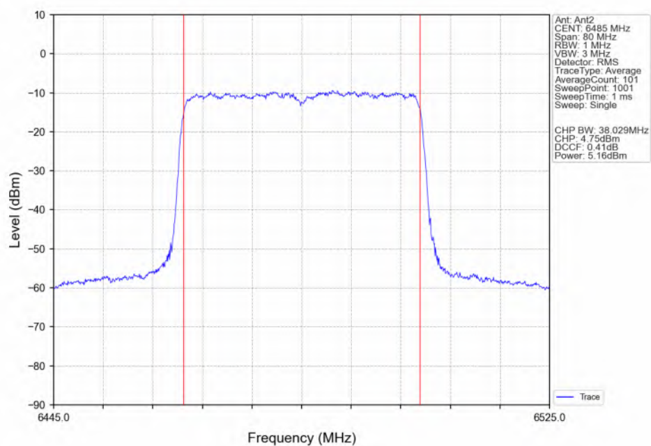
802.11ax(HEW40)_MCH_6485MHz_SU_ / Ant2_NTNV
