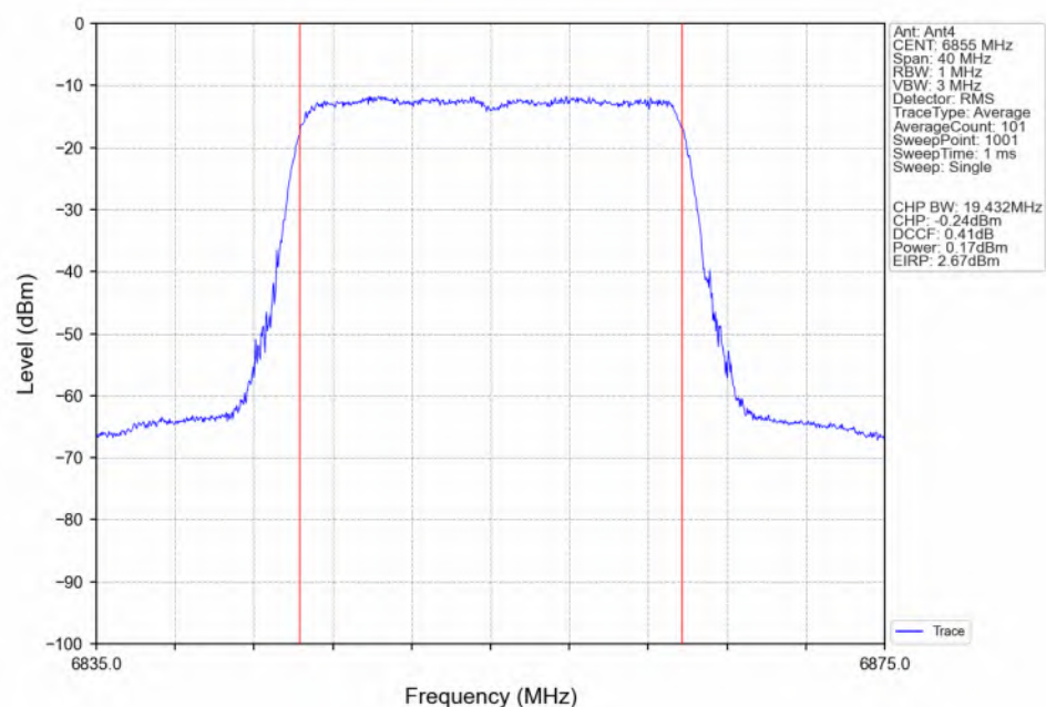
802.11ax(HEW20)_HCH_6855MHz_SU_ / Ant4_NTNV
