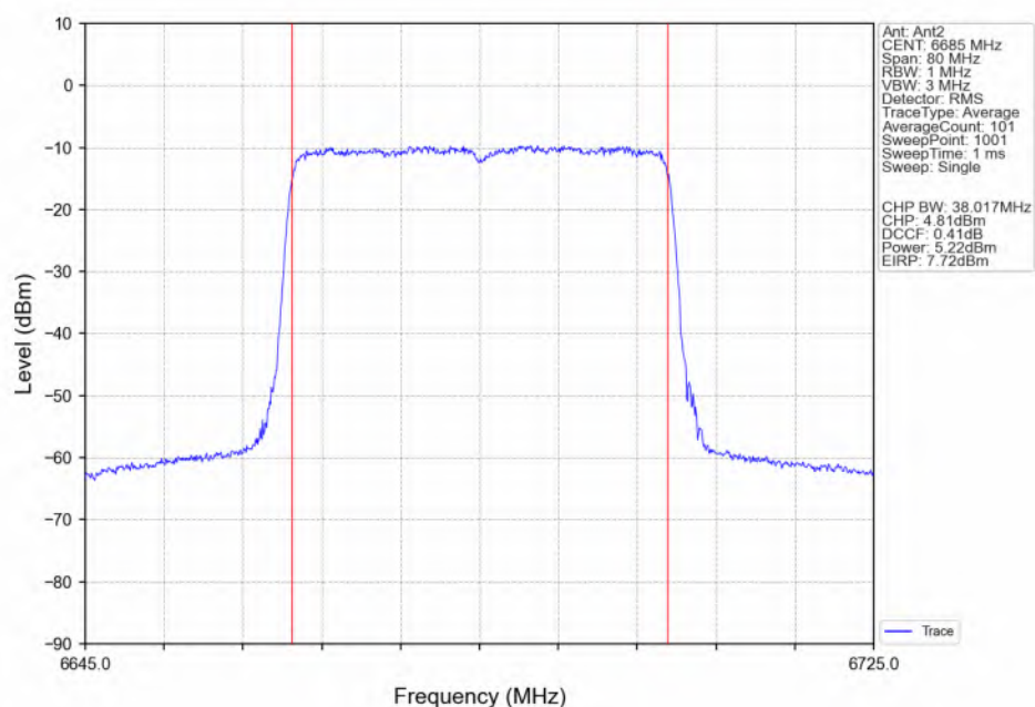
802.11ax(HEW40)_MCH_6685MHz_SU_ / Ant2_NTNV
