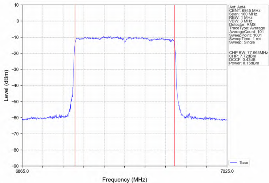
802.11ax(HEW80)_LCH_6945MHz_SU_ / Ant4_NTNV
