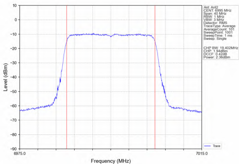
802.11ax(HEW20)_MCH_6995MHz_SU_ / Ant2_NTNV
