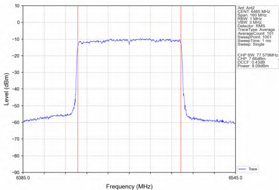
802.11ax(HEW80)_LCH_6465MHz_SU_ / Ant2_NTNV
