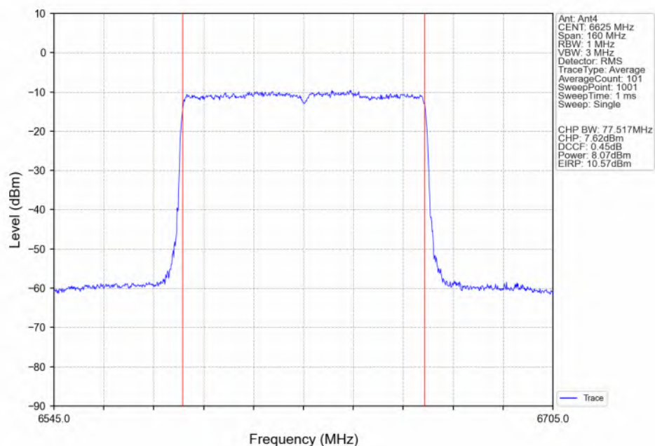
802.11ax(HEW80)_LCH_6625MHz_SU_ / Ant4_NTNV
