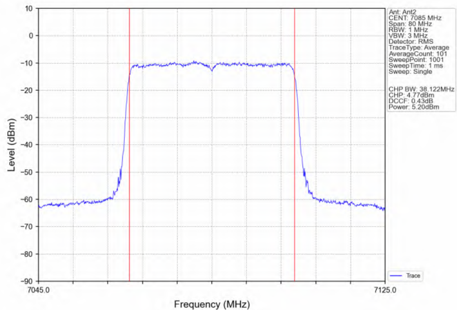
802.11ax(HEW40)_HCH_7085MHz_SU_ / Ant2_NTNV
