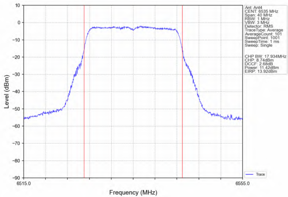
802.11a_LCH_6535MHz_Ant4_NTNV
