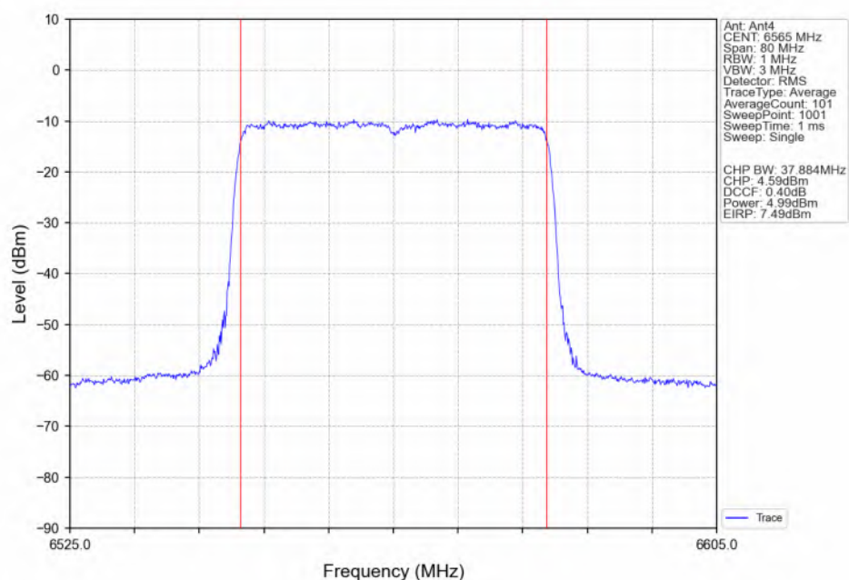
802.11ax(HEW40)_LCH_6565MHz_SU_ / Ant4_NTNV
