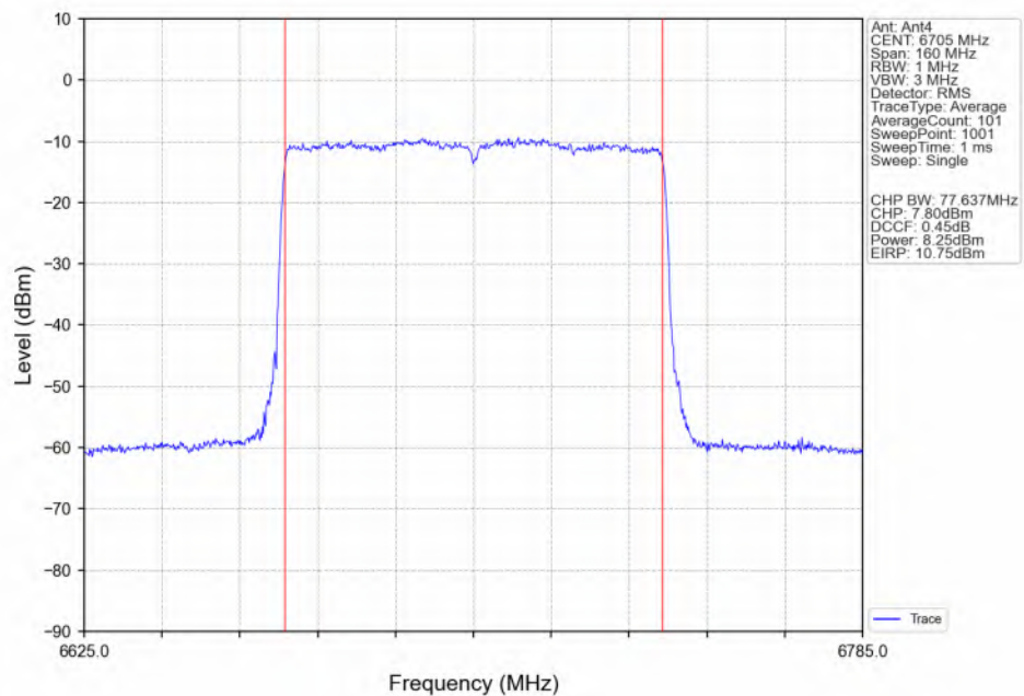
802.11ax(HEW80)_MCH_6705MHz_SU_ / Ant4_NTNV
