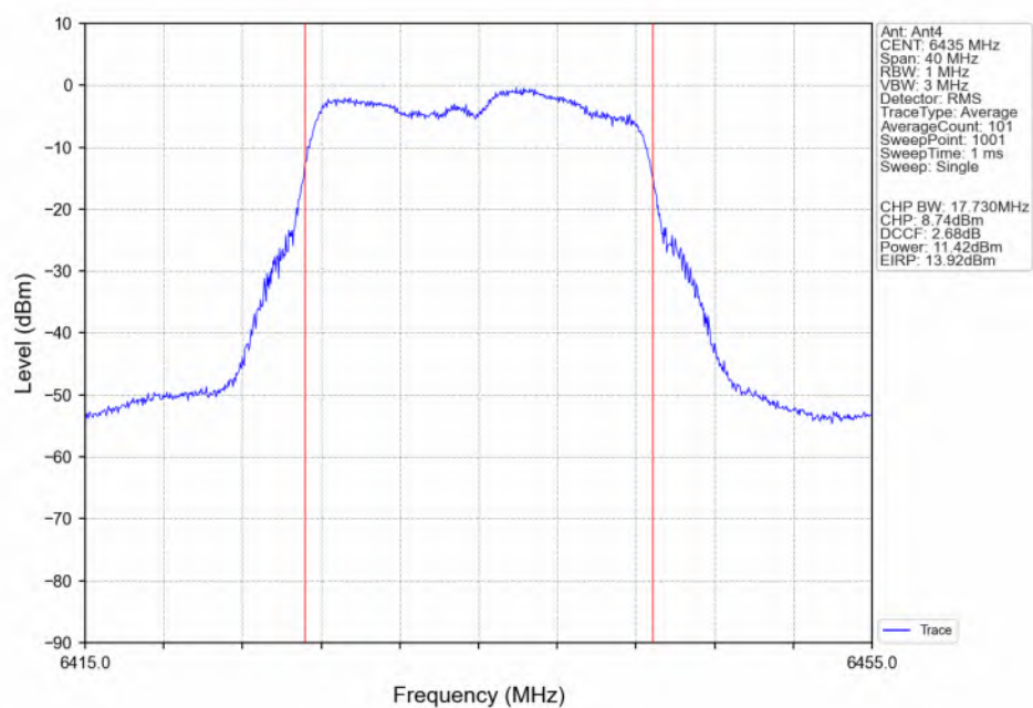
802.11a_LCH_6435MHz_Ant4_NTNV
