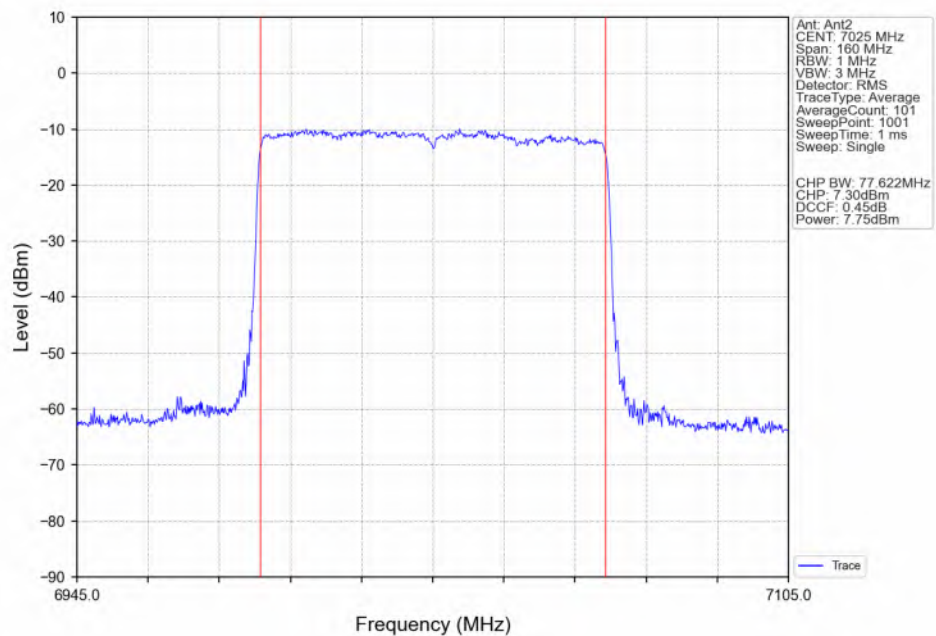
802.11ax(HEW80)_HCH_7025MHz_SU_ / Ant2_NTNV
