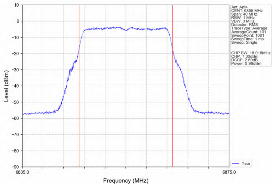
802.11a_HCH_6855MHz_Ant4_NTNV
