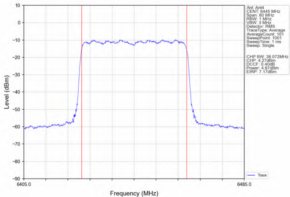
802.11ax(HEW40)_LCH_6445MHz_SU_ / Ant4_NTNV
