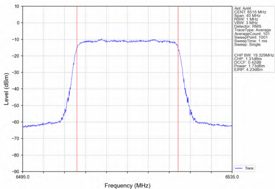
802.11ax(HEW20)_HCH_6515MHz_SU_ / Ant4_NTNV
