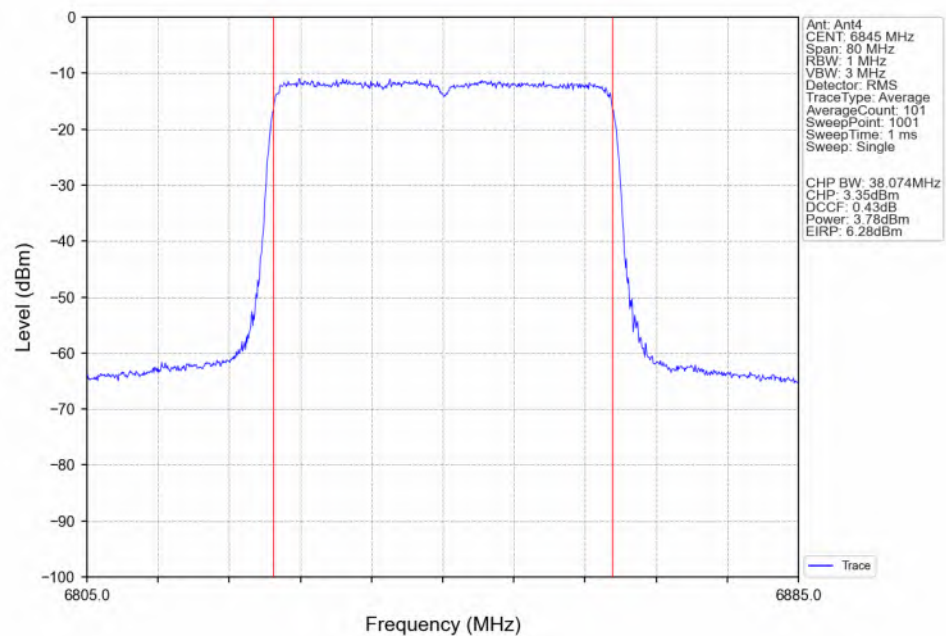
802.11ax(HEW40)_HCH_6845MHz_SU_ / Ant4_NTNV
