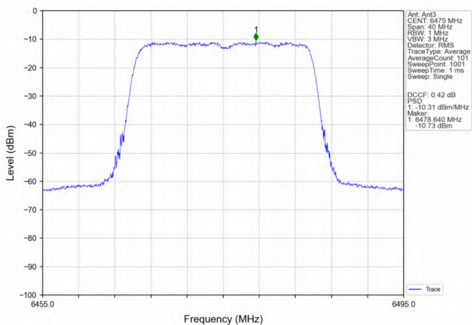
802.11ax(HEW20)_MCH_6475MHz_SU_ / Ant3_NTNV
