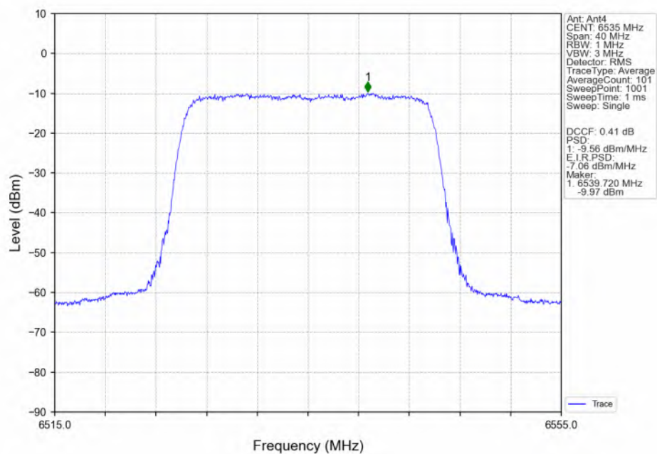
802.11ax(HEW20)_LCH_6535MHz_SU_ / Ant4_NTNV
