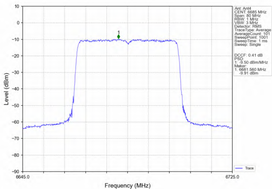
802.11ax(HEW40)_MCH_6685MHz_SU_ / Ant4_NTNV
