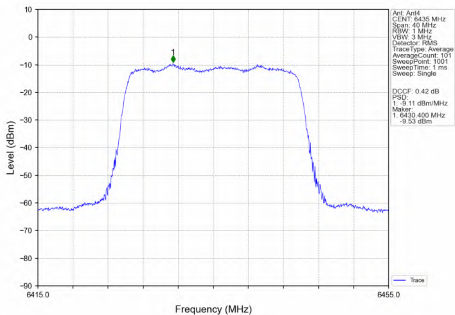
802.11ax(HEW20)_LCH_6435MHz_SU_ / Ant4_NTNV
