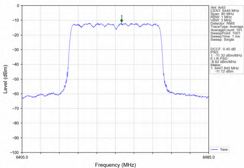
802.11ax(HEW40)_LCH_6445MHz_SU_ / Ant3_NTNV
