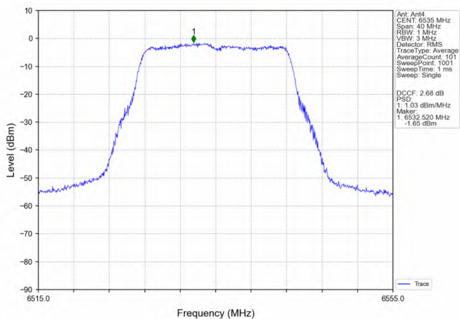
802.11a_LCH_6535MHz_Ant4_NTNV
