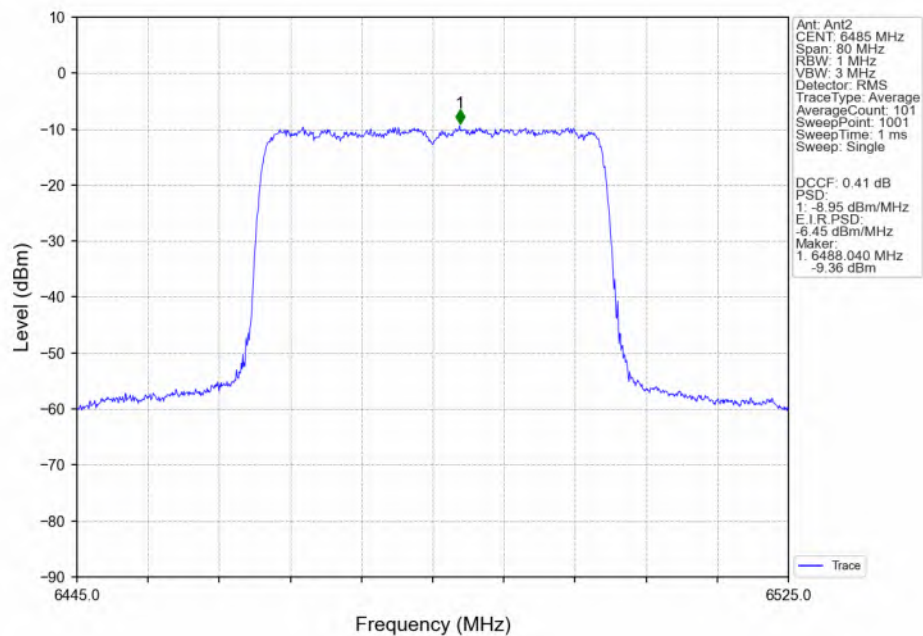
802.11ax(HEW40)_MCH_6485MHz_SU_ / Ant2_NTNV
