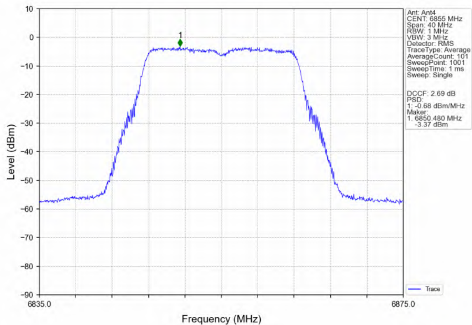
802.11a_HCH_6855MHz_Ant4_NTNV
