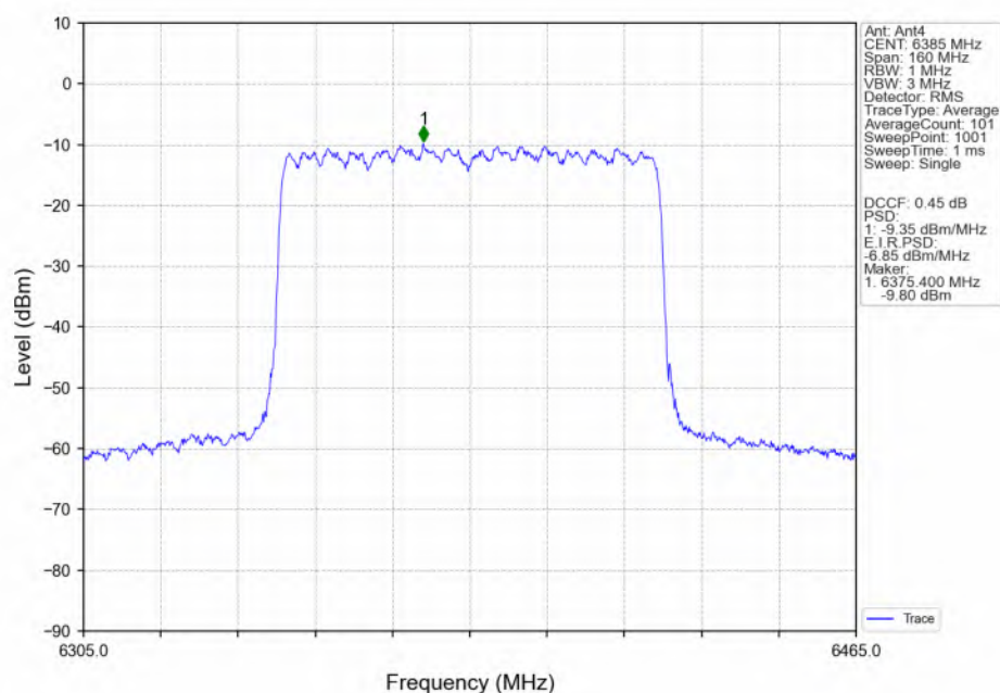
802.11ax(HEW80)_HCH_6385MHz_SU_ / Ant4_NTNV
