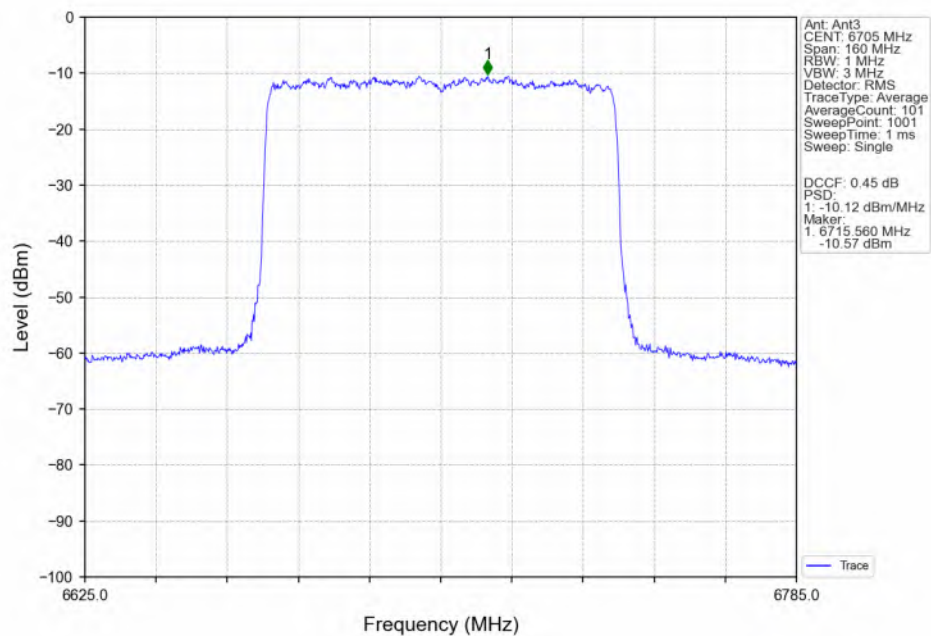
802.11ax(HEW80)_MCH_6705MHz_SU / Ant3_NTNV
