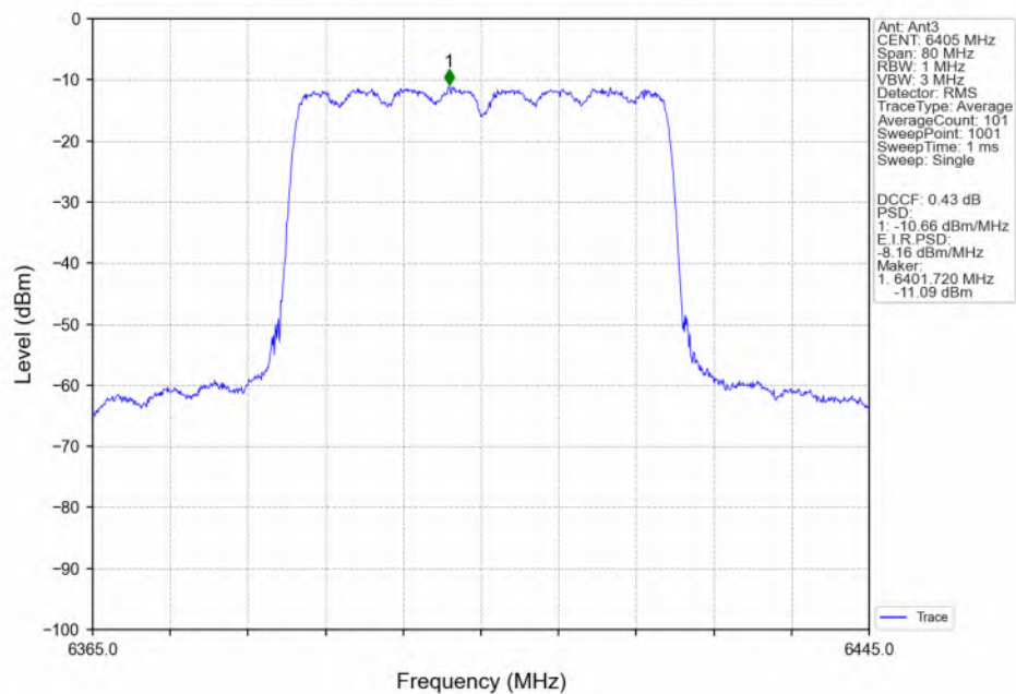
802.11ax(HEW40)_HCH_6405MHz_SU / Ant3_NTNV
