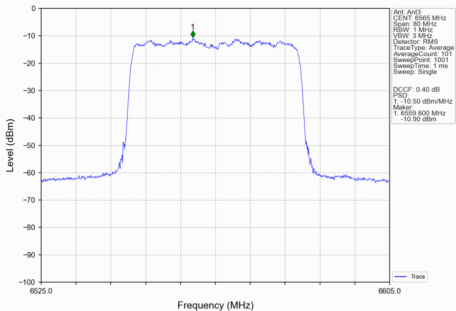
802.11ax(HEW40)_LCH_6565MHz_SU_ / Ant3_NTNV
