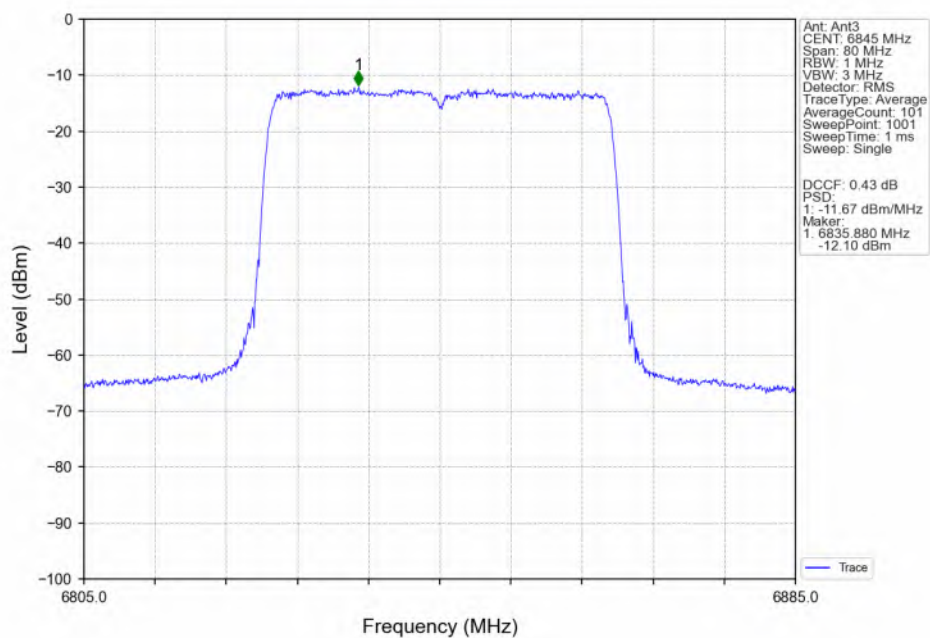
802.11ax(HEW40)_HCH_6845MHz_SU_ / Ant3_NTNV
