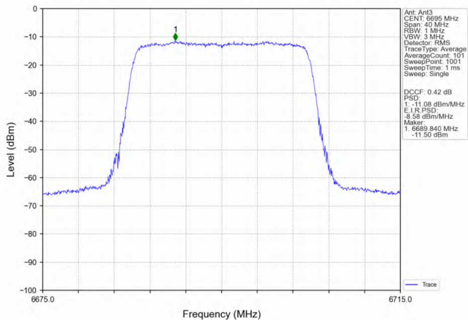
802.11ax(HEW20)_MCH_6695MHz_SU_ / Ant3_NTNV
