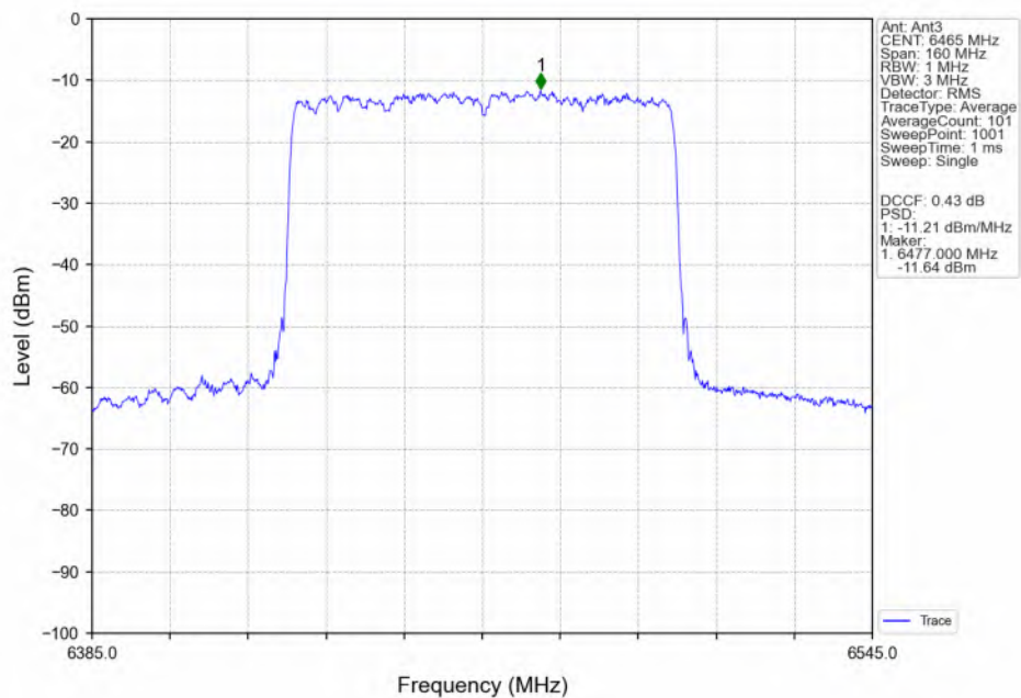
802.11ax(HEW80)_LCH_6465MHz_SU_ / Ant3_NTNV
