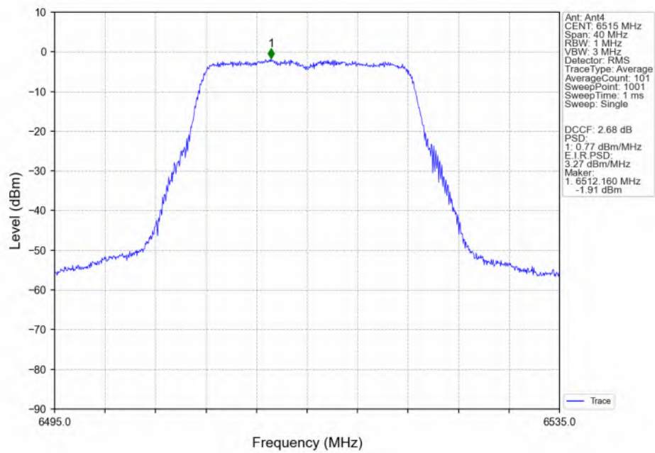
802.11a_HCH_6515MHz_Ant4_NTNV
