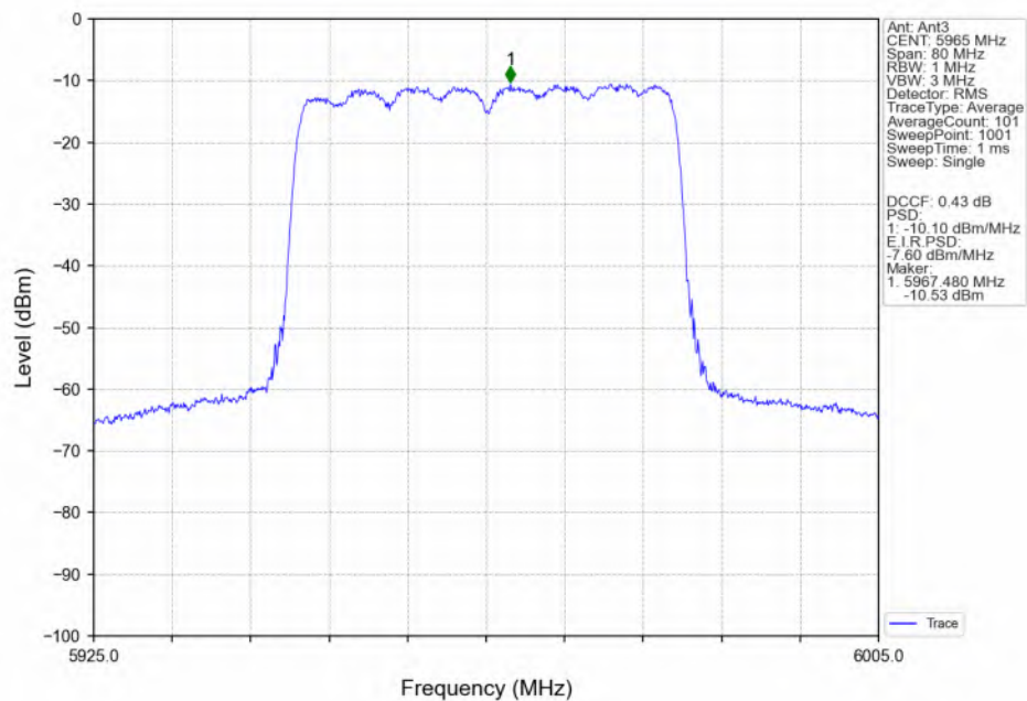
802.11ax(HEW40)_LCH_5965MHz_SU_ / Ant3_NTNV
