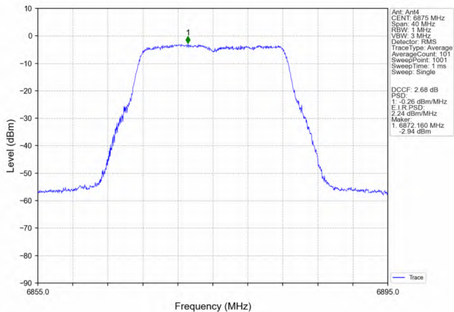
802.11a_HCH_6875MHz_Ant4_NTNV
