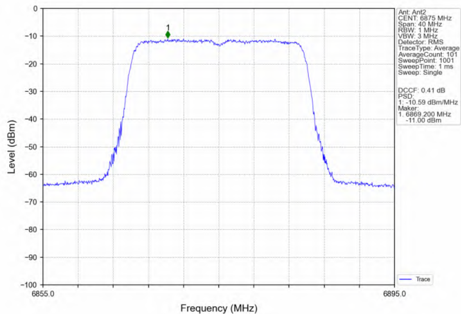
802.11ax(HEW20)_HCH_6875MHz_SU_ / Ant2_NTNV
