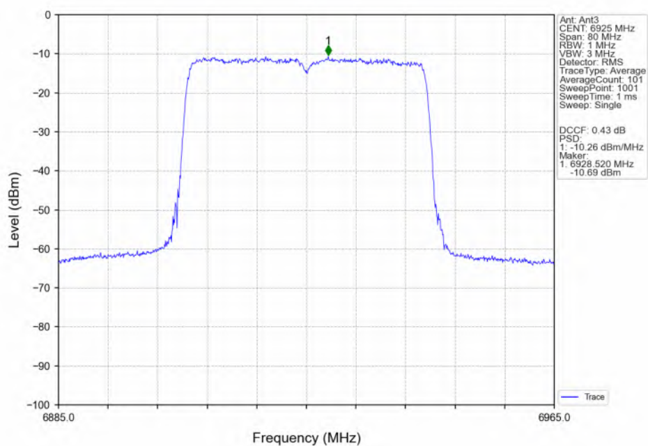
802.11ax(HEW40)_LCH_6925MHz_SU_ / Ant3_NTNV
