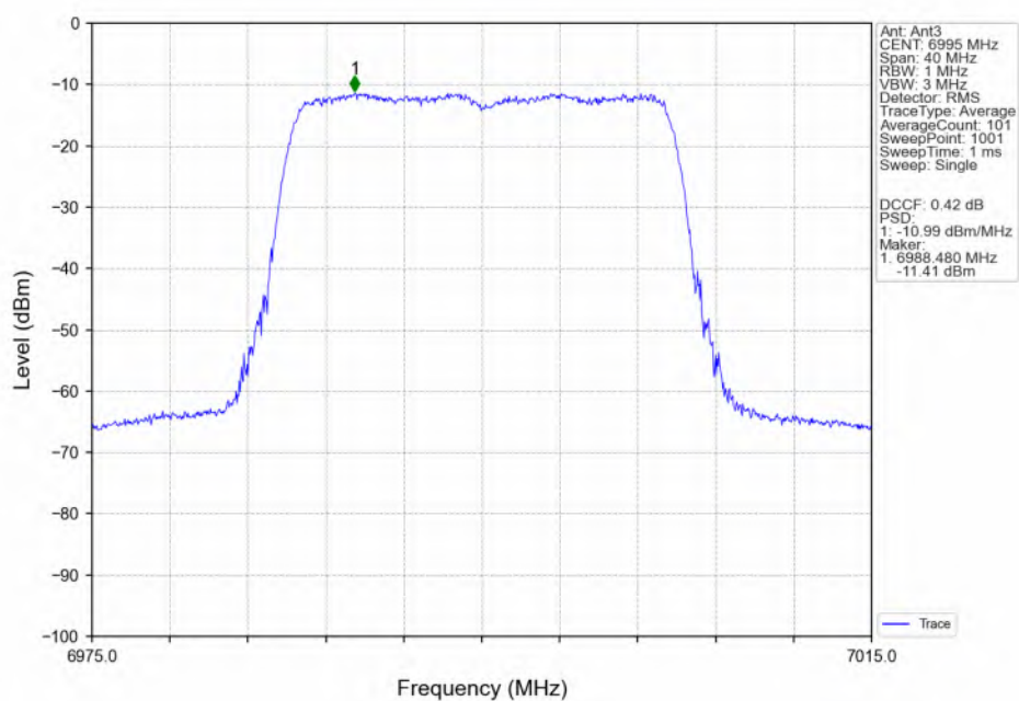
802.11ax(HEW20)_MCH_6995MHz_SU_ / Ant3_NTNV
