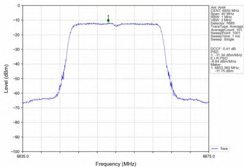
802.11ax(HEW20)_HCH_6855MHz_SU_ / Ant4_NTNV
