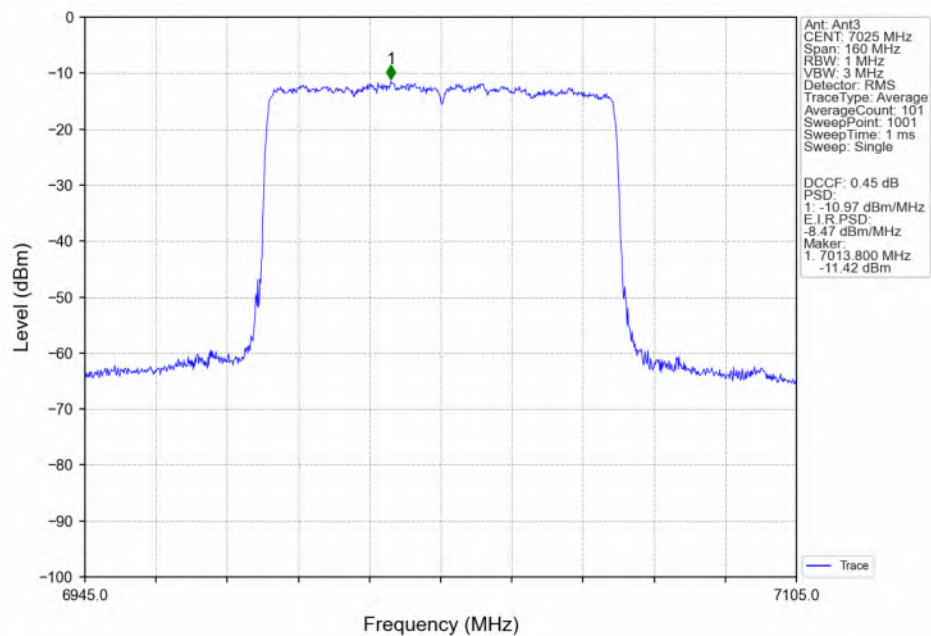
802.11ax(HEW80)_HCH_7025MHz_SU_ / Ant3_NTNV
