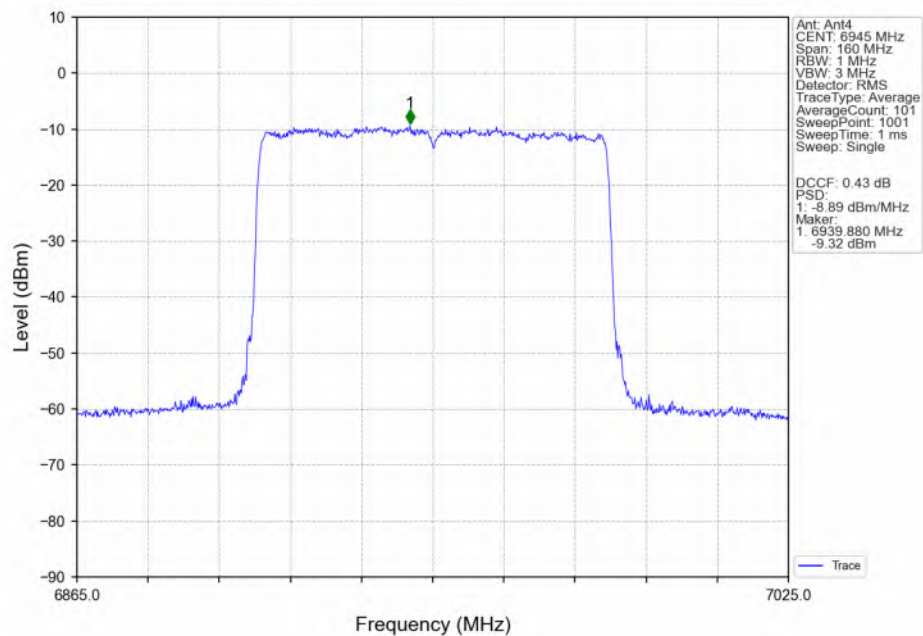
802.11ax(HEW80)_LCH_6945MHz_SU_ / Ant4_NTNV
