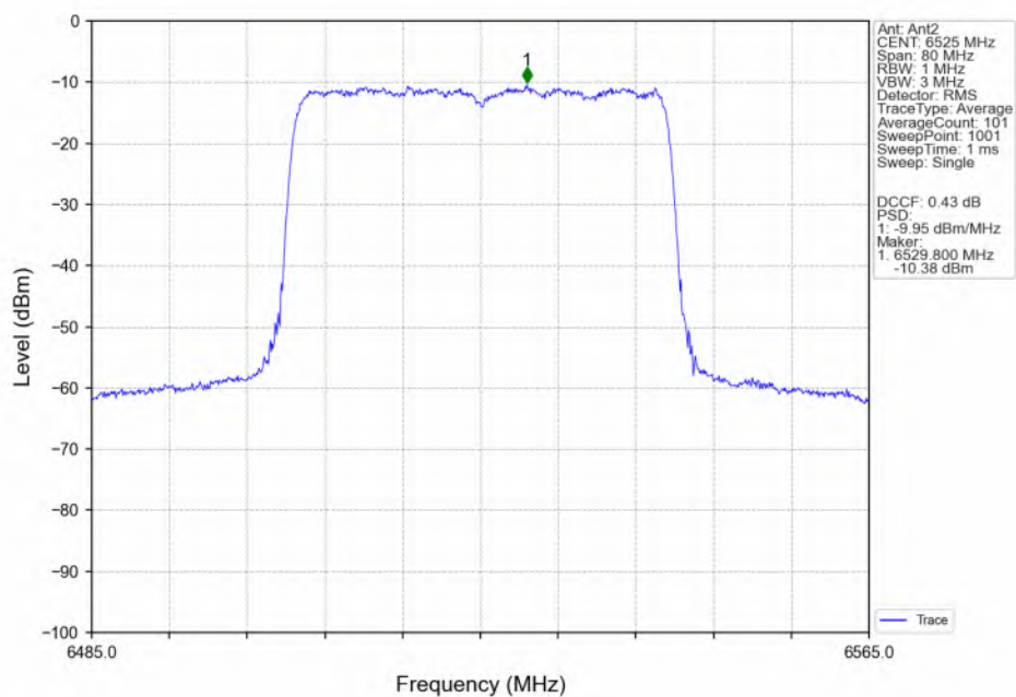
802.11ax(HEW40)_HCH_6525MHz_SU_/_Ant2_NTNV
