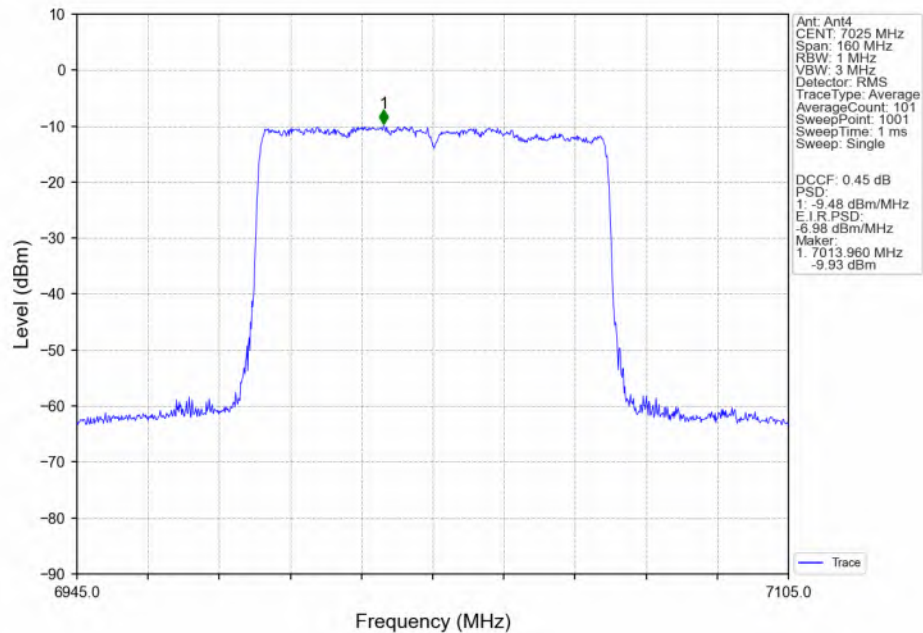
802.11ax(HEW80)_HCH_7025MHz_SU_ / MIMO_NTNV
