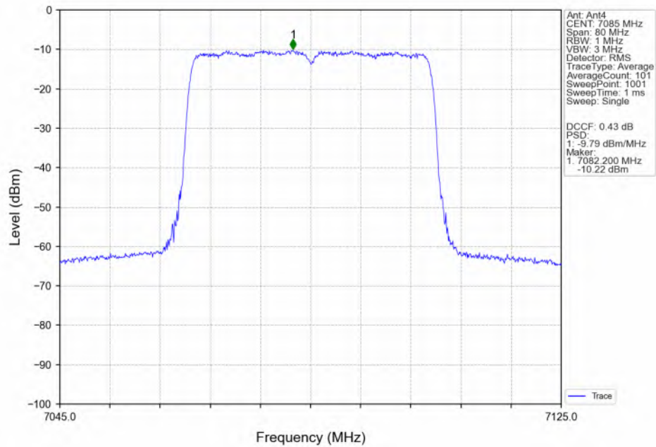
802.11ax(HEW40)_HCH_7085MHz_SU_ / MIMO_NTNV
