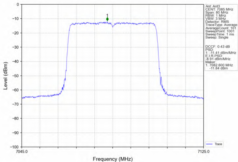
802.11ax(HEW40)_HCH_7085MHz_SU / Ant3_NTNV
