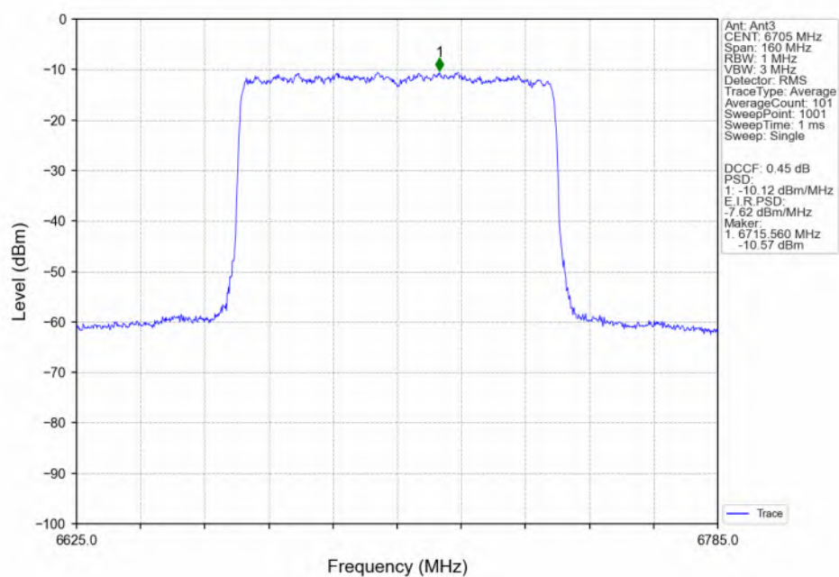
802.11ax(HEW80)_MCH_6705MHz_SU / Ant3_NTNV
