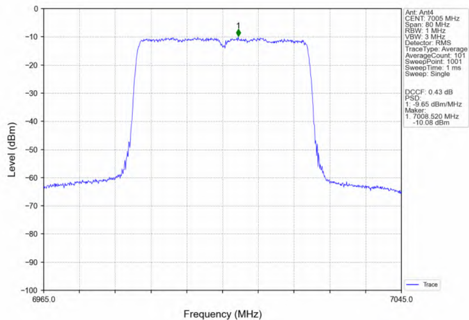
802.11ax(HEW40)_MCH_7005MHz_SU_ / Ant4_NTNV
