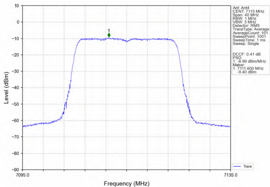
802.11ax(HEW20)_HCH_7115MHz_SU_ / Ant4_NTNV
