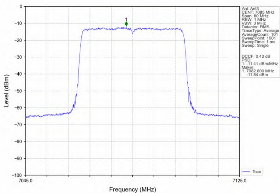
802.11ax(HEW40)_HCH_7085MHz_SU_ / Ant3_NTNV
