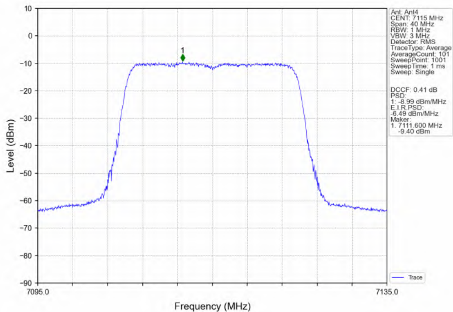
802.11ax(HEW20)_HCH_7115MHz_SU_ / Ant4_NTNV
