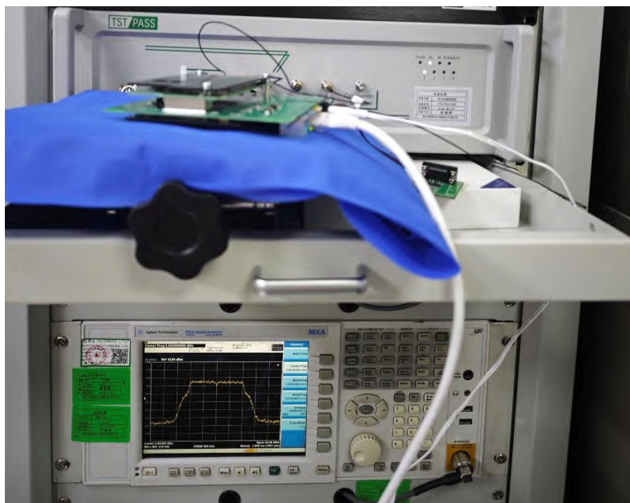
Photograph 4: Set-up photo for RC Conducted Emission
