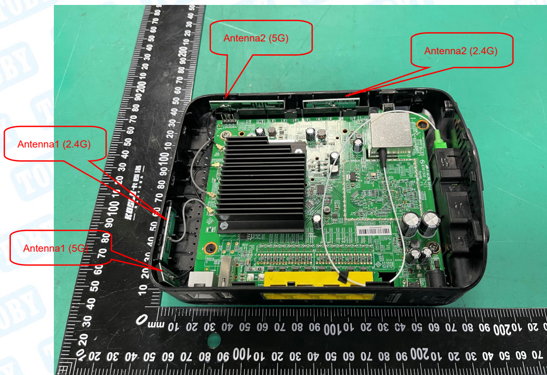
Photo 9 Internal of EUT
