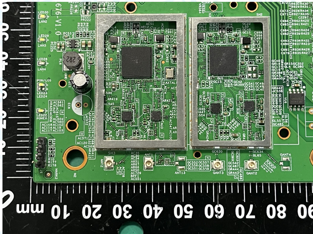
Photo 14 Appearance of PCB
