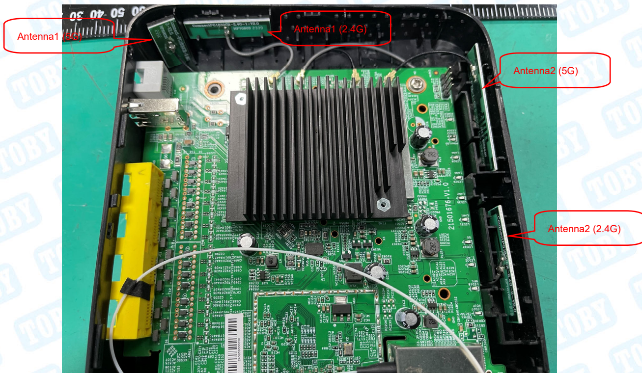
Photo 9 Internal of EUT
