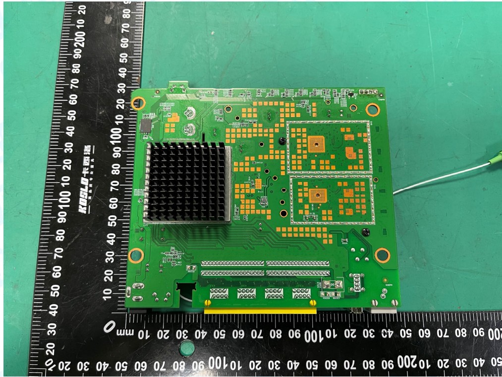
Photo 11 Appearance of PCB
