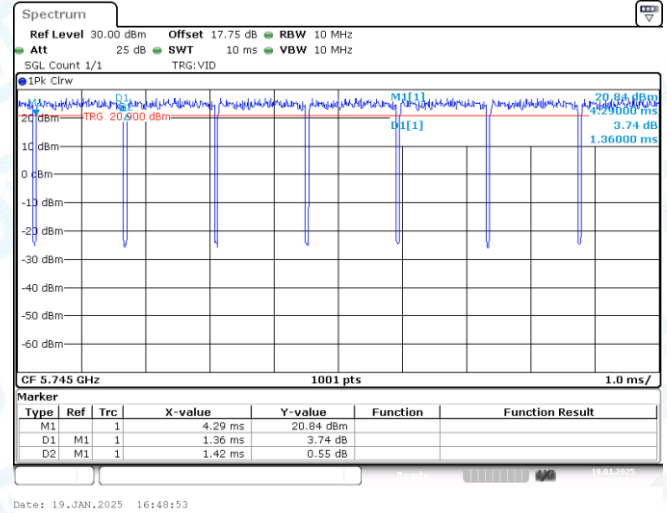
NTVN-11A-CDD-Ant2-5745
