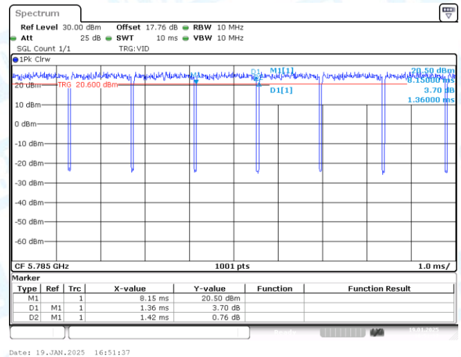
NTVN-11A-CDD-Ant2-5785
