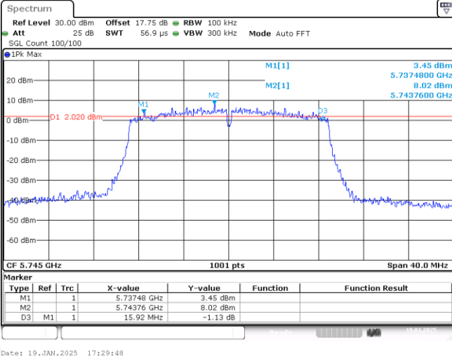
11AC20-CDD-Ant1-5745-PASS
