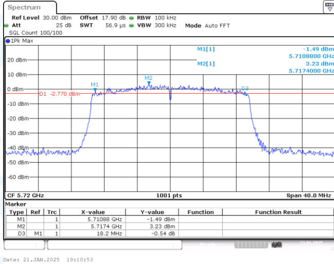
11AX20-CDD-Ant1-5720
