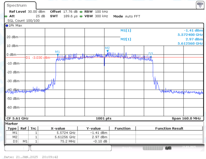
11AX80-CDD-Ant2-5610-PASS
