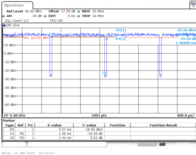
NTNV-11A-CDD-Ant1-5580
