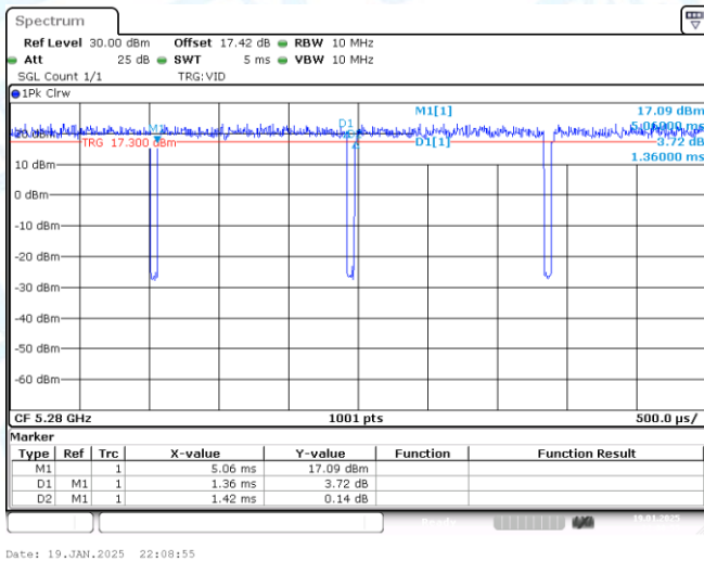
NTNV-11A-CDD-Ant1-5280
