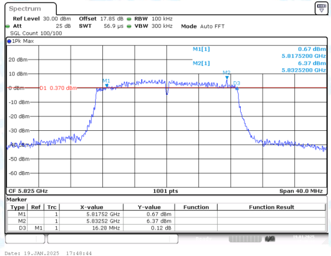
11AC20-CDD-Ant2-5825-PASS
