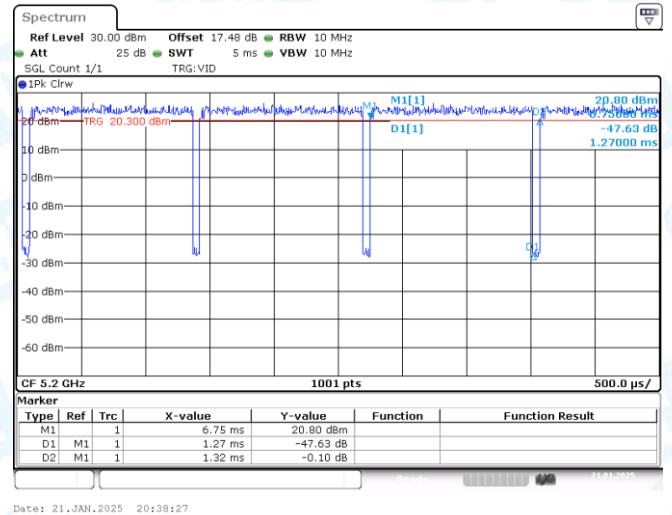
NTNV-11N20-CDD-Ant2-5200
