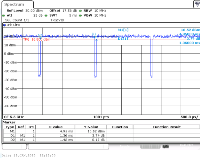
NTNV-11A-CDD-Ant1-5500
