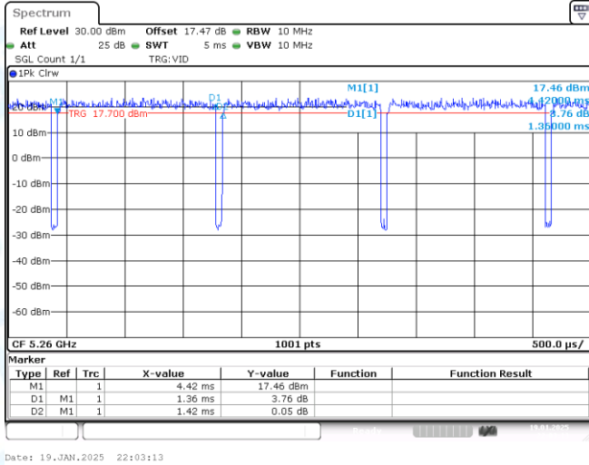
NTNV-11A-CDD-Ant1-5260
