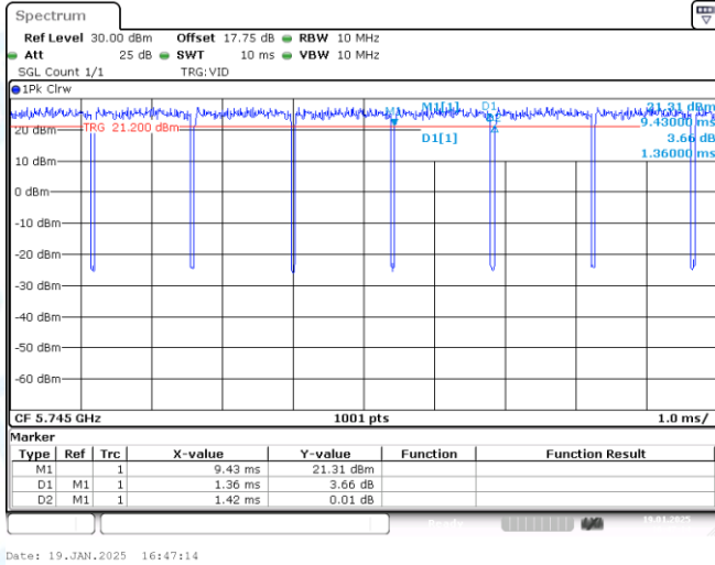
NTVN-11A-CDD-Ant1-5745
