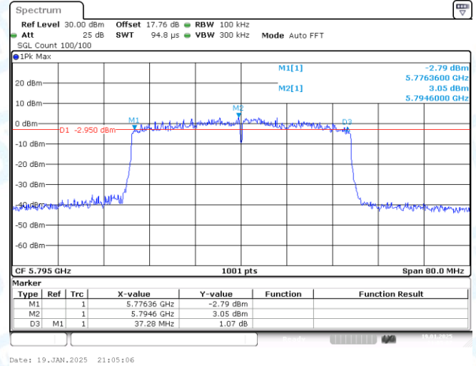
11AX40-CDD-Ant2-5795-PASS
