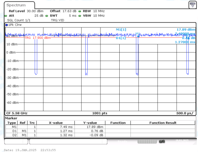
NTNV-11N20-CDD-Ant2-5580
