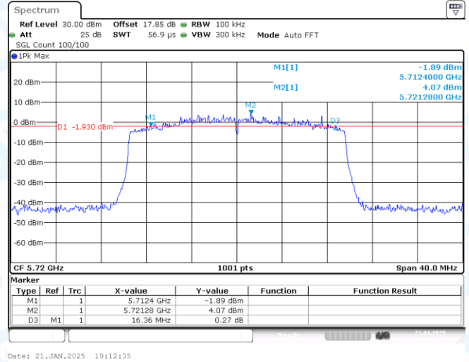
11AX20-CDD-Ant2-5720
