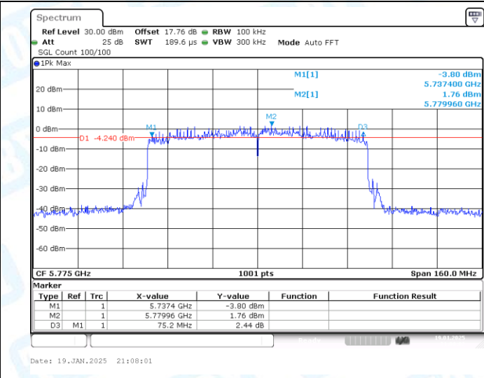
11AX80-CDD-Ant2-5775-PASS
