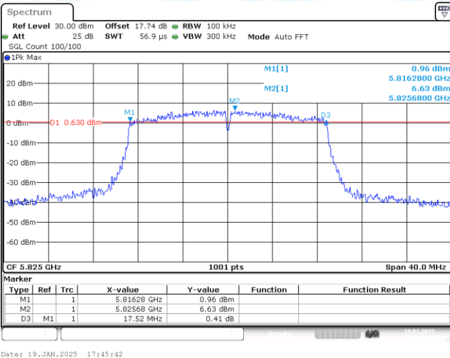
11AC20-CDD-Ant1-5825-PASS
