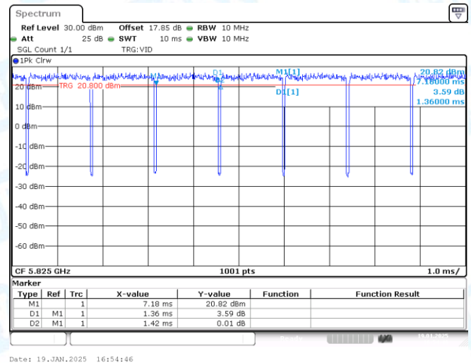
NTVN-11A-CDD-Ant2-5825
