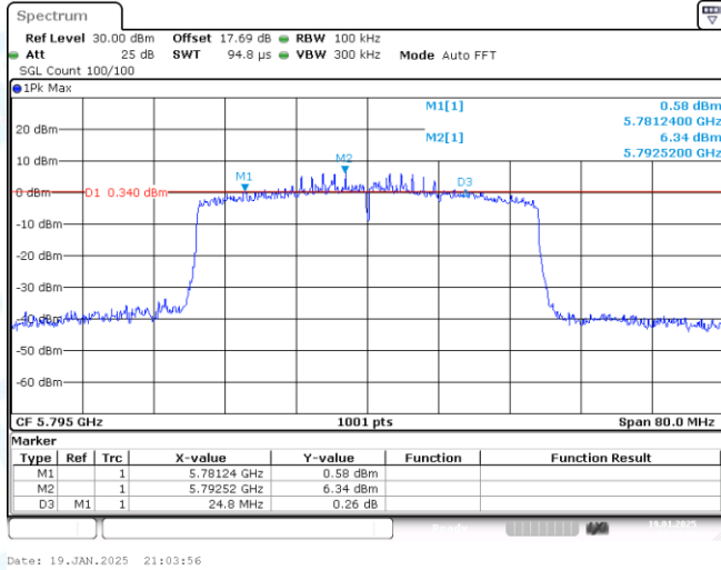
11AX40-CDD-Ant1-5795-PASS
