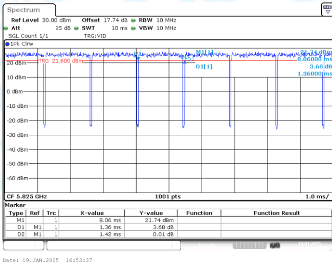
NTVN-11A-CDD-Ant1-5825
