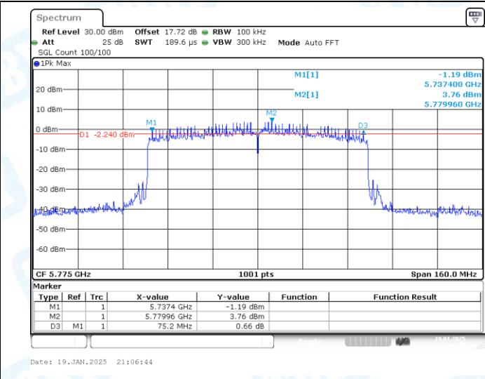
11AX80-CDD-Ant1-5775-PASS
