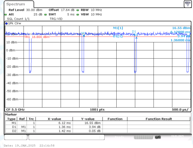
NTNV-11A-CDD-Ant2-5500
