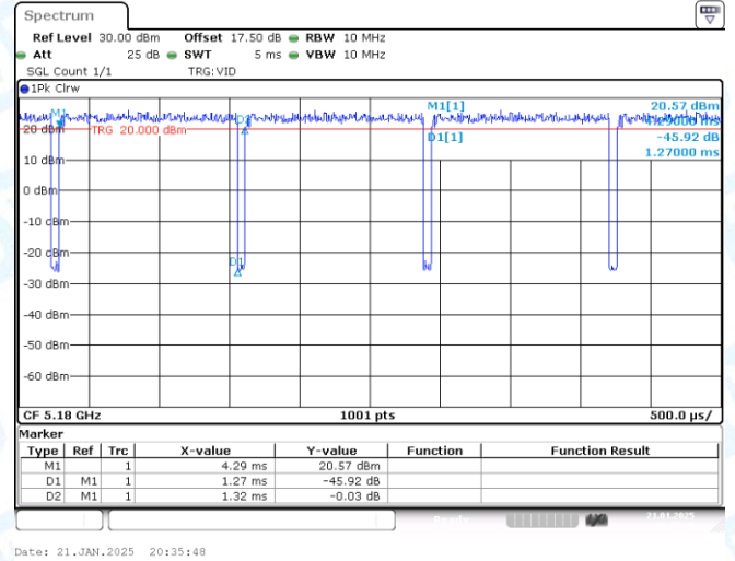
NTNV-11N20-CDD-Ant2-5180
