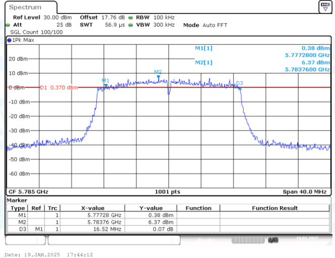
11AC20-CDD-Ant2-5785-PASS
