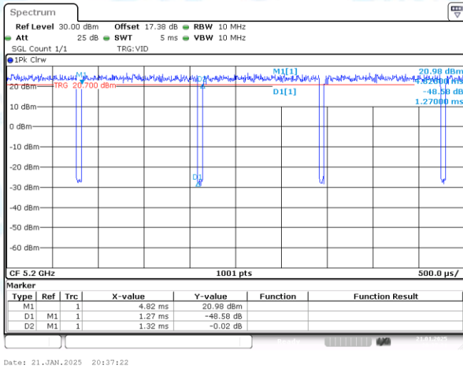
NTNV-11N20-CDD-Ant1-5200
