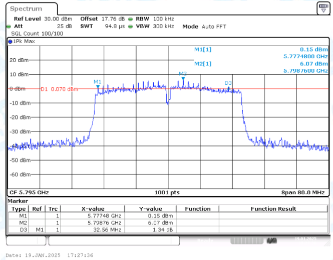
11N40-CDD-Ant2-5795-PASS
