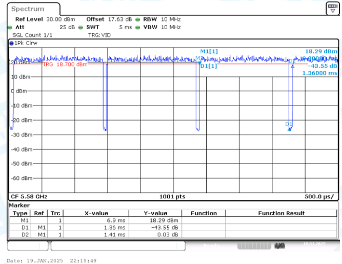
NTNV-11A-CDD-Ant2-5580
