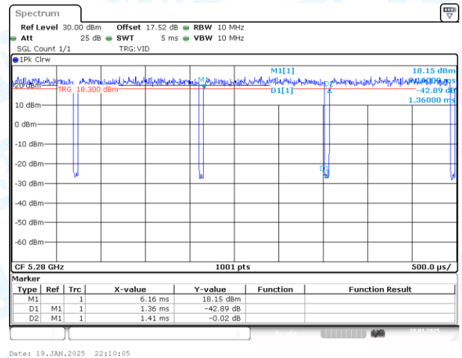
NTNV-11A-CDD-Ant2-5280
