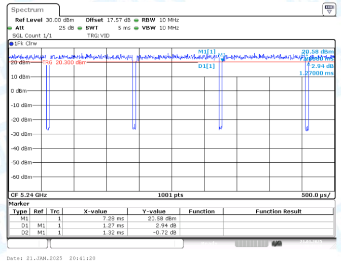
NTNV-11N20-CDD-Ant2-5240
