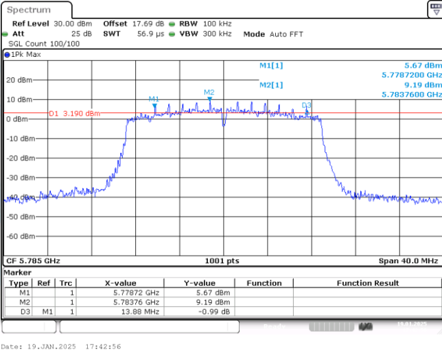
11AC20-CDD-Ant1-5785-PASS
