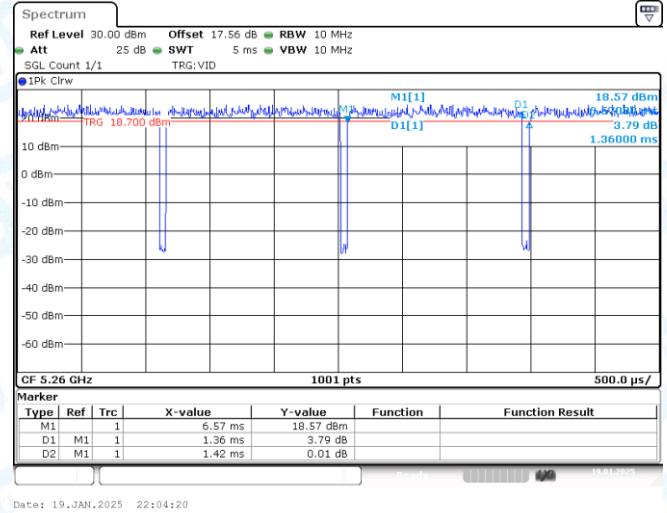
NTNV-11A-CDD-Ant2-5260
