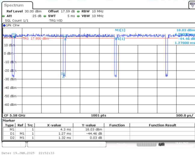
NTNV-11N20-CDD-Ant1-5580
