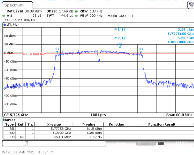
11N40-CDD-Ant1-5795-PASS
