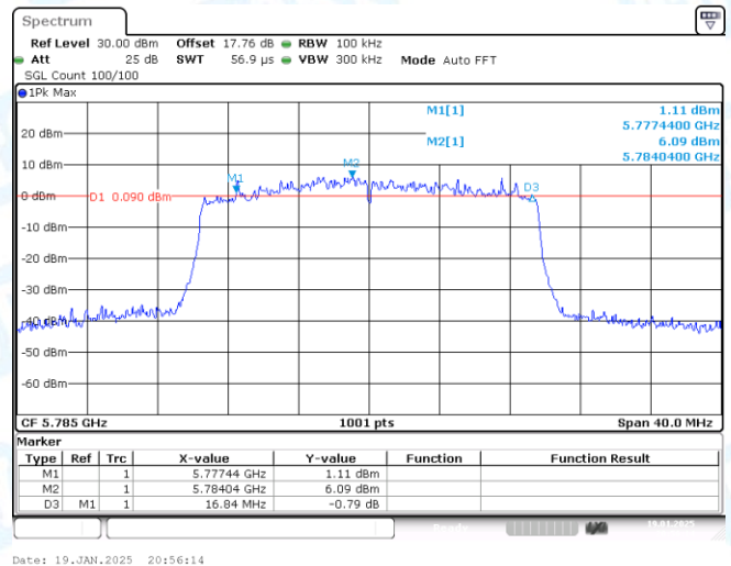
11AX20-CDD-Ant2-5785-PASS
