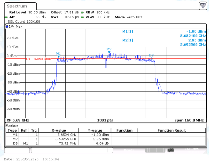
11AX80-CDD-Ant2-5690
