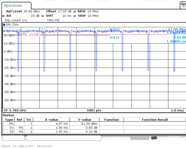
NTVN-11A-CDD-Ant1-5785
