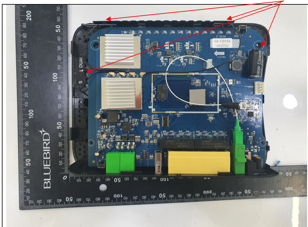
PCB Antenna
