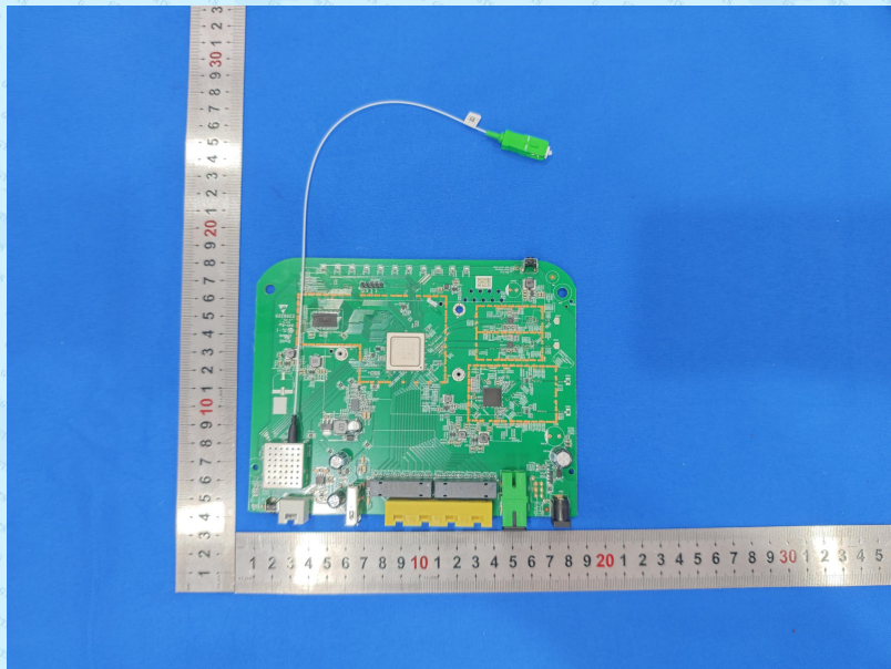
PCB
