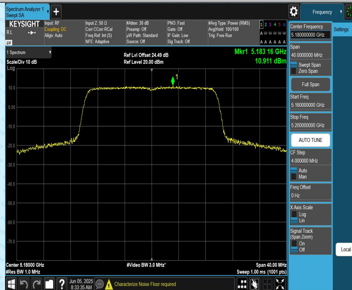
11AX20CDD_Ant2_5180
