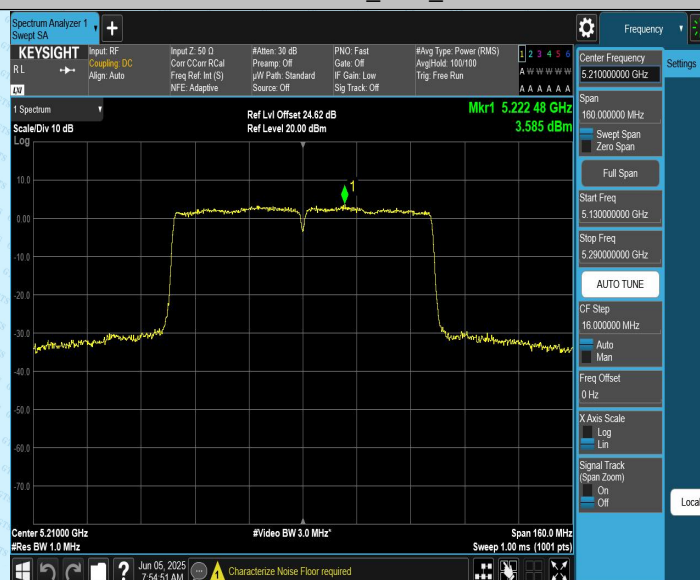
11AC80CDD_Ant2_5210
