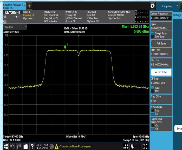
11AC40CDD_Ant2_5670
