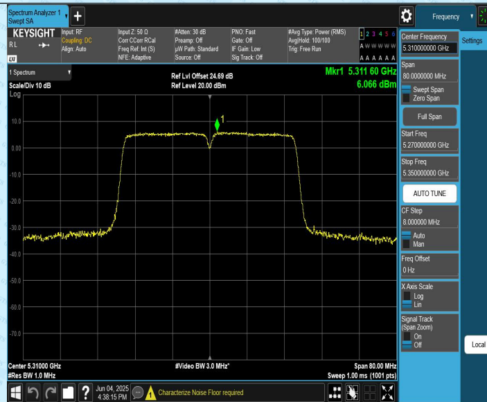
11AC40CDD_Ant2_5310
