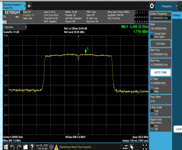
11AC80CDD_Ant2_5290
