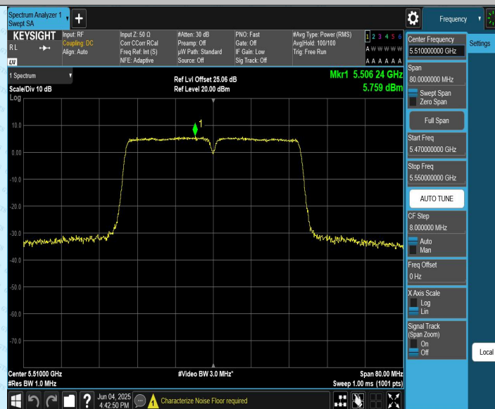
11AC40CDD_Ant2_5510
