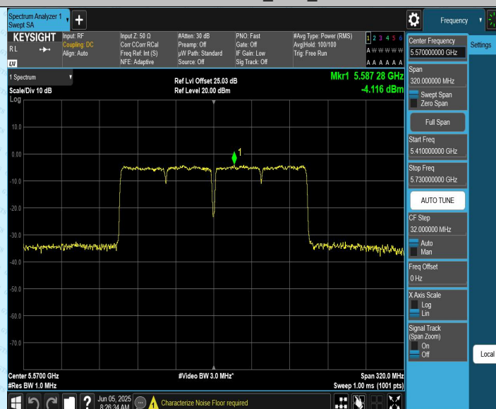
11AC160CDD_Ant2_5570
