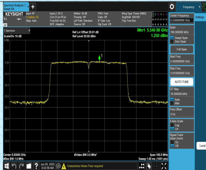
11AC80CDD_Ant2_5530
