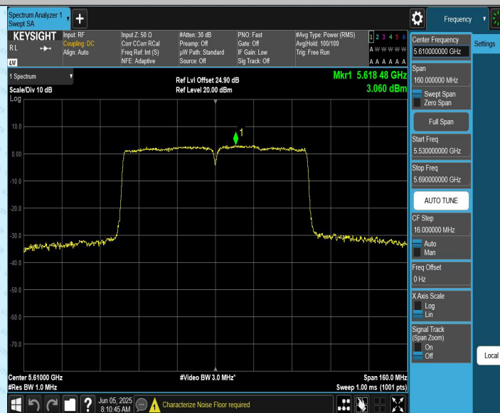
11AC80CDD_Ant2_5610
