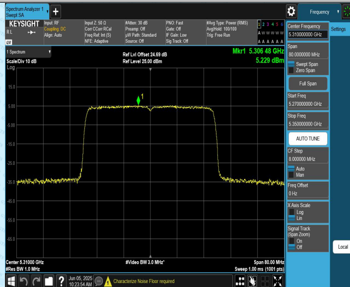
11AX40CDD_Ant2_5310
