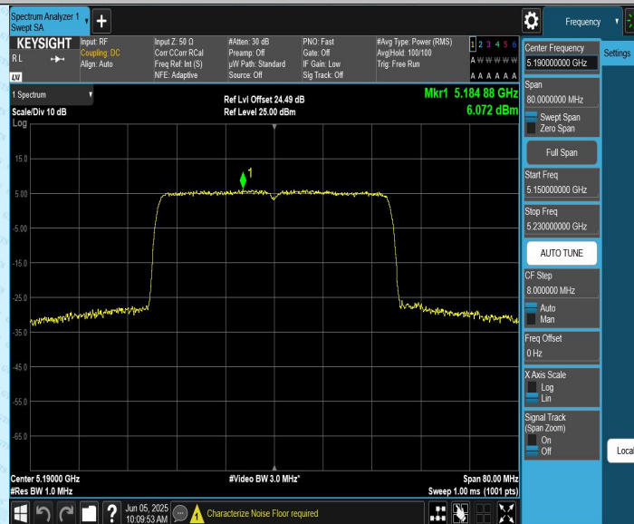
11AX40CDD_Ant2_5190
