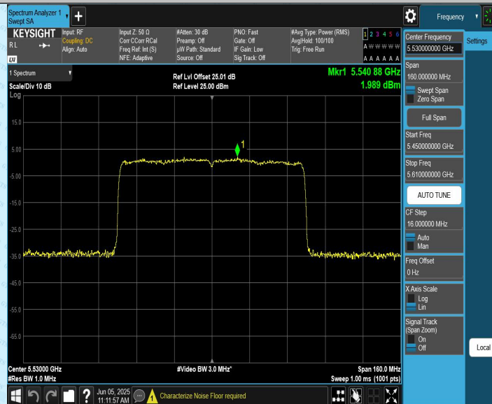
11AX80CDD_Ant2_5530
