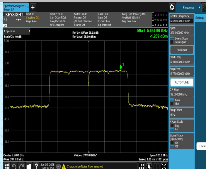
11AX160CDD_Ant2_5570
