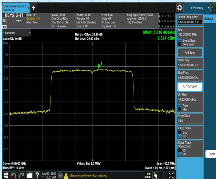
11AX80CDD_Ant2_5610
