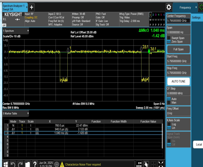
11AC40CDD_Ant2_5795
