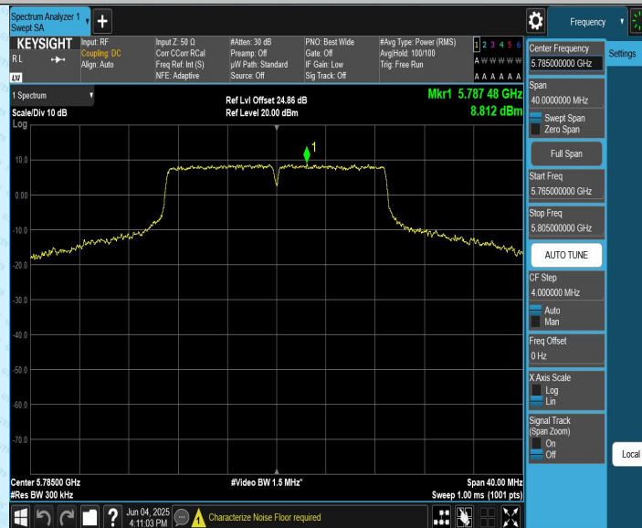
11AC20CDD_Ant2_5785
