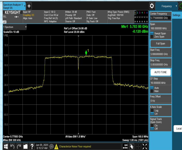
11AC80CDD_Ant2_5775
