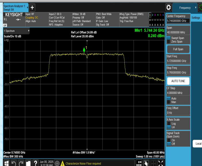
11AX20CDD_Ant2_5745
