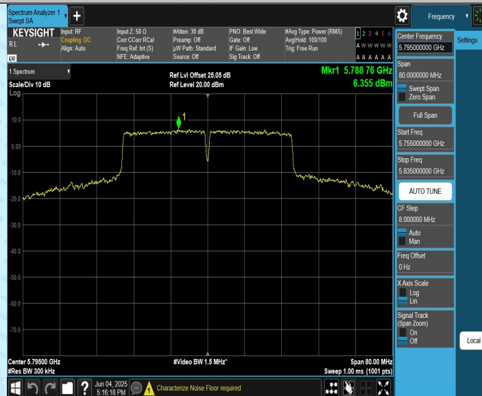
11AC40CDD_Ant2_5795
