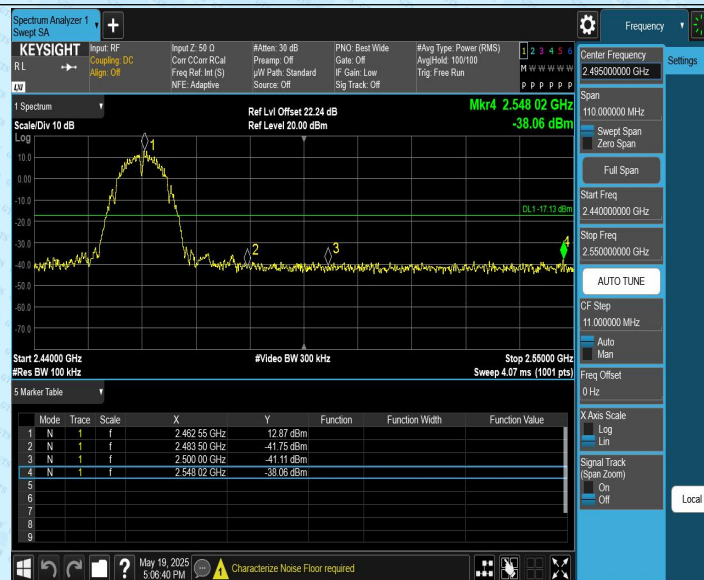
11B-CDD_Ant2_High_2462
