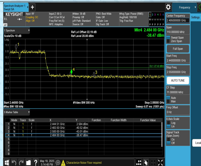
11N40CDD_Ant2_High_2452
