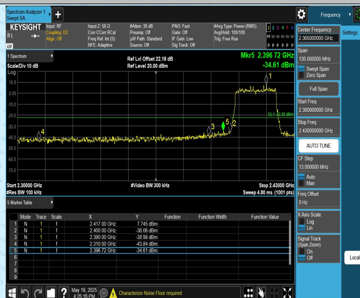
11AX20CDD_Ant2_Low_2412
