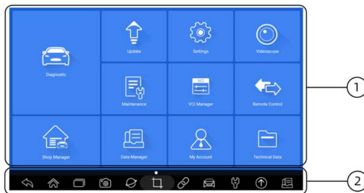
Figure 3-7 Sample Home Screen
