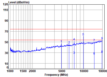
BT_DH5_TX_CH_78_Horizontal
