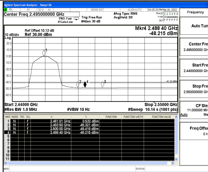
11G_Ant_High_2462_Peak
