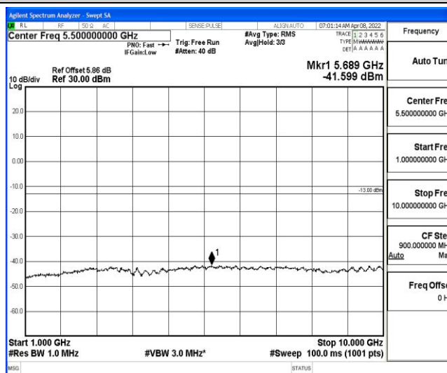
Band14-10MHz-QPSK-23330-1RB#0-Range4:1000~10000MHz
