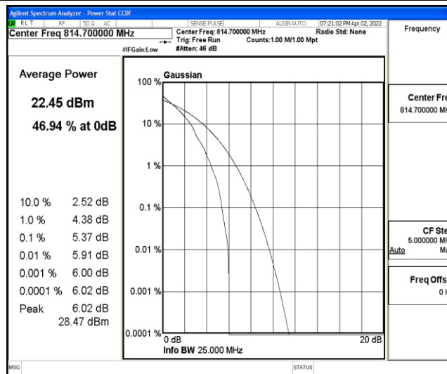
Band26-1.4MHz-QPSK-26697-6RB#0
