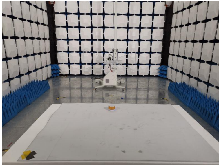
Below 1GHz for radiated emission test setup
