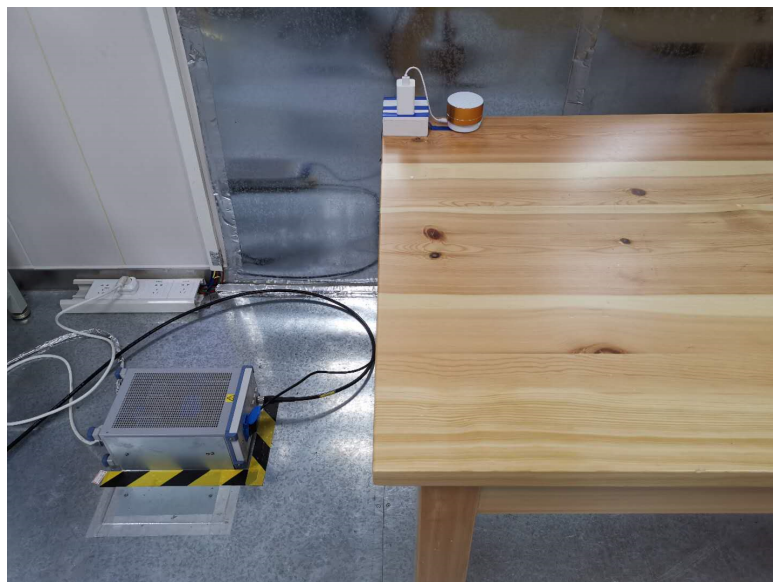
conducted emission test setup
