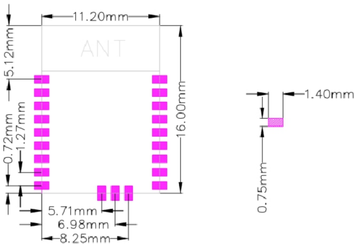
4-5 Reference packaging size
