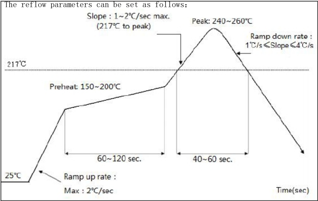
Figure 5-1 Recommended reflow curv
