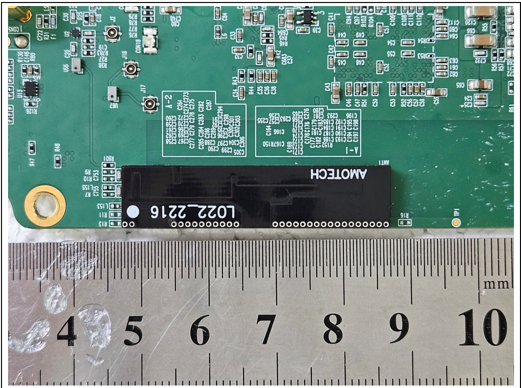
< Antenna 1 >
