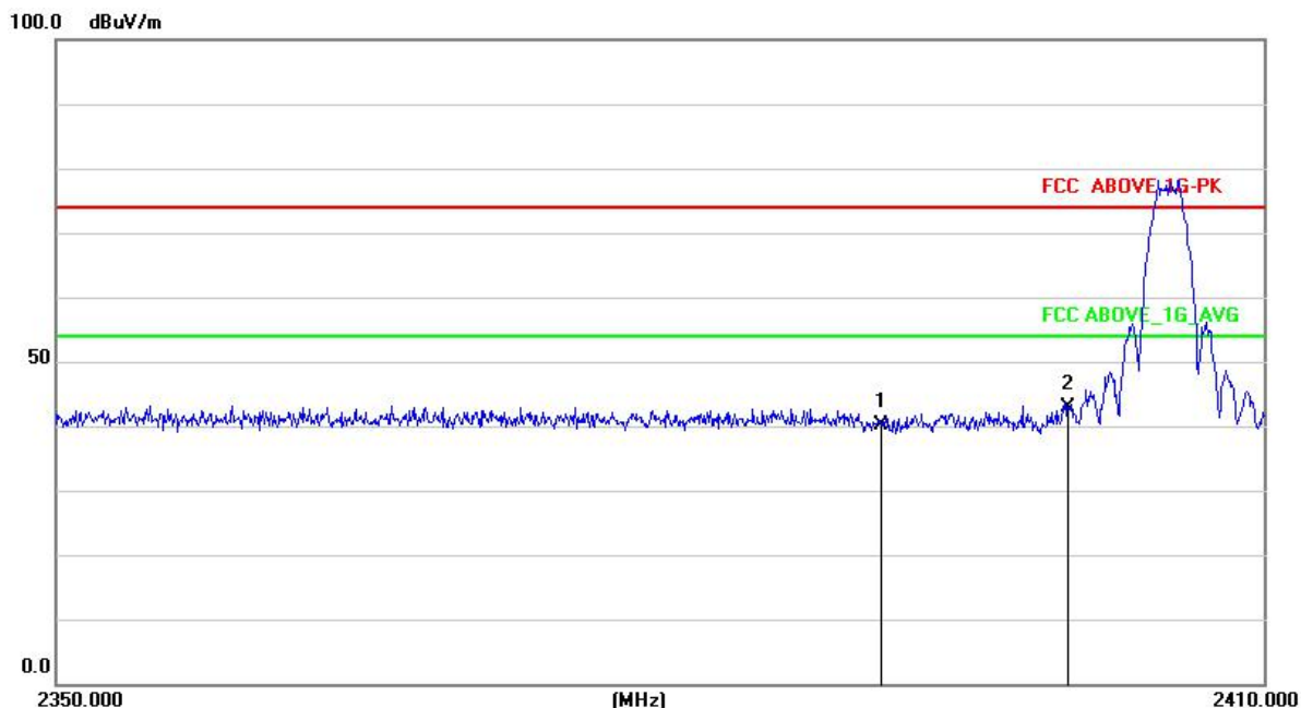
2402MHz Vertical
