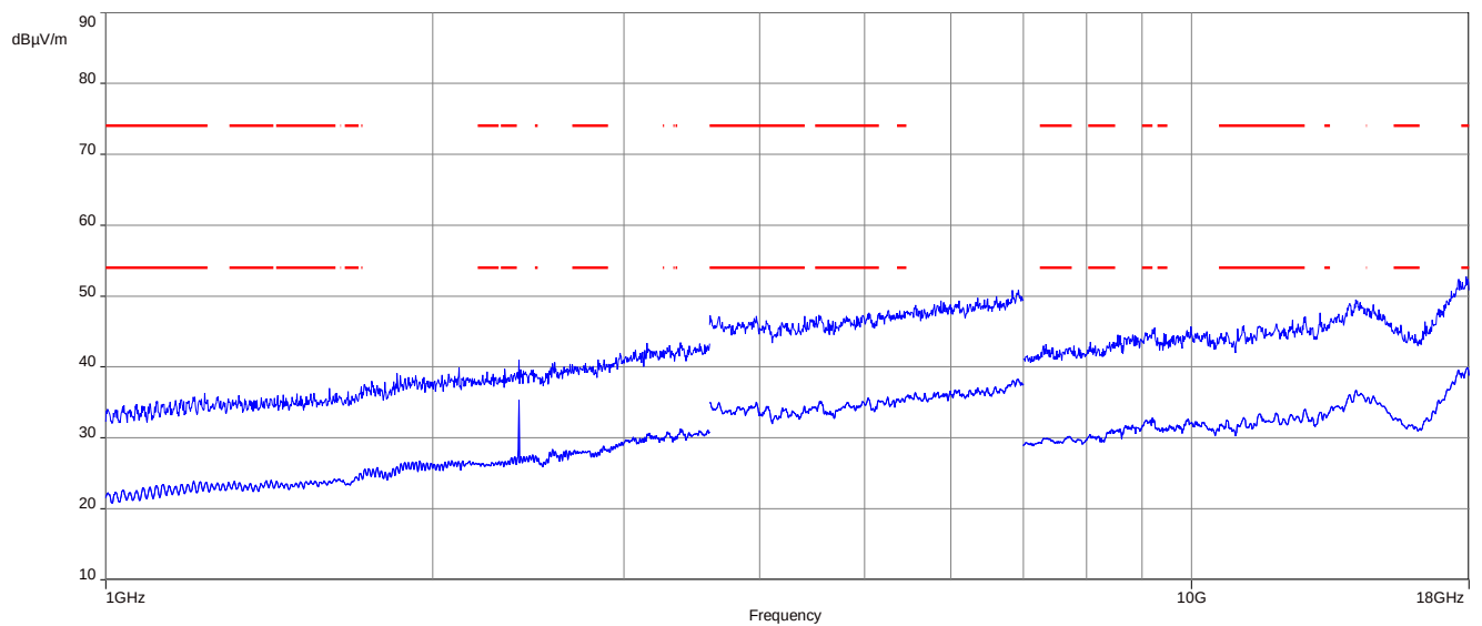
Plot 4: 1 GHz to 18 GHz, RX mode, 2402 MHz, vertical & horizontal polarization, 1 Msps
