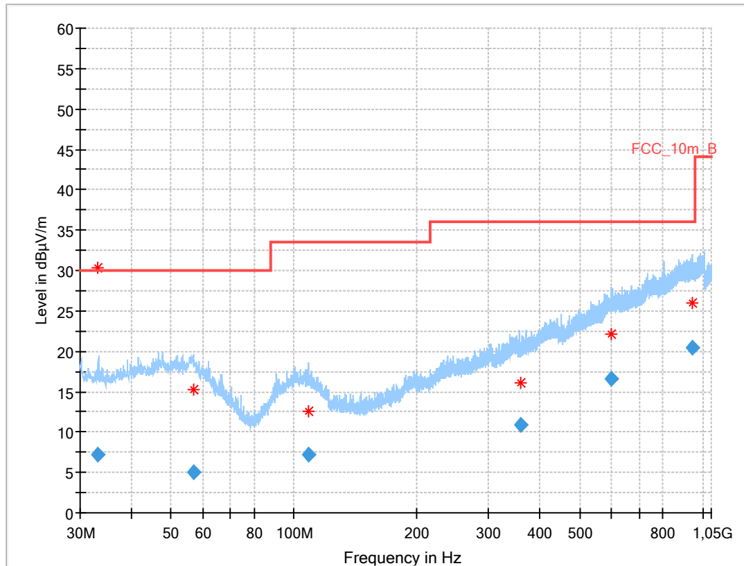
Plot 4: 30 MHz to 1 GHz, RX mode, 2402 MHz, vertical & horizontal polarization, 1 Msps
