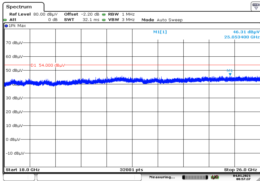
Plot 5: 18 GHz to 26 GHz, valid for all channels and modes, vertical & horizontal polarization, 1 Msps
