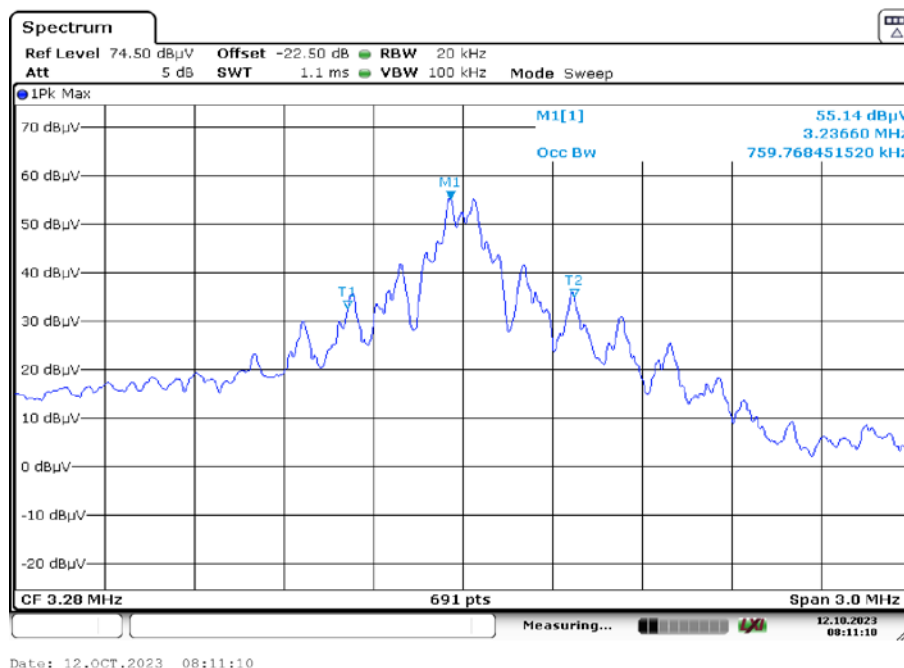
Plot 2: 99 % emission bandwidth MI e2e 5 ms
