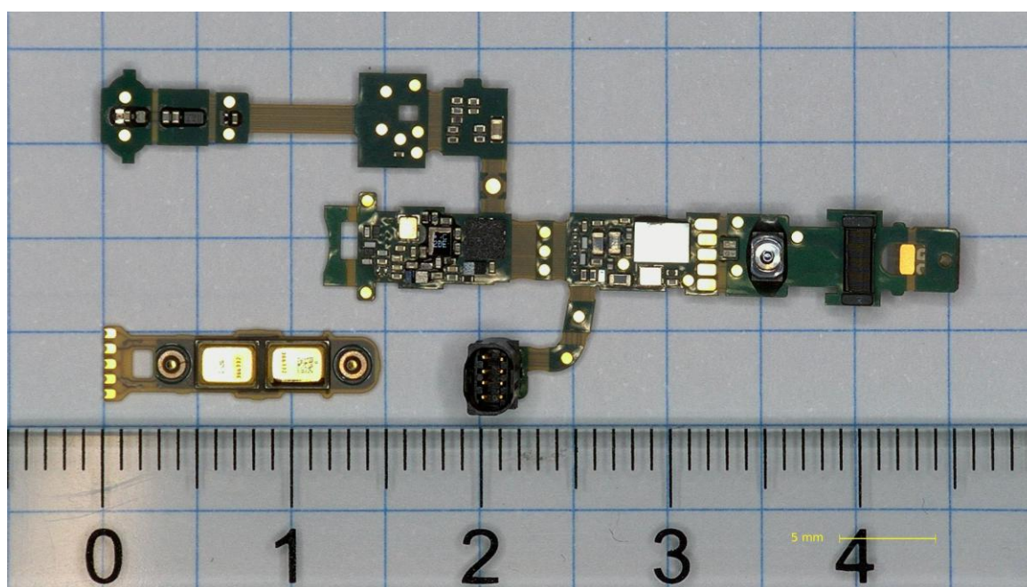
FPC print - top
