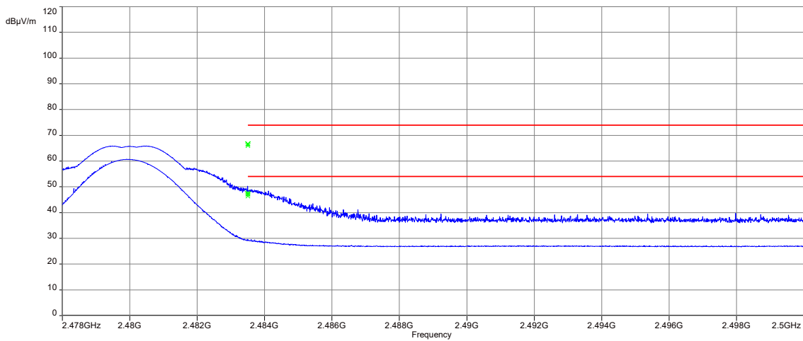
Plot 4: Upper restricted band, 2 Msps
