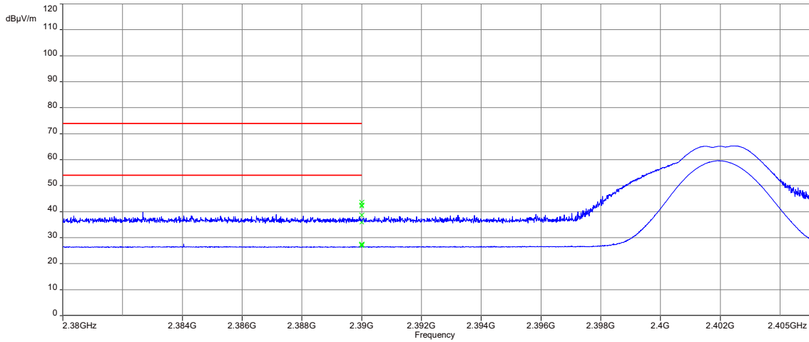
Plot 3: Lower restricted band, 2 Msps
