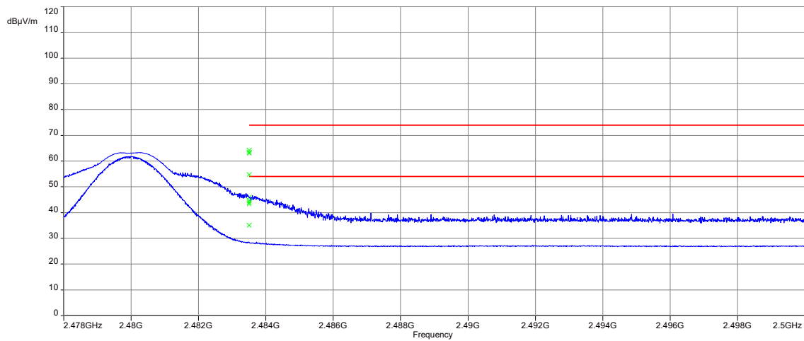
Plot 2: Upper restricted band, 1 Msps
