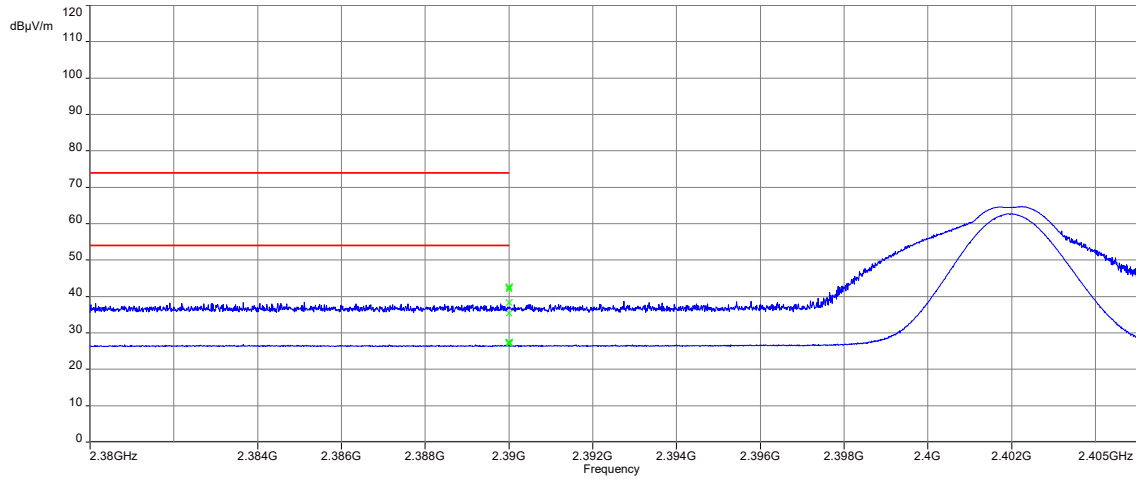
Plot 1: Lower restricted band, 1 Msps
