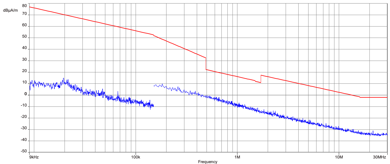
Plot 2: 9 kHz – 30 MHz, magnetic spurious emissions, 212 kBit/s ISED
