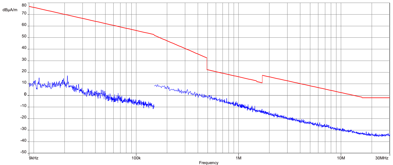
Plot 4: 9 kHz – 30 MHz, magnetic spurious emissions, 424 kBit/s ISED
