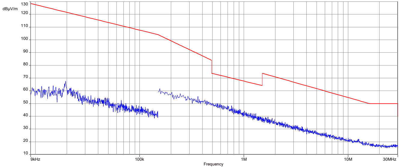
Plot 3: 9 kHz – 30 MHz, magnetic spurious emissions, 424 kBit/s FCC
