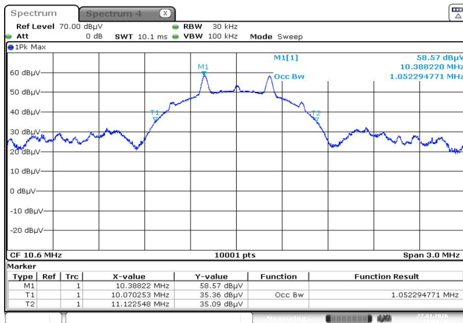
Plot 2: 99 % emission bandwidth 424 kBit/s
