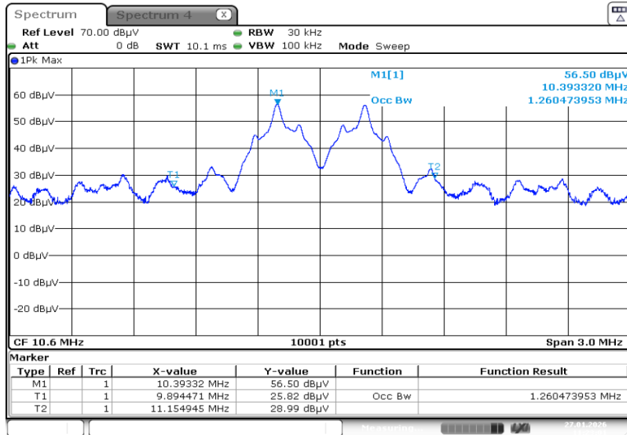
Plot 1: 99 % emission bandwidth 212 kBit/s
