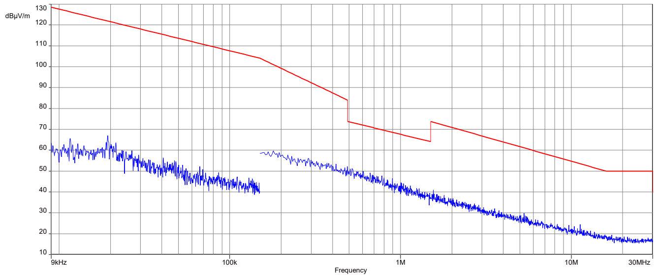
Plot 1: 9 kHz – 30 MHz, magnetic spurious emissions, 212 kBit/s FCC
