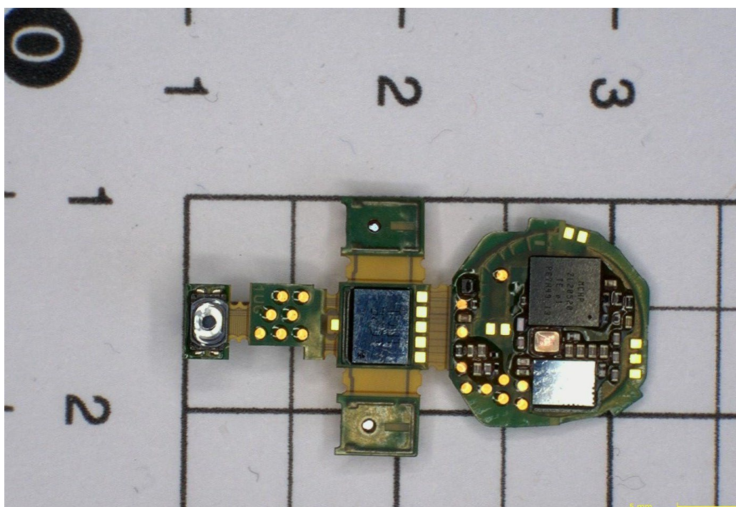
FPC print - top
