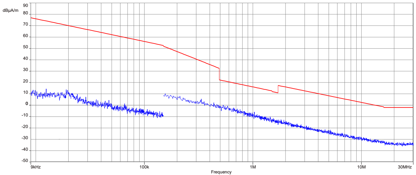
Plot 2: 212 kBit/s, 9 kHz – 30 MHz, magnetic spurious emissions IC
