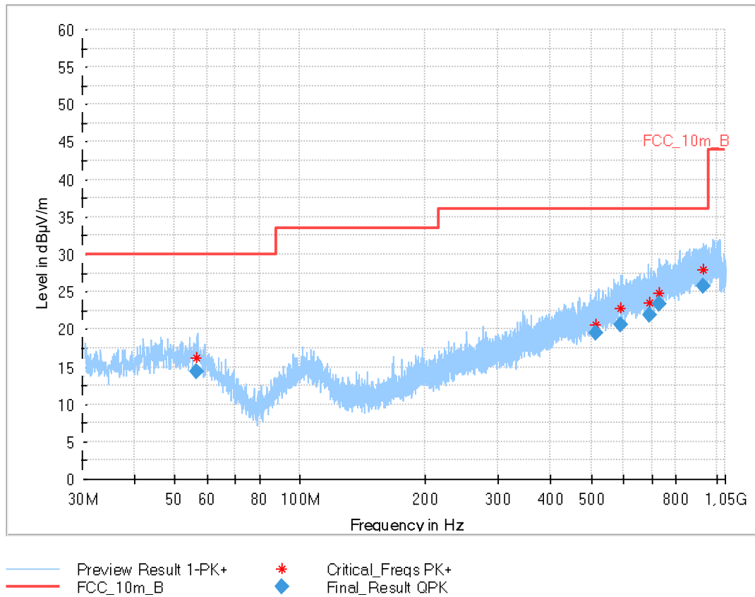
Plot 6: 424 kBit/s, 30 MHz – 1 GHz, vertical and horizontal polarization
