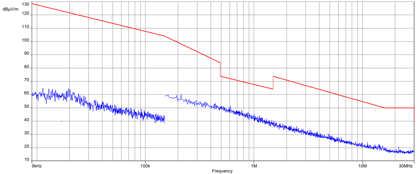
Plot 3: 424 kBit/s, 9 kHz – 30 MHz, magnetic spurious emissions FCC
