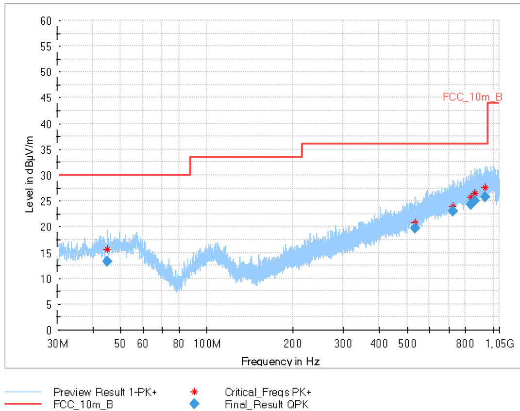
Plot 5: 212 kBit/s, 30 MHz – 1 GHz, vertical and horizontal polarization
