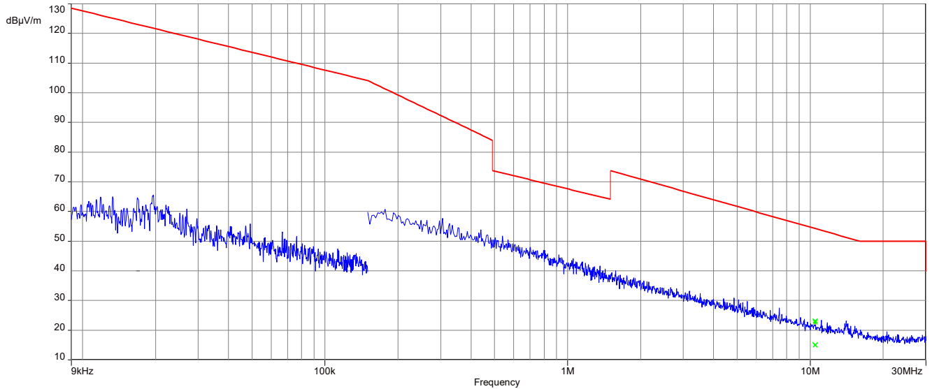
Plot 1: 212 kBit/s, 9 kHz – 30 MHz, magnetic spurious emissions FCC
