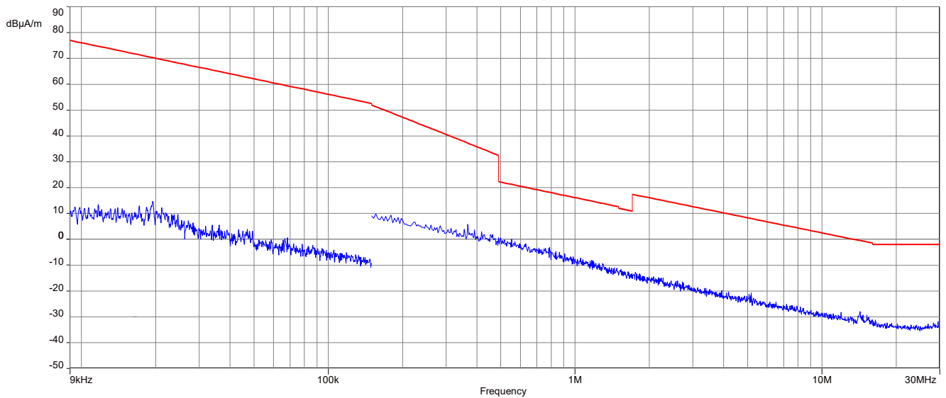
Plot 4: 424 kBit/s, 9 kHz – 30 MHz, magnetic spurious emissions IC
