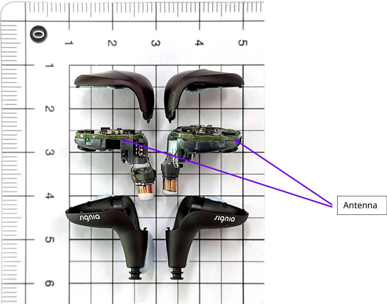
Hearing Aid with exploded enclosures:
