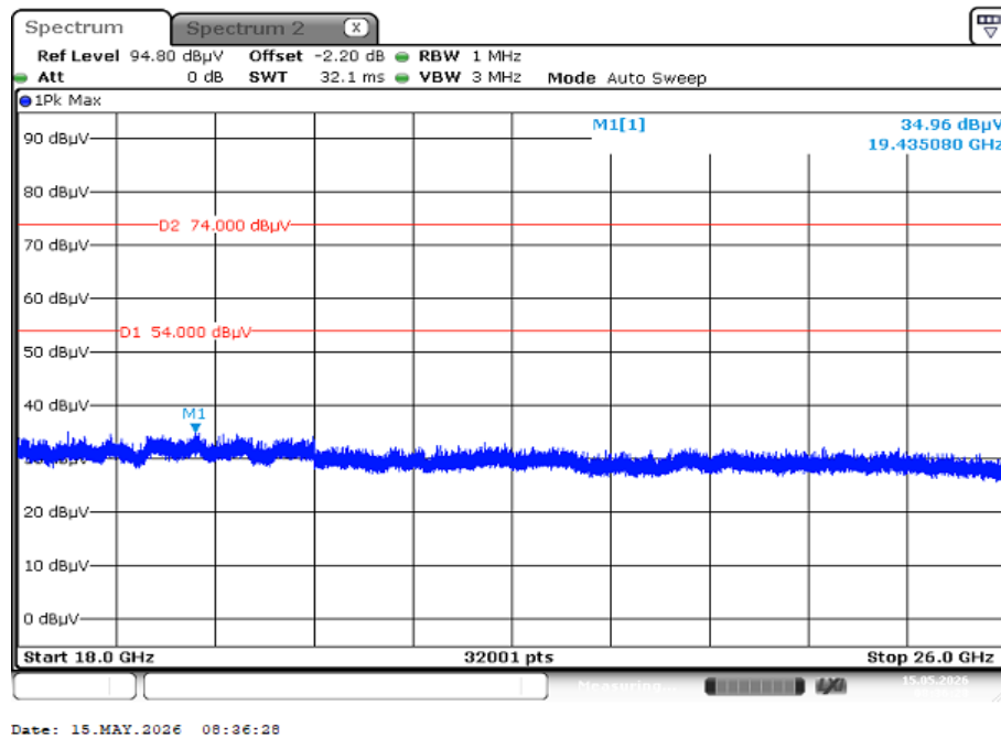
Plot 8: 18 GHz to 26 GHz, TX mode, vertical & horizontal polarization, valid for all channels of 2 Msps
