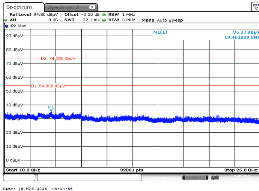
Plot 4: 18 GHz to 26 GHz, TX mode, vertical & horizontal polarization, valid for all channels of 1 Msps
