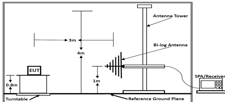
Below 1GHz
