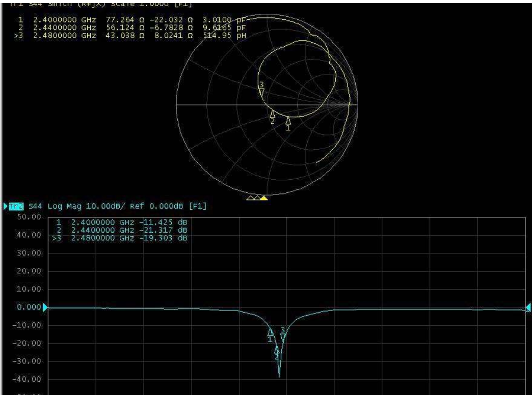
Return Loss
