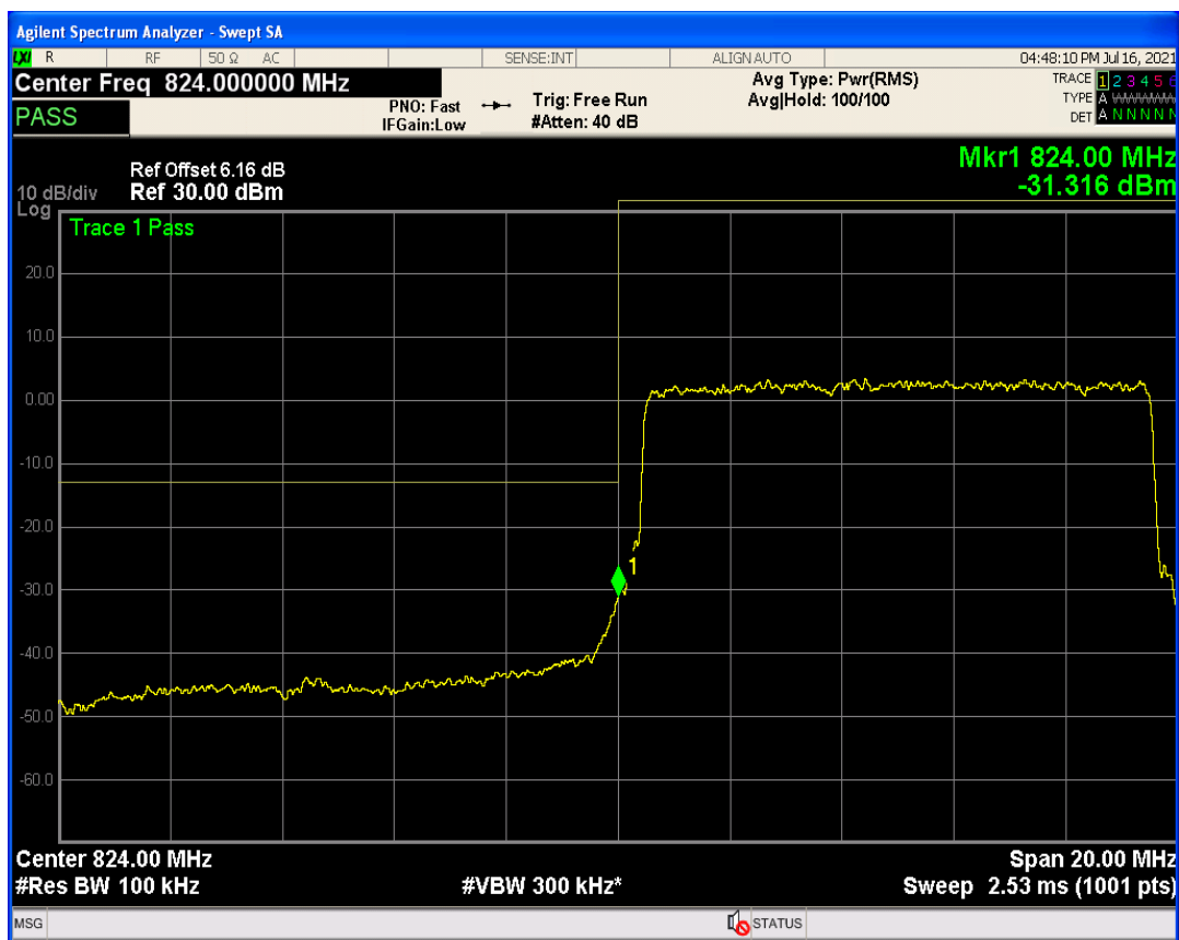
Band26b QAM16 BW=10MHz Channel=26840 RB Size=1 Position=#Max
