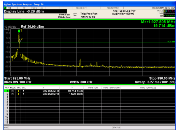
Band Edge-High Channel
