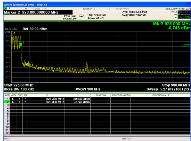
Band Edge-High Channel (Hopping Mode)
