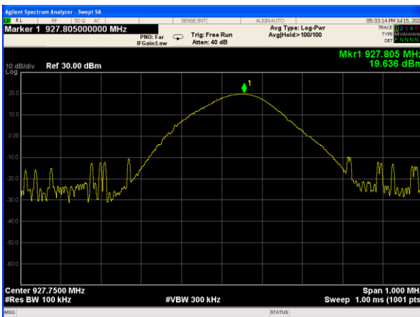
Peak output Power plot on channel 51
