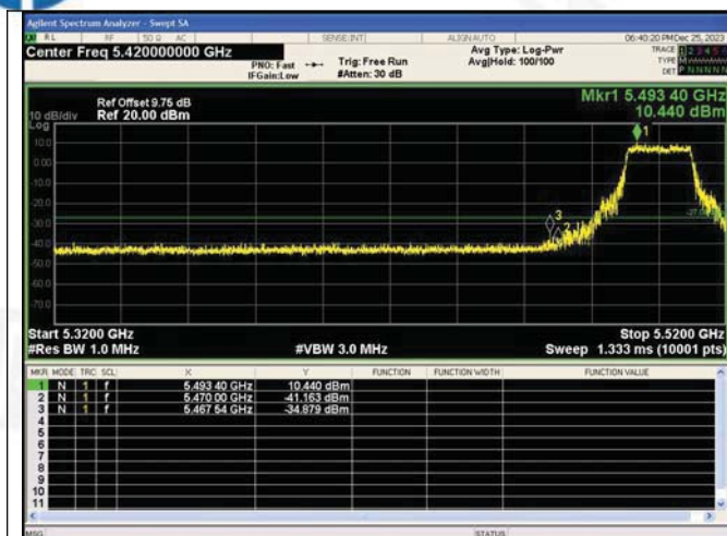
802.11ax(VH40)-5510
