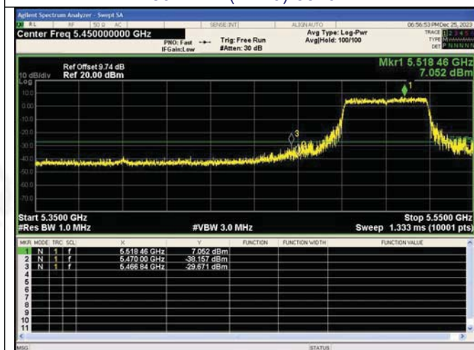
802.11n(HT20)-5500
